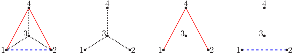
Fig. 3. A maximal Gallai coloring and its bipartitions.
