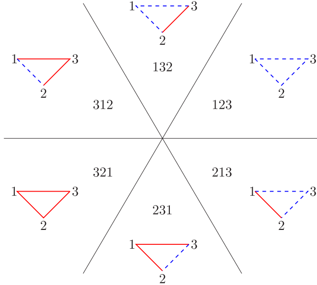
Fig. 6. The bijection from permutations in S_3 to 2-transitive colorings of \vec{K}_3 . Edges corresponding to inversions are drawn solid red.
