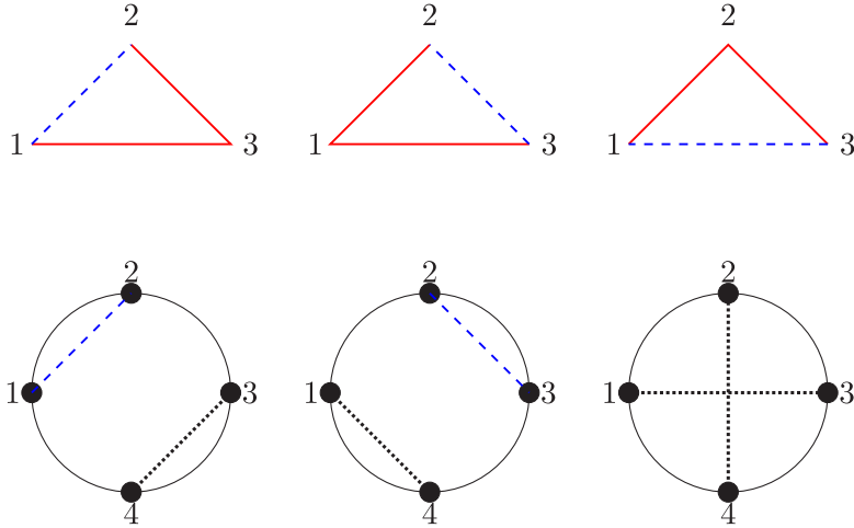
Fig. 2. The case n = 3 . The top row shows the three maximal Gallai partitions of K_3 . Each partition has two blocks, one of which is a singleton. The singleton edge is drawn dashed blue, and the two edges in the other block are drawn solid red. Note that the singleton edge (1, 3) does not have consecutive endpoint labels. The bottom row shows the three perfect matchings in M_4 . A chord in a matching is drawn dashed blue if its endpoints have consecutive labels in the set \{1, 2, 3\} , namely, it is a short chord in the upper half-plane.
