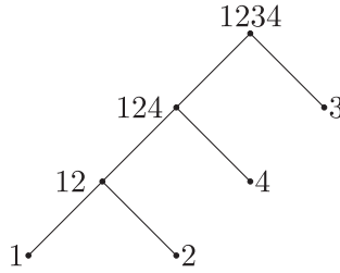
Fig. 4. The corresponding binary partition tree.
