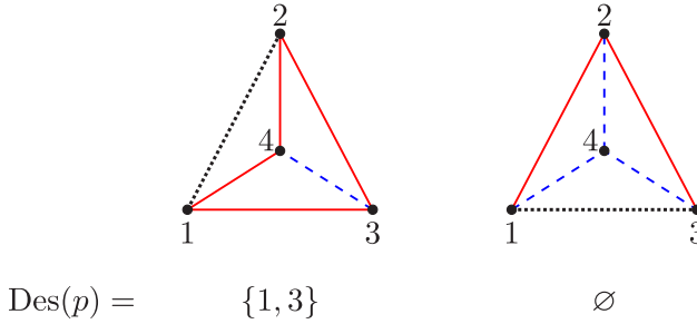
Fig. 1. Descent sets of Gallai partitions.
