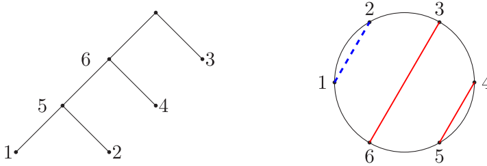
Fig. 5. A relabeled tree and the corresponding perfect matching. The short chord in the upper half-plane is colored dashed blue.
