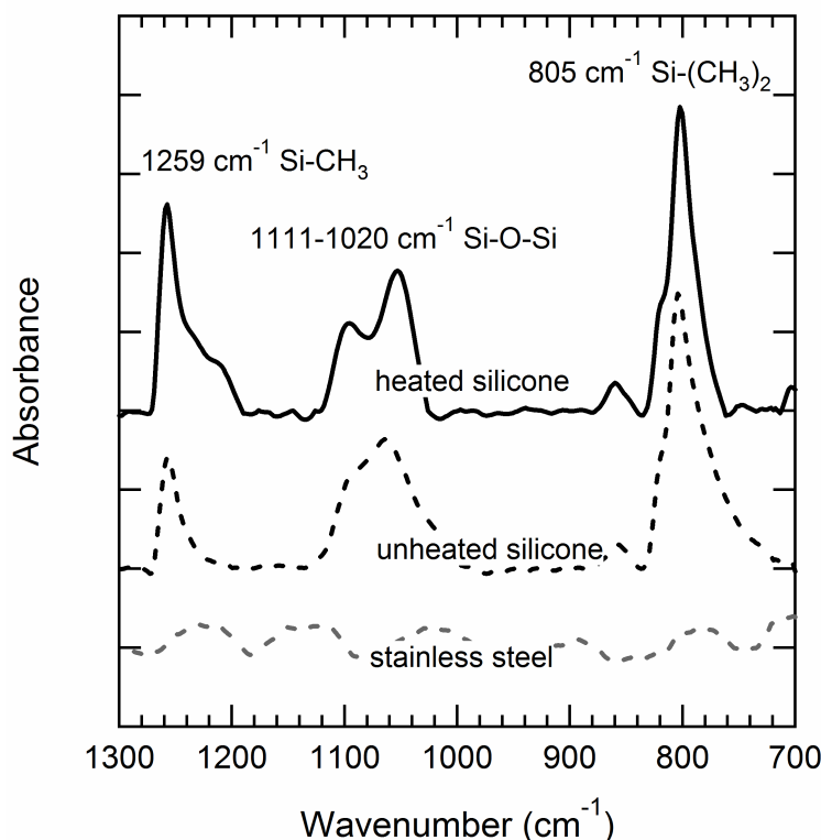
Figure 6. FTIR spectra of soot passed through equal lengths of stainless steel and silicone conductive tubing at room temperature (unheated), and heated silicone conductive tubing. Peaks in the spectra of the soot collected via silicone tubing correspond to siloxane functional groups and are not evident in the spectra of soot collected via stainless steel tubing. The distance between each tick mark on the vertical axis is 0.01 absorbance units.
