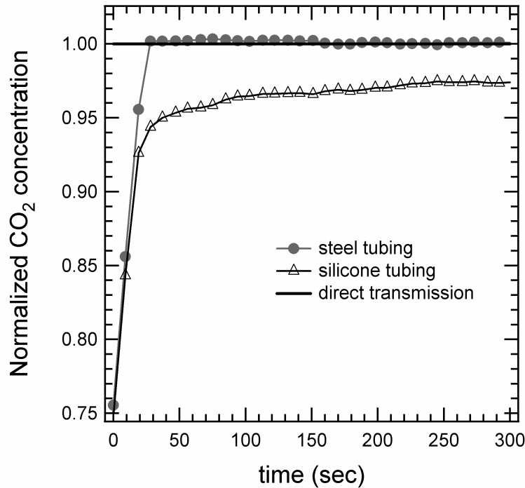
Figure 2. CO 2 concentrations in air dilution gas (initially 50,000 ppm CO 2 ) directly from the flow manifold and after transport through 15.2 m of stainless steel or 15.2 m of conductive silicone tubing. The CO 2 concentration is about 5% lower after transport through silicone tubing as compared to its concentration direct from the manifold or after transport through stainless steel tubing. The CO 2 concentration after transmission through silicone tubing appears to slowly recover, but the dynamic response time is greater than 5 min.
