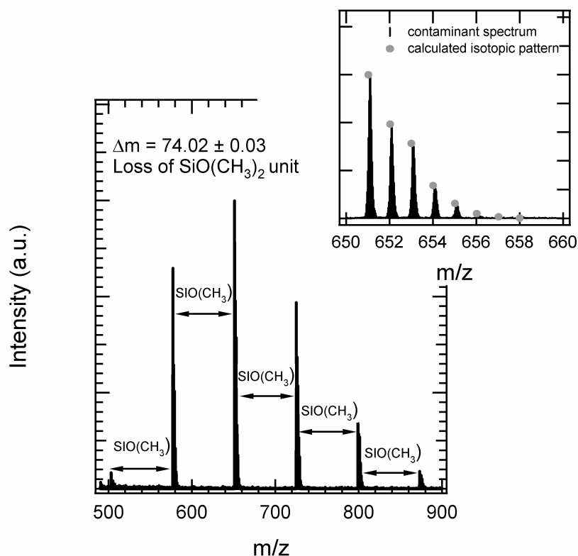
Figure 5. High resolution ( \Delta m/m \sim 3,000 ) mass spectrum for the PDMS contaminant obtained after soft-ionization using VUV radiation. Adjacent peaks are separated by 74.02 \pm 0.03 mass units, which corresponds to \text{SiO}(\text{CH}_3)_2 ( m/z 74.02). The inset compares the experimental spectrum to the predicted isotopic fragmentation pattern for (\text{SiO}(\text{CH}_3)_2)_8\text{SiOCH}_3^+ .
