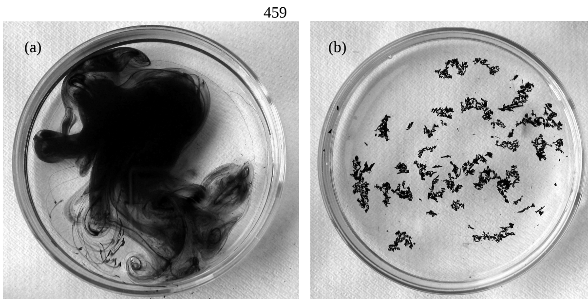
Figure 8. (a) Soot from a diffusion flame made hydrophilic by reaction with ozone. Shown is the soot as it is mixing with water. (b) Soot from a diffusion flame that does not mix with water despite ozone exposure. The soot in (b) was collected through silicone conductive tubing as opposed to the soot in (a), which was collected through stainless steel tubing.
