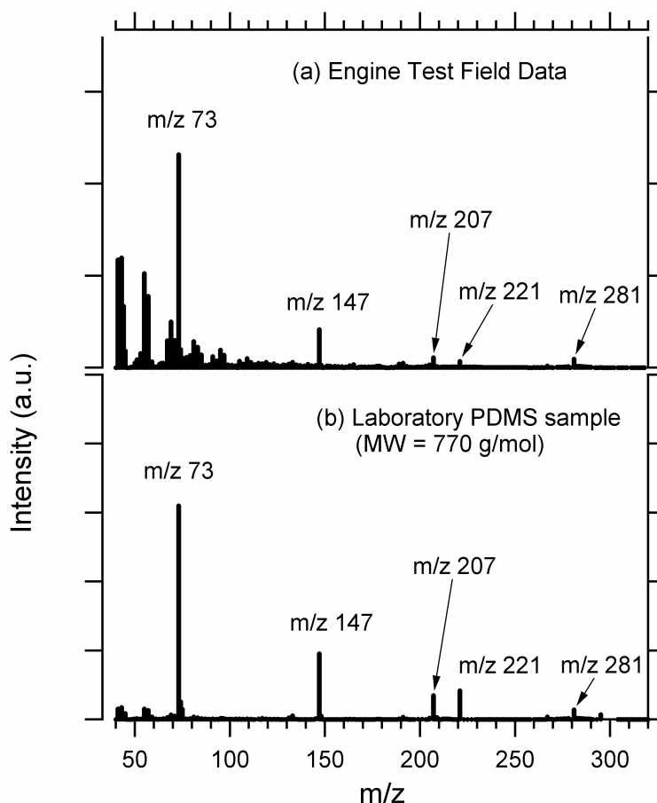
Figure 3. Characteristic EI ionization mass spectra obtained for a) engine exhaust particles and b) aerosolized polydimethylsiloxane (PDMS). The m/z features distinctive of PDMS, ( m/z = 73, 147, 207, 221, 281 ) are readily apparent as a contaminant in the engine exhaust particles.
