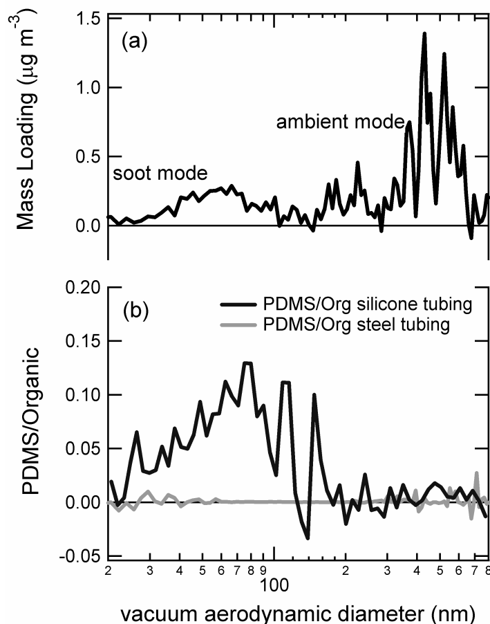
Figure 4. Particle size distribution of organic material and polydimethylsiloxane (PDMS) coated on soot particles generated by combustion of kerosene in a diffusion flame: a) total mass loading of organic particles obtained using either silicone (shown) or stainless steel tubing, b) ratio of PDMS to total organic obtained for using either silicone or stainless steel tubing. Data were collected for an hour by an aerosol mass spectrometer. When the silicone tubing is used, the mass loading of PDMS is about 10% of the total organic material in the 30-100 size range and roughly 2% in the 400-800 nm range. The size distribution of PDMS and organic material indicates well-mixed particle population for both soot sized particles (30-100 nm) and accumulation mode particles (400-800 nm).
