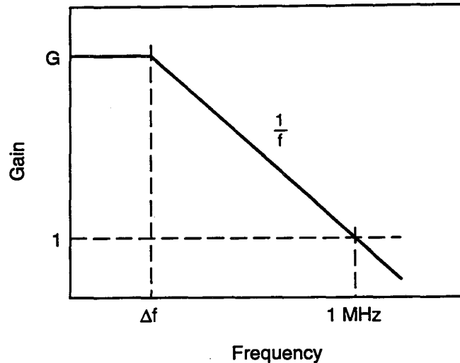
Figure 3-2. Typical Bode plot for the RF feedback circuit, illustrating the 1/f roll-off of the gain. The gain must decrease to unity at f \cong 1 MHz to ensure the stability of the feedback loop. [XBL 921-5517]
