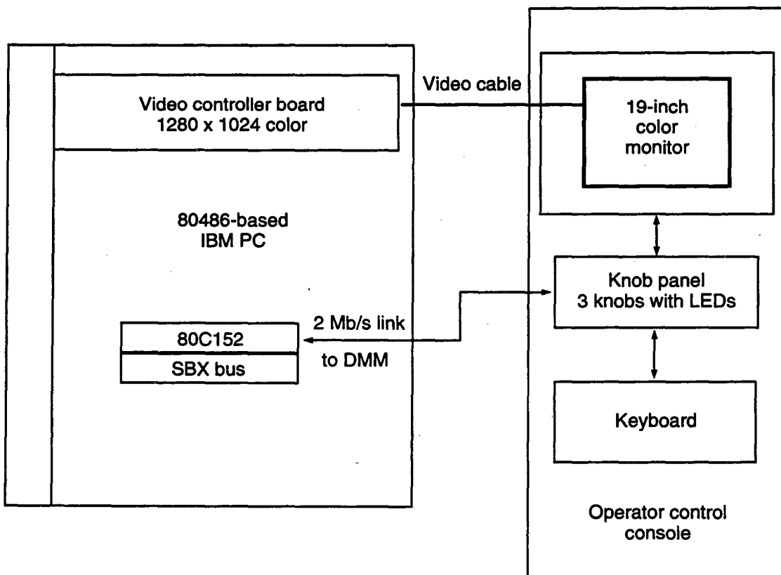
Figure 5-5. Block diagram of an operator control station. [XBL 902-5418]
