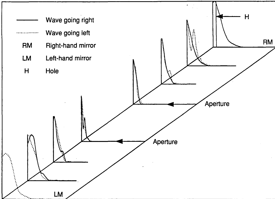
Figure 4-14. Intracavity intensity profiles of the dominant mode at a wavelength of 3 \mu\text{m} , for a gain of 55%. [XBL 922-5601]
