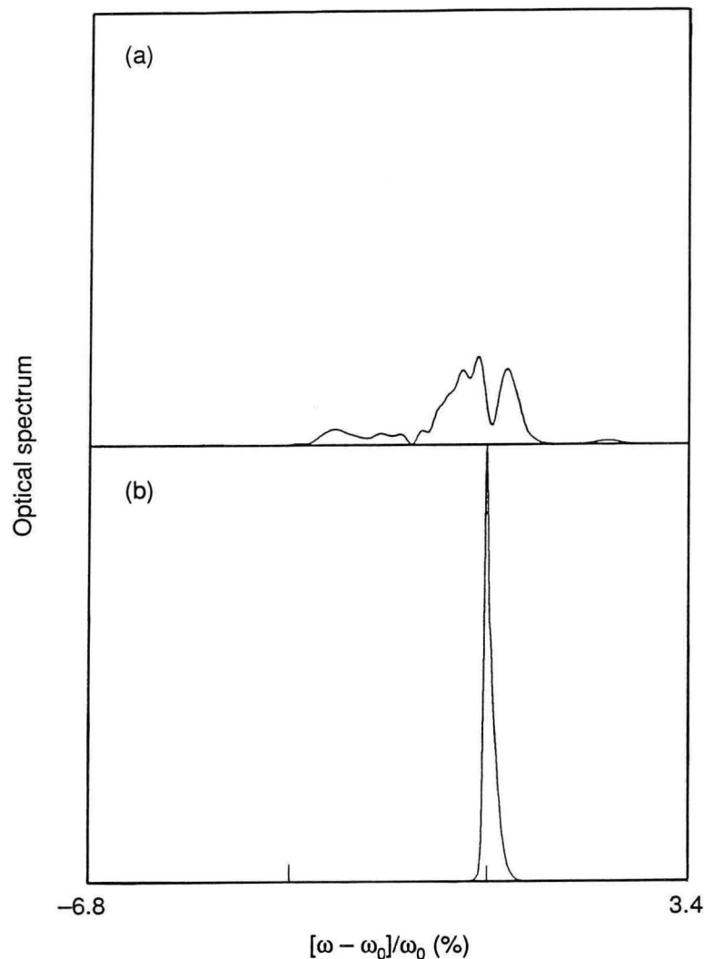
Figure 4-2. The FEL spectra for different cavity detunings, as a function of the relative frequency, for \lambda = 10 \mu\text{m} , \tau = 33 \text{ ps} , and pulse charge = 1 nC: (a) \delta L = 18 \mu\text{m} , corresponding to point A in Fig. 4-1; (b) \delta L = 89 \mu\text{m} , corresponding to point B. [XBL 922-5577]
