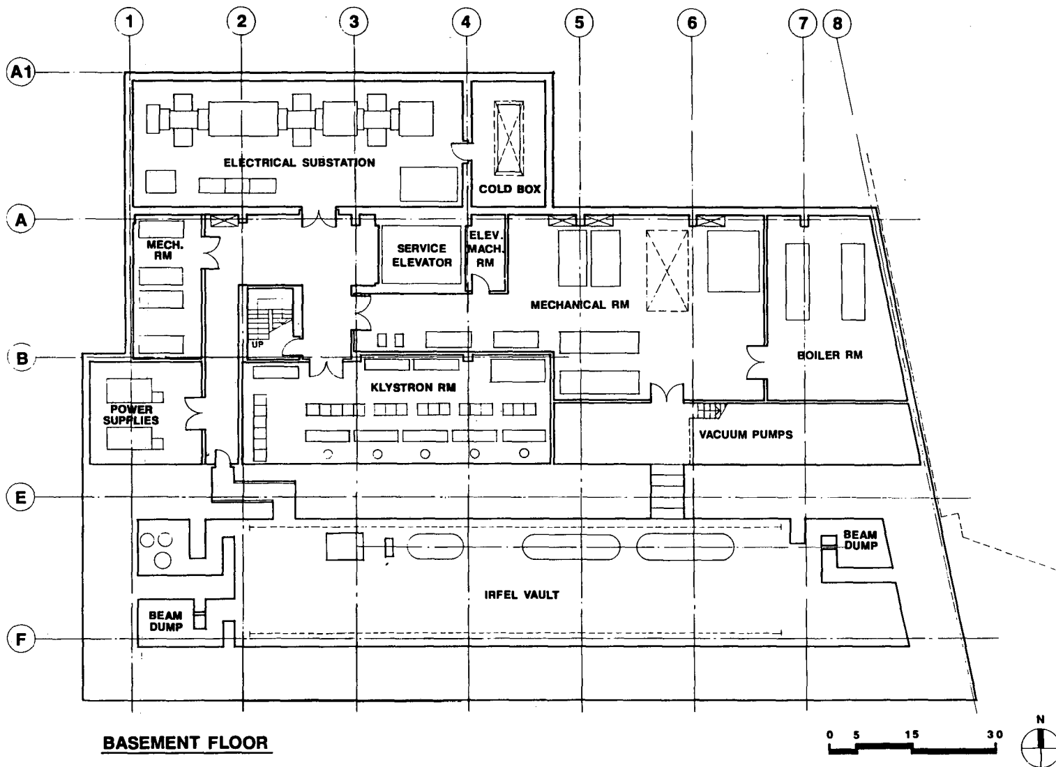
Figure 2-4. Plan view of the basement level of the proposed CDRL building.
