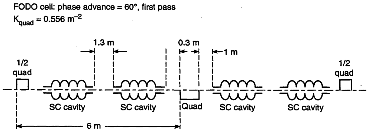
Figure 3-18. Model of the SCRF cavity and magnet configuration, used for simulation of multipass beam breakup. [XBL 922-5569]
