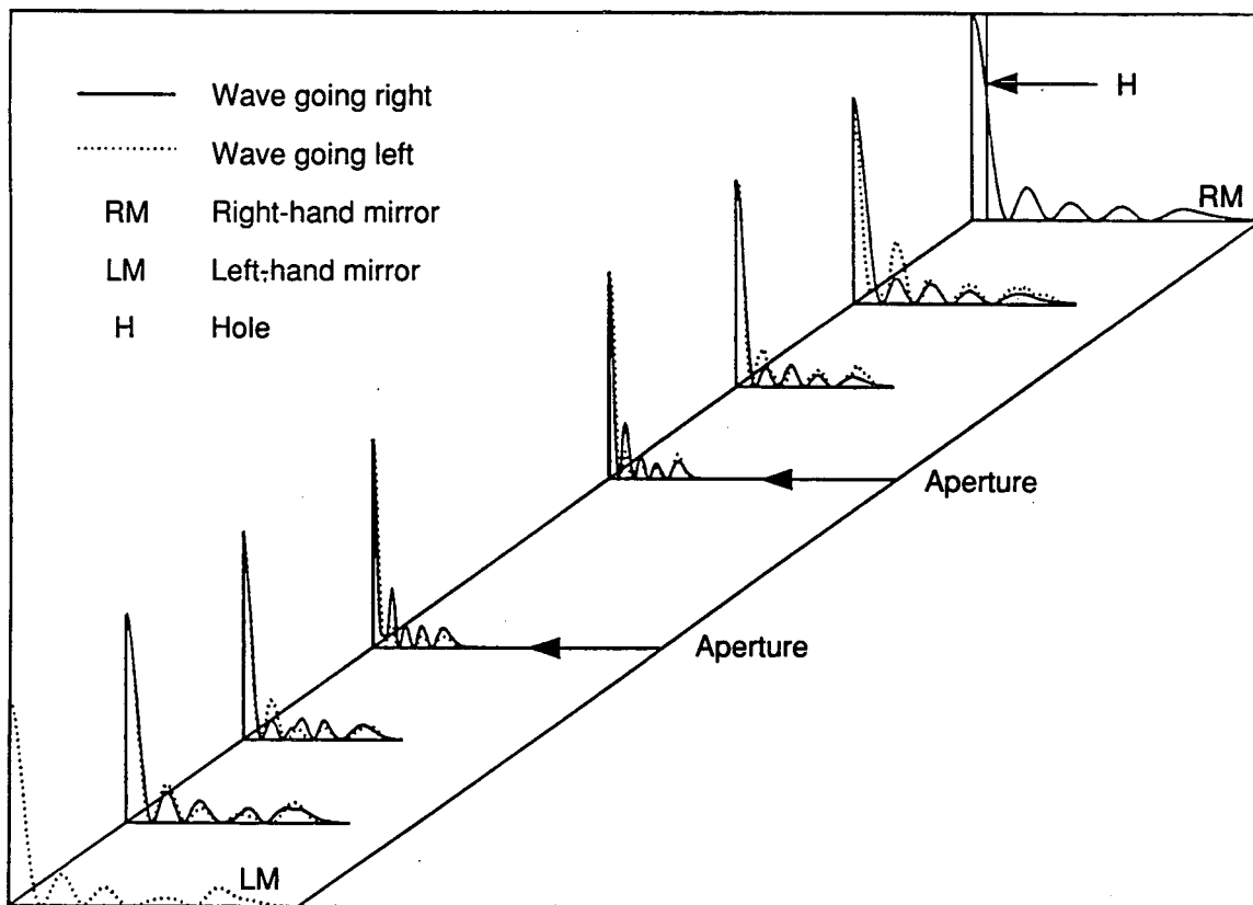
Figure 4-12. Intracavity intensity profiles of the dominant mode at a wavelength of 3 \mu\text{m} , for a gain of 0%. [XBL 922-5603]
