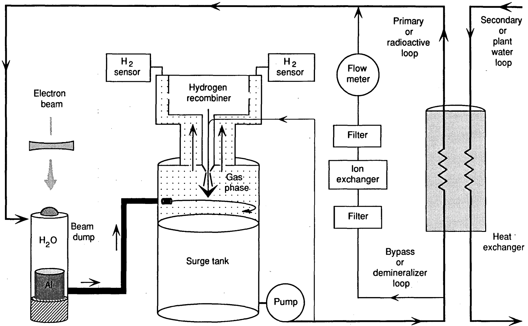
Figure 3-24. Schematic of the beam dump design for the IRFEL. [XBL 924-5658]
