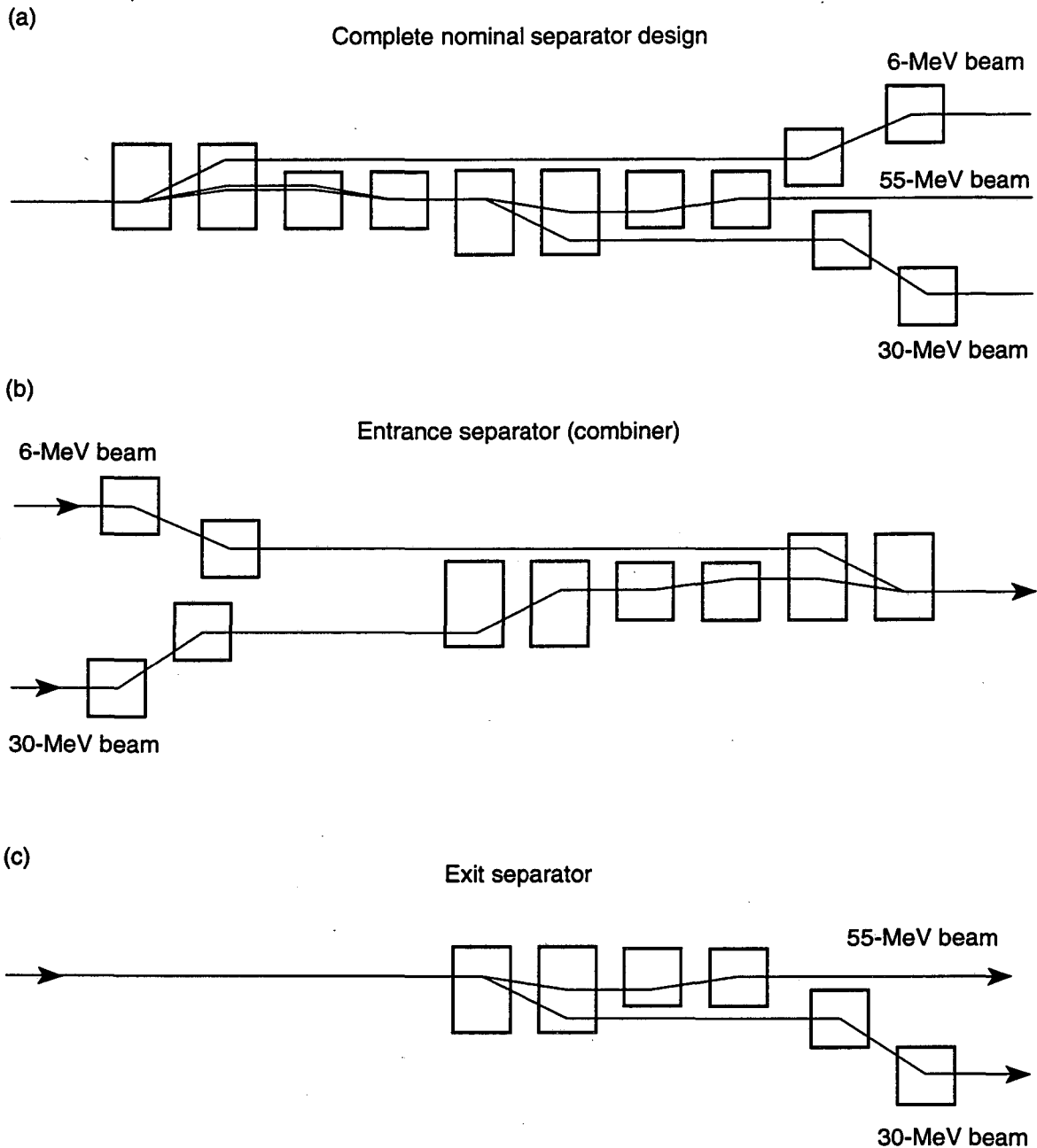
Figure 3-17. Schematics of three separator configurations: (a) the nominal separator design, which provides for the separation of the 6-MeV injected beam, a medium-energy (typically, 30-MeV) beam, and a high-energy (typically, 55-MeV) beam; (b) the entrance “separator,” which combines the injected beam and the recirculated beam; and (c) the exit separator, which directs beam to the two arcs downstream of the accelerator section. [XBL 922-5568]
