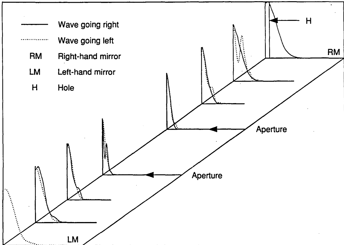
Figure 4-13. Intracavity intensity profiles of the dominant mode at a wavelength of 3 \mu\text{m} , for a gain of 2%. [XBL 922-5602]
