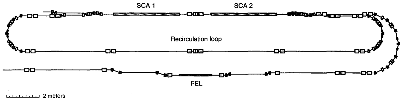
Figure 3-15. Plan view of the electron beam transport system, showing the location of the magnetic elements. The sizes of the magnets are not to scale. [XBL 922-5582]
