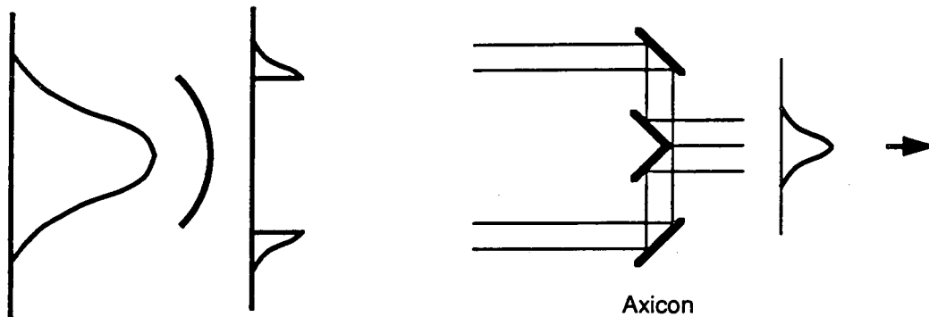
Figure 4-22. Schematic illustration of an axicon, used to improve the mode quality of an edge-coupled beam. [XBL 922-5596]
