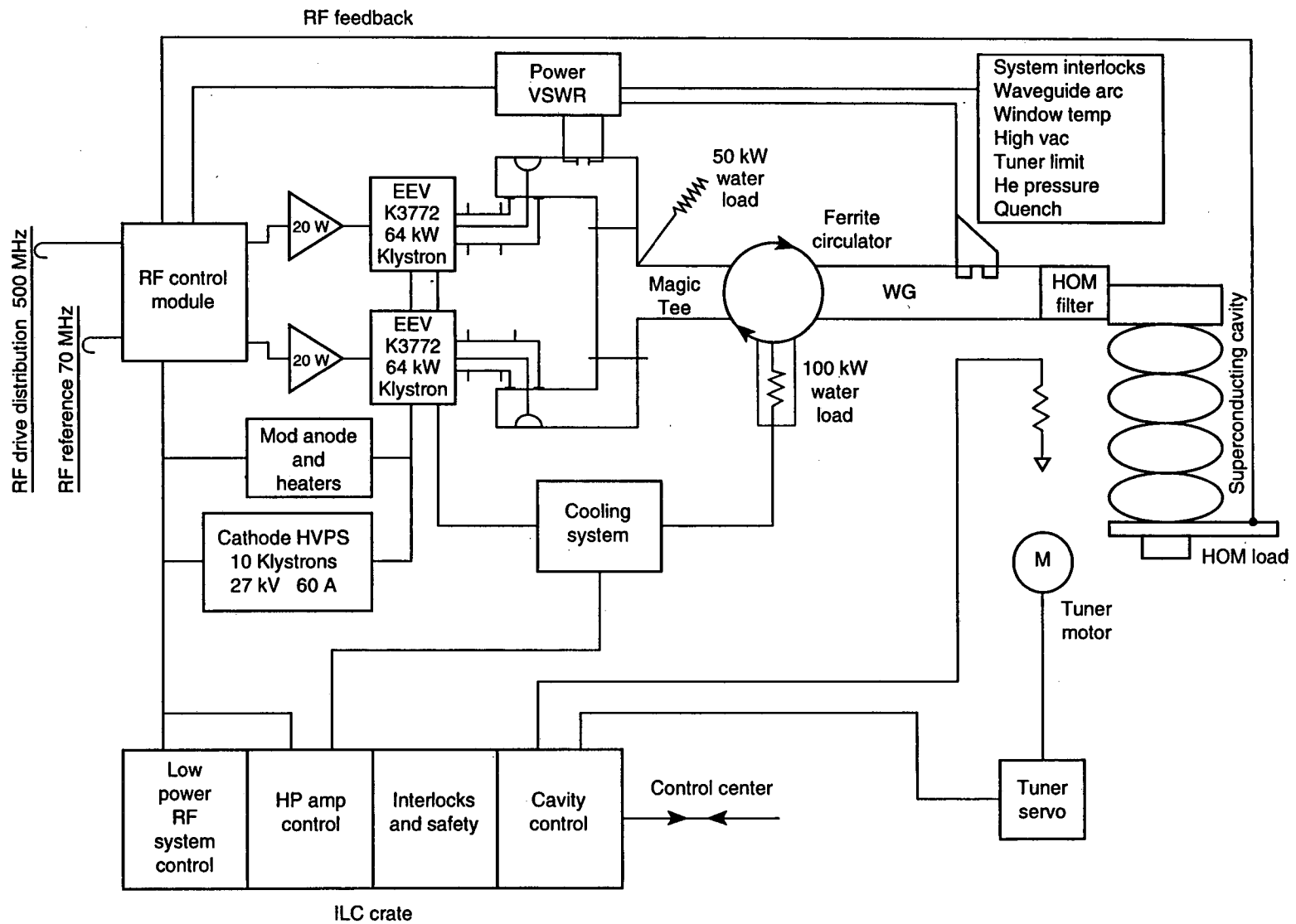
Figure 3-11. Schematic of the high-power RF system for the superconducting accelerator. [XBL 9111-6853]
