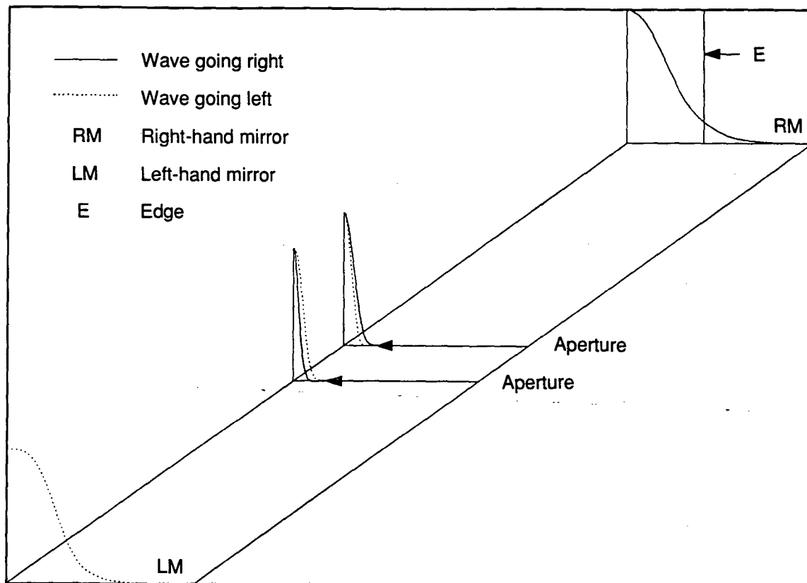
Figure 4-21. Intracavity mode profile at a wavelength of 21.5 \mu\text{m} , for an edge-coupled resonator. [XBL 922-5593]
