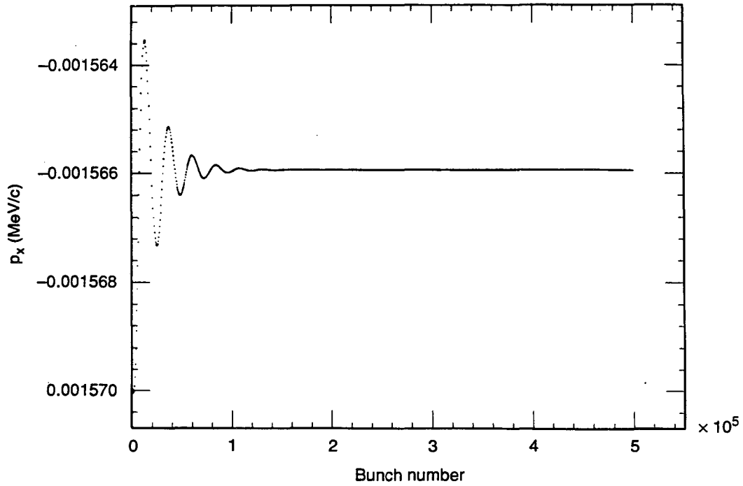
Figure 3-19. Bunch momentum as a function of bunch number for I = 90 mA. [XBL 922-5584]
