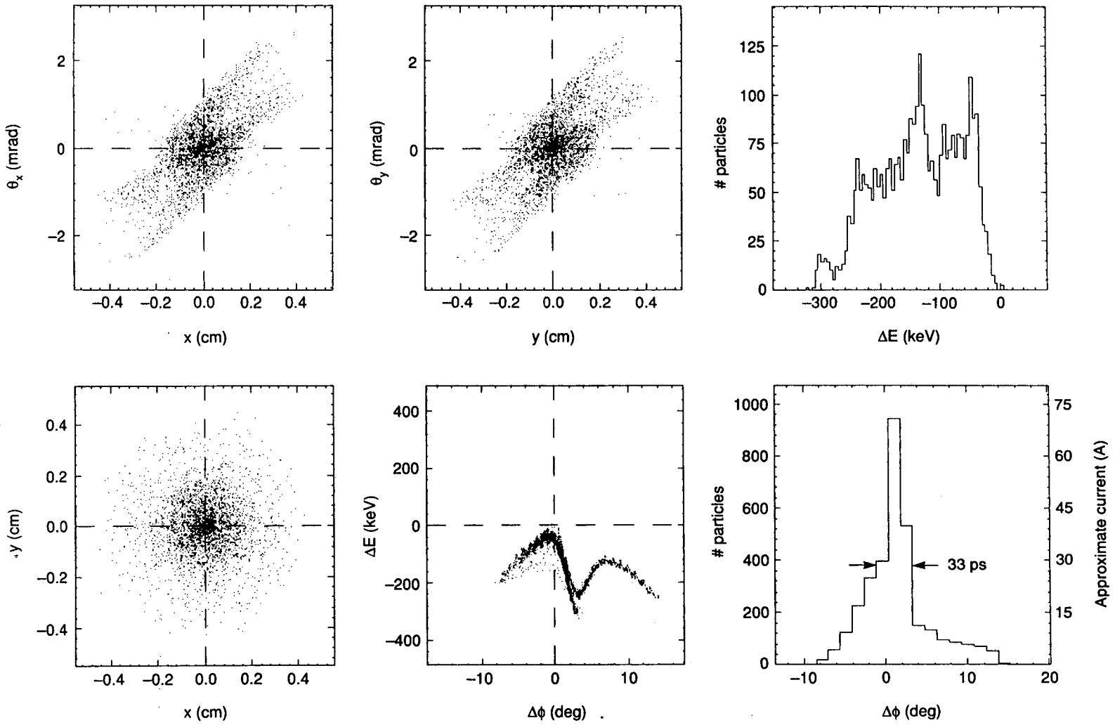
Figure 3-6b. Electron beam characteristics at the injector exit, downstream of the slit. See Fig. 3-6a for explanation. [XBL 922-5588]
