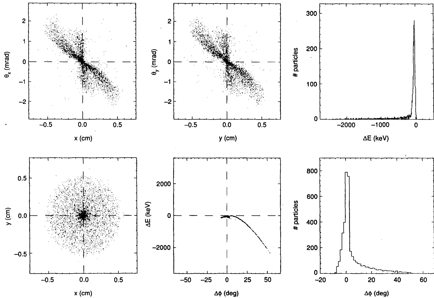
Figure 3-6a. Electron beam characteristics at the injector exit, upstream of the slit. The scatter plots at the upper left and upper center show the x and y phase space profiles, and the plot at the lower left shows the x-y beam profile. The plot at the lower center depicts the energy as a function of particle phase (z position). At the far right, histograms display the energy and phase distributions of the particles. [XBL 922-5587]
