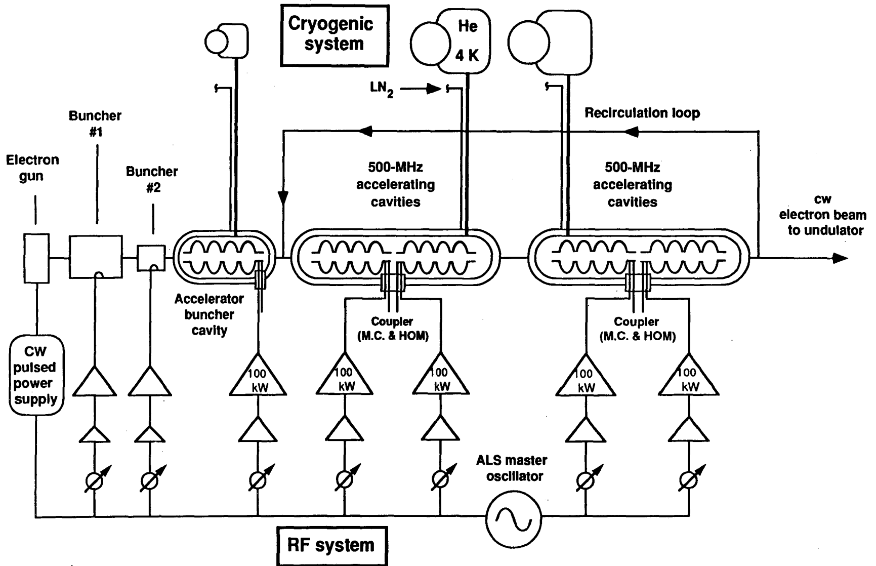
Figure 3-9. Schematic illustration of the RF accelerator system, together with the injector described in section 3.2. [XBL 922-5609]
