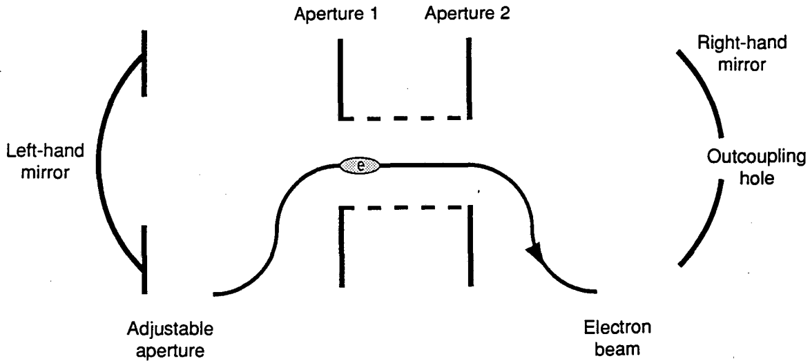
Figure 4-9. Cross-sectional view of a cylindrical IRFEL resonator, as modeled for the simulation code HOLD. The resonator consists of two mirrors and two intracavity apertures. A circular hole is located at the center of the right-hand mirror, and an adjustable aperture is placed in front of the left-hand mirror for mode control. The dashed lines indicate the boundary of an undulator bore simulated by the two fixed apertures. An electron beam traverses the FEL interaction region from aperture 1 to aperture 2. [XBL 922-5606]
