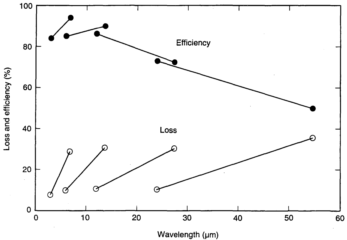
Figure 4-20. Edge-coupling performance parameters as functions of wavelength. [XBL 922-5594]
