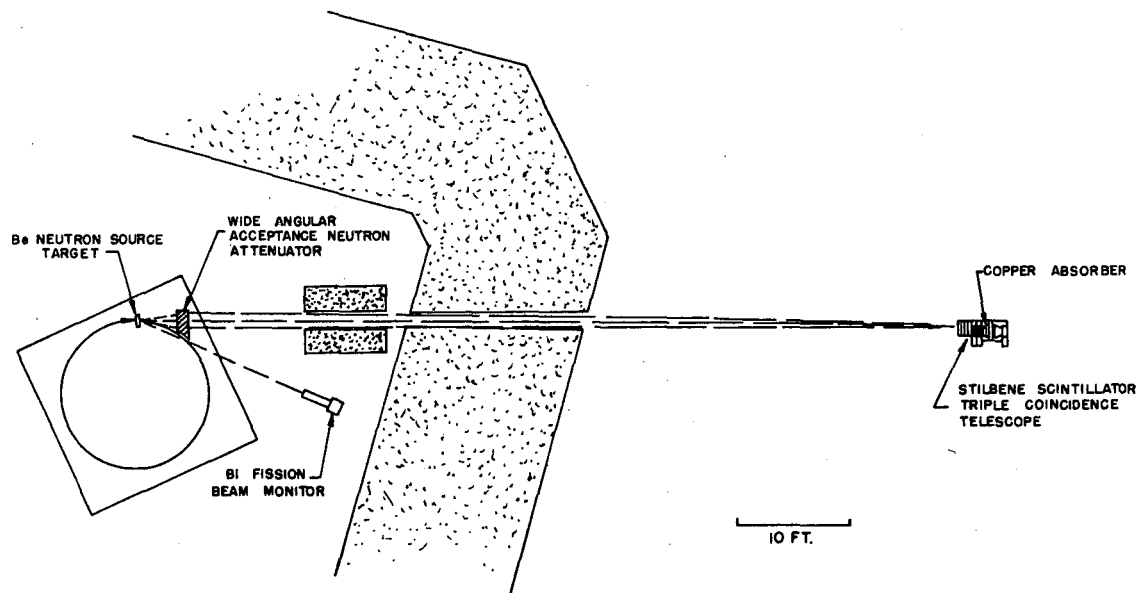
ATTENUATOR IN PROXIMITY OF SOURCE ARRANGEMENT
