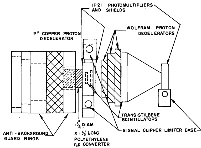
NEUTRON DETECTOR TELESCOPE (ELASTIC SCATTERING ARRANGEMENT)
