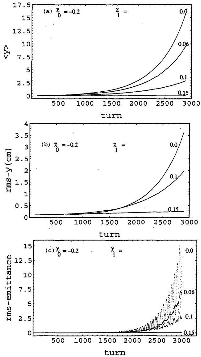
FIG. 7. Multi-particle simulation results showing stabilization of the HT motions of (a) the centroid, (b) the rms-size, and (c) the rms-emittance of a Gaussian beam by \chi_1 , when \chi_0 = -0.2 and \Upsilon = 0.22 . The estimated stability threshold for the l = 0 mode, according to Eq. (57), is \chi_1 \geq 0.22 . See Eqs. (8) and (9) for definitions of \chi_0 , \chi_1 , and \Upsilon .
