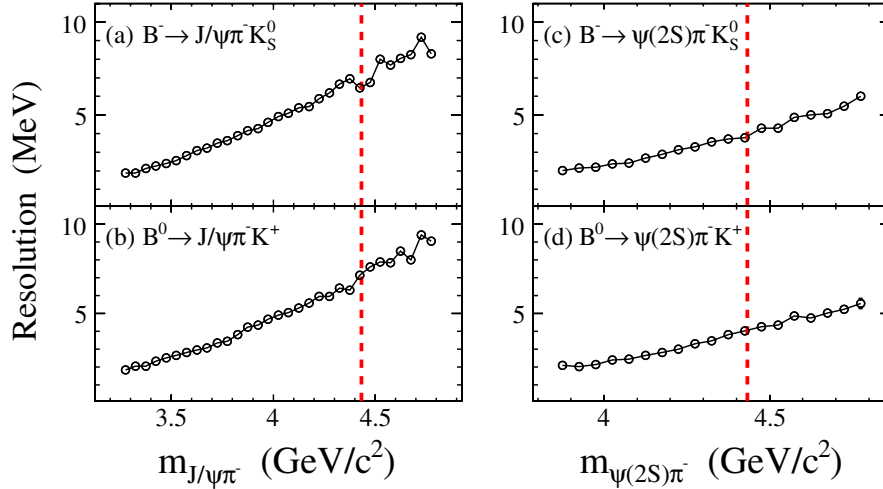
FIG. 6 (color online). The \psi\pi^- mass resolution in 50 \text{ MeV}/c^2 intervals as a function of \psi\pi^- mass for the decay modes (a) B^- \rightarrow J/\psi\pi^-K_S^0 , (b) B^0 \rightarrow J/\psi\pi^-K^+ , (c) B^- \rightarrow \psi(2S)\pi^-K_S^0 , and (d) B^0 \rightarrow \psi(2S)\pi^-K^+ . The dashed vertical lines indicate m_{\psi\pi^-} = 4.433 \text{ GeV}/c^2 .
