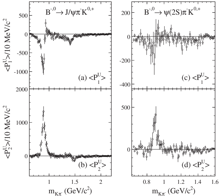
FIG. 14. The m_{K\pi^-} dependence of (a) \langle P_1^U \rangle and (b) \langle P_2^U \rangle for B^{0,-} \rightarrow J/\psi \pi^- K^{+,0} ; the m_{K\pi^-} dependence of (c) \langle P_1^U \rangle and (d) \langle P_2^U \rangle for B^{0,-} \rightarrow \psi(2S) \pi^- K^{+,0} .
