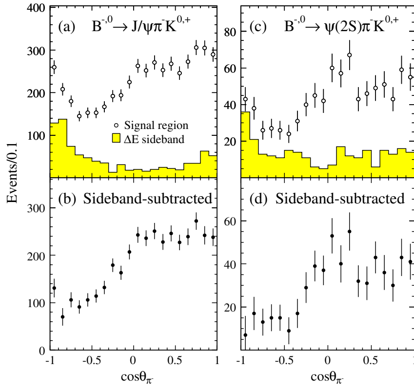
FIG. 31 (color online). The \cos\theta_\pi distributions for the combined K\pi^- mass regions A, C, and E, (a), (b) for the decay modes B^{-,0} \rightarrow J/\psi\pi^-K^{0,+} , and (c), (d) for B^{-,0} \rightarrow \psi(2S)\pi^-K^{0,+} . In (a) and (c), the points represent the data in the signal region, and the shaded histograms show the \Delta E sideband events. In (b) and (d), the signal region distributions are shown after sideband subtraction. No efficiency correction is applied to the data.
