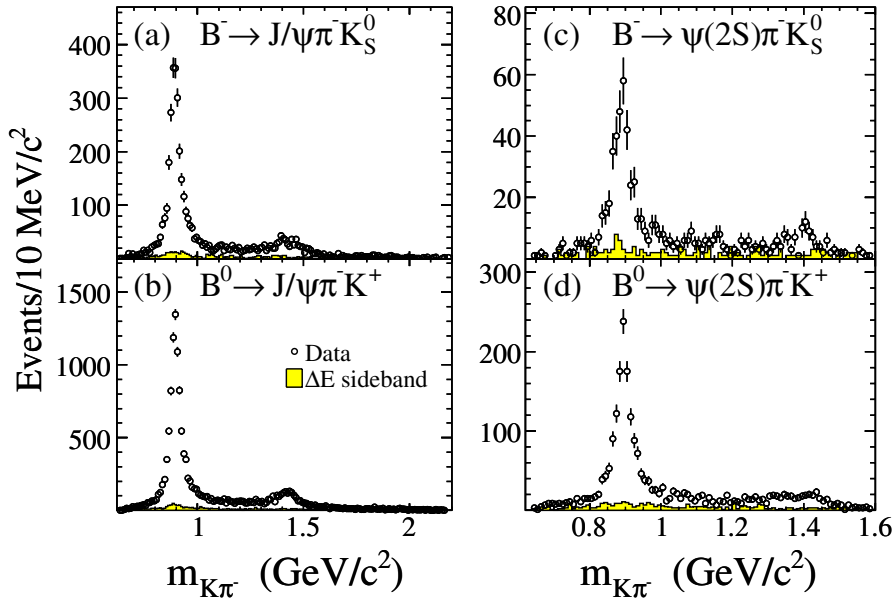
FIG. 3 (color online). The m_{K\pi} mass projections for the Dalitz plots of Fig. 2. The data points are for the m_{ES} - \Delta E signal regions, and the filled histograms are for the \Delta E sideband regions.
