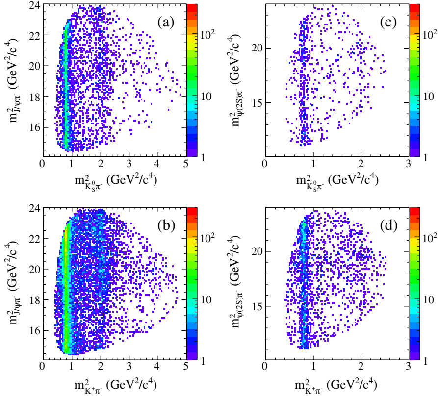
FIG. 2 (color online). The m_{\psi\pi}^2 versus m_{K\pi}^2 Dalitz plot distributions for the signal regions for the decay modes (a) B^- \rightarrow J/\psi \pi^- K_S^0 , (b) B^0 \rightarrow J/\psi \pi^- K^+ , (c) B^- \rightarrow \psi(2S) \pi^- K_S^0 , (d) B^0 \rightarrow \psi(2S) \pi^- K^+ . The intensity scale is logarithmic.
