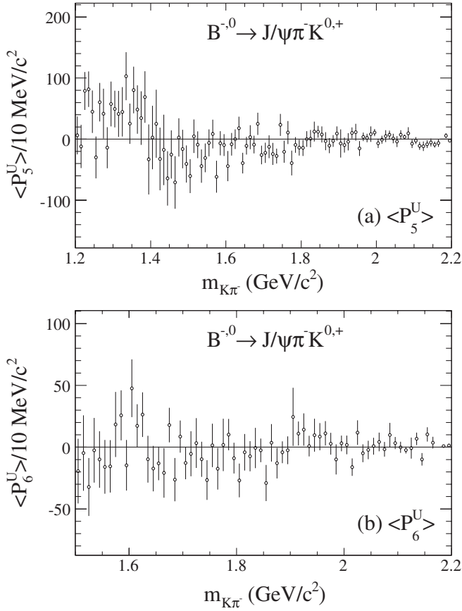
FIG. 16. (a) The m_{K\pi^-} dependence of \langle P_5^U \rangle for m_{K\pi^-} > 1.2 GeV/ c^2 for B^{0,-} \rightarrow J/\psi \pi^- K^{0,+} ; (b) the m_{K\pi^-} dependence of \langle P_6^U \rangle for m_{K\pi^-} > 1.5 GeV/ c^2 for B^{0,-} \rightarrow J/\psi \pi^- K^{0,+} .
