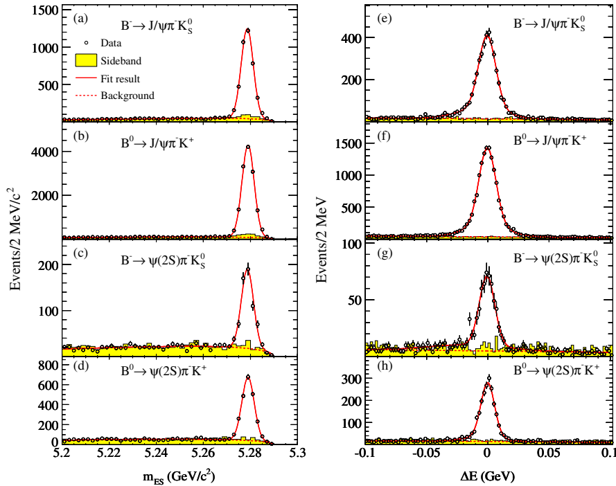
FIG. 1 (color online). The m_{ES} distributions, (a)–(d), and \Delta E distributions, (e)–(h), for the decay modes B^- \rightarrow J/\psi\pi^- K_S^0 , B^0 \rightarrow J/\psi\pi^- K^+ , B^- \rightarrow \psi(2S)\pi^- K_S^0 , and B^0 \rightarrow \psi(2S)\pi^- K^+ . The points show the data, and the solid curves represent the fit functions. The dashed curves indicate the background contributions, and the filled histograms show the corresponding distributions for the sideband regions.
