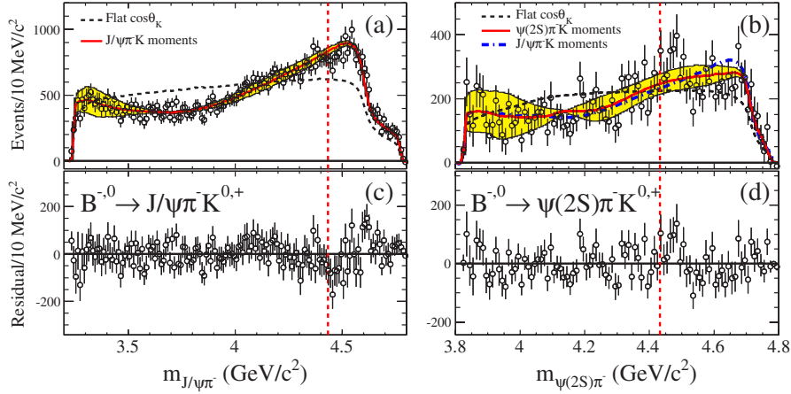
FIG. 21 (color online). The \psi\pi^- mass distributions for the combined decay modes (a) B^{-,0} \rightarrow J/\psi\pi^- K^{0,+} and (b) B^{-,0} \rightarrow \psi(2S)\pi^- K^{0,+} . The points show the data after efficiency correction and \Delta E sideband subtraction. The dashed curves show the K\pi^- reflection for a flat \cos\theta_K distribution, while the solid curves show the result of \cos\theta_K weighting. The shaded bands represent the effect of statistical uncertainty on the normalized moments. In (b), the dot-dashed curve indicates the effect of weighting with the normalized J/\psi\pi^- K moments. The dashed vertical lines indicate m_{\psi\pi^-} = 4.433 GeV/c 2 . In (c) and (d), we show the residuals (data—solid curve) for (a) and (b), respectively.
