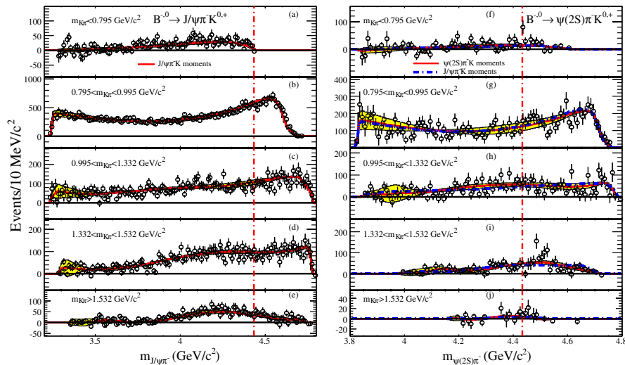
FIG. 25 (color online). The \psi\pi^- mass distributions in regions A–E of K\pi^- mass for the combined decay modes [(a)–(e)] B^{-,0} \rightarrow J/\psi\pi^-K^{0,+} , and [(f)–(j)] B^{-,0} \rightarrow \psi(2S)\pi^-K^{0,+} ; the open dots represent the data, and the solid curves and shaded bands are as in Fig. 21, but calculated for the relevant K\pi^- mass region using the same overall normalization constant as for Fig. 17. In (f)–(j), the dot-dashed curves are obtained using K\pi^- normalized moments for B^{-,0} \rightarrow J/\psi\pi^-K^{0,+} in Eq. (35), instead of those from B^{-,0} \rightarrow \psi(2S)\pi^-K^{0,+} ; the dot-dashed vertical lines indicate m_{\psi\pi^-} = 4.433 \text{ GeV}/c^2 .
