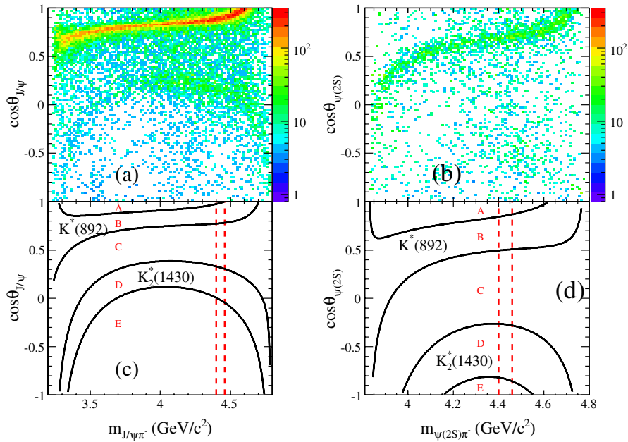
FIG. 22 (color online). The \cos\theta_\psi versus m_{\psi\pi^-} rectangular Dalitz plots for (a) B^{-,0} \rightarrow J/\psi\pi^- K^{0,+} , and (b) B^{-,0} \rightarrow \psi(2S)\pi^- K^{0,+} ; (c) and (d), the corresponding plots indicating the loci of the K^*(892) and K_2^*(1430) resonance bands defined in the text; regions A–E, defined by Eqs. (36)–(40), are indicated. The dashed vertical lines show the mass range 4.400 < m_{\psi\pi^-} < 4.460 GeV/c 2 .
