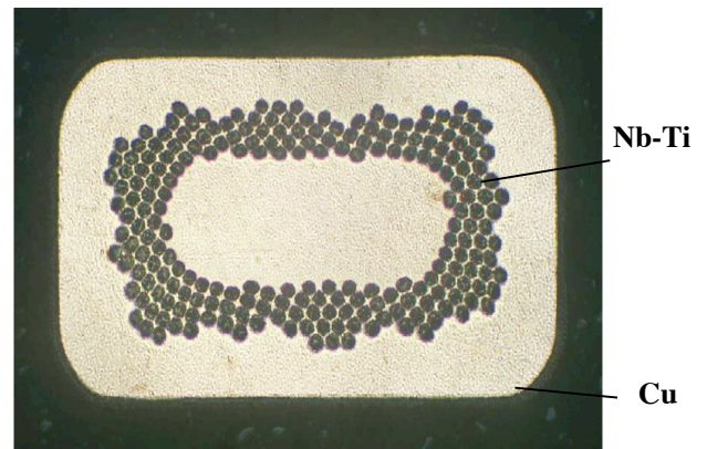
Figure 1 Coupling magnet conductor cross-section with 222 Nb-Ti filaments in a copper matrix ( I_c = 760 \text{ A @ } 5 \text{ T \& } 4.2 \text{ K} )
