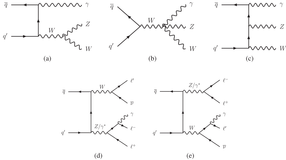
FIG. 1. Representative leading-order Feynman diagrams for (a)–(c) WZ\gamma production and (d), (e) \ell'^{\pm}\nu\ell^+\ell^-\gamma production via the FSR processes Z \rightarrow \ell^+\ell^-\gamma and W \rightarrow \ell'\nu\gamma .
