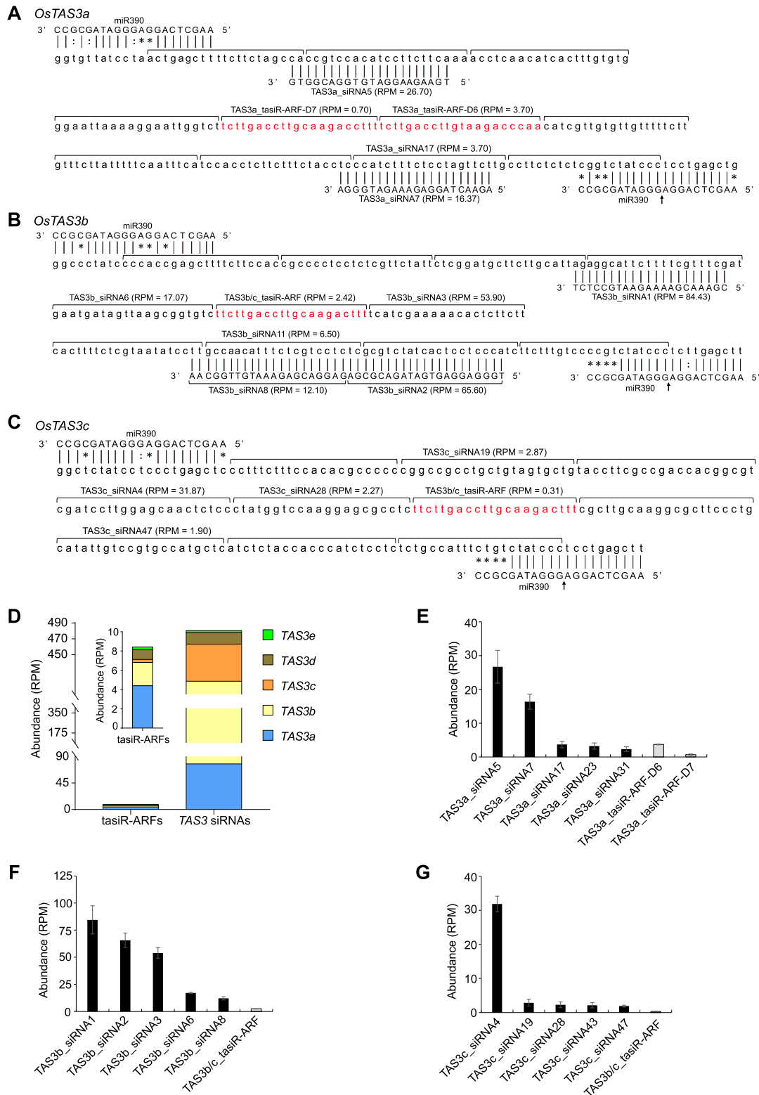
Figure 1 Sequences of TAS3 genes and abundance of TAS3 siRNAs in rice. A–C, Sequences of TAS3a (A), TAS3b (B), and TAS3c (C) transcripts between the two miR390 recognition sites. The phased siRNAs are indicated by brackets, and the register of the phased siRNAs is determined by cleavage (arrow) at the 3′-miR390 recognition site. The sequences of rice tasiR-ARFs, which are adopted from tasiRNADB (https://bioinfo.jit.edu.cn/tasiRNADatabase), are indicated in red. The siRNAs with high abundance are labeled, and their mean abundance in the small RNA libraries is displayed in parentheses. D, Cumulative abundance of tasiR-ARFs and TAS3 siRNAs from the five TAS3 loci in rice. “RPM” is short for “reads per million mapped reads.” E–G, Abundance of tasiR-ARFs and top-ranked non-tasiR-ARF TAS3 siRNAs generated from TAS3a (E), TAS3b (F), and TAS3c (G) transcripts in rice. Each analysis includes three independent replicates. The abundance of siRNAs is displayed as mean ± standard deviation.
