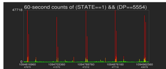
Figure 3. Drilling even deeper into the data, the suspicious activity occurs daily at 21:15 local time.
