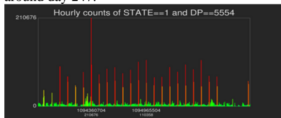
Figure 2. Drilling into the data, we compute and display a histogram of suspicious activity over a four-week period at one-hour temporal resolution. Evidence of regular activity becomes apparent.
