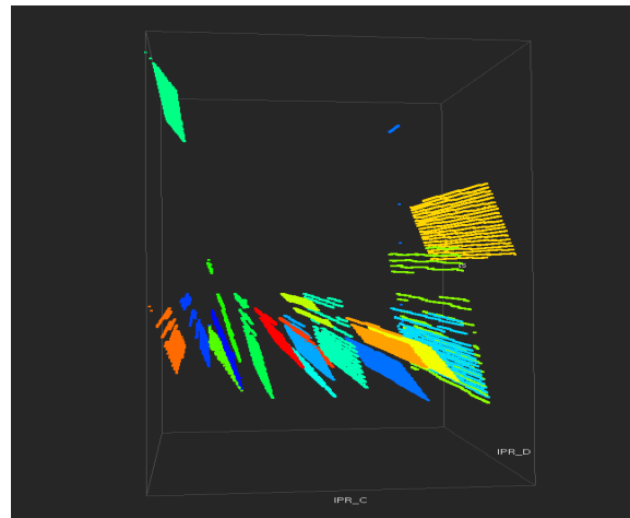
Figure 4. After several more query/display iterations, we determine the IP addresses of the twenty remote hosts participating in a distributed scan of a major DOE computing facility. This image shows the destination addresses being attacked by the twenty different hosts during one of the attack cycles.
