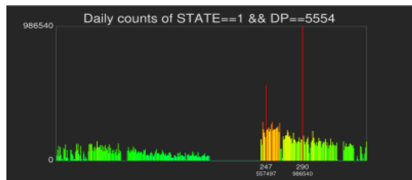
Figure 1. Histogram of suspicious activity over a one-year period at one-day granularity. Coordinated activity appears in the weeks around day 247.
