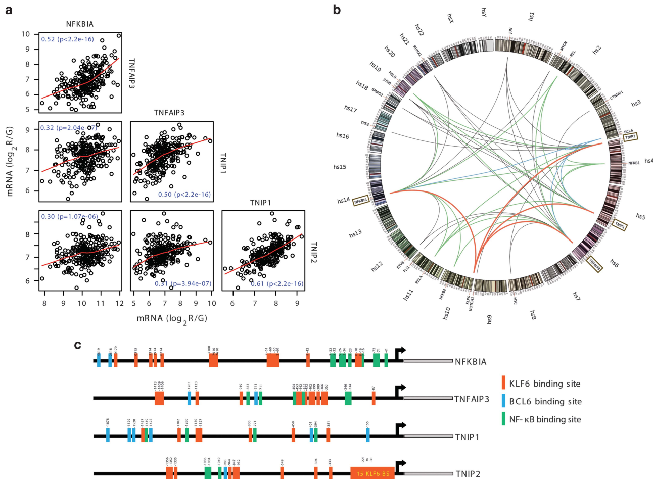
Figure 1. Negative regulators of NF- \kappa B are co-regulated in glioblastoma. (a) Scatter plot matrix for messenger RNA expression of NF- \kappa B control genes NFKB1A , TNFAIP3 , TNIP1 and TNIP2 representing pairwise associations between each of these variables in 188 glioblastomas. Locally weighted least squares smooth fits indicate the appropriateness of the linear regression analyses. The corresponding P -values indicate the statistical significance of these relationships according to estimated slope of the regression line. (false discovery rate adjusted q < 1 \times 10^{-5} ). (b) Genome-wide correlation analysis of the four NF- \kappa B control genes ( TNIP1 , TNIP2 , NFKB1A , TNFAIP3 ) with other gene transcripts in 413 glioblastomas (significance level: P < 1 \times 10^{-5} ). Significant associations between the NF- \kappa B-negative regulators and Rel-like domain-containing proteins ( NFKB1 , NFKB2 , RELA , c-REL and RELB ) are indicated by green edges. Edges connecting the control genes to KLF6 and BCL6 , red and blue, respectively. (c) Schematic diagram of predicted binding sites of transcription factors KLF6 , BCL6 and NF- \kappa B in the promoter regions of the four NF- \kappa B control genes ( NFKB1A , TNFAIP3 , TNIP1 and TNIP2 ).
