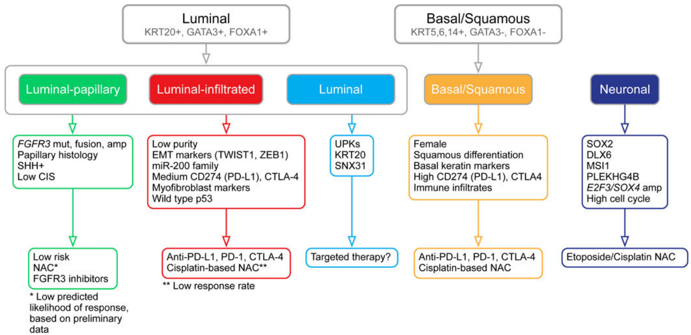
Figure 7. Proposed schema of expression-based, subtype-stratified therapeutic approach as a framework for prospective hypothesis testing in clinical trials. * For luminal-papillary cases, the low predicted likelihood of response is based on preliminary data from (Seiler et al., 2017). See Discussion.
