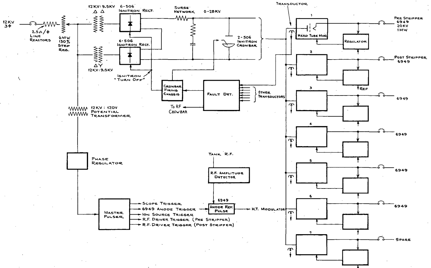
BERKELEY HILAC OSCILLATOR ANODE POWER SUPPLY
