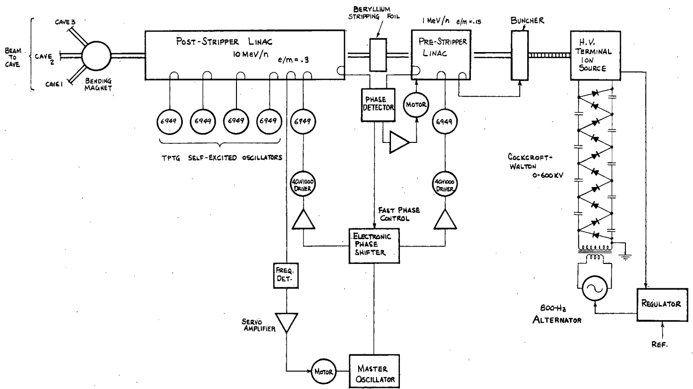
BERKELEY HILAC R.F. SYSTEM
