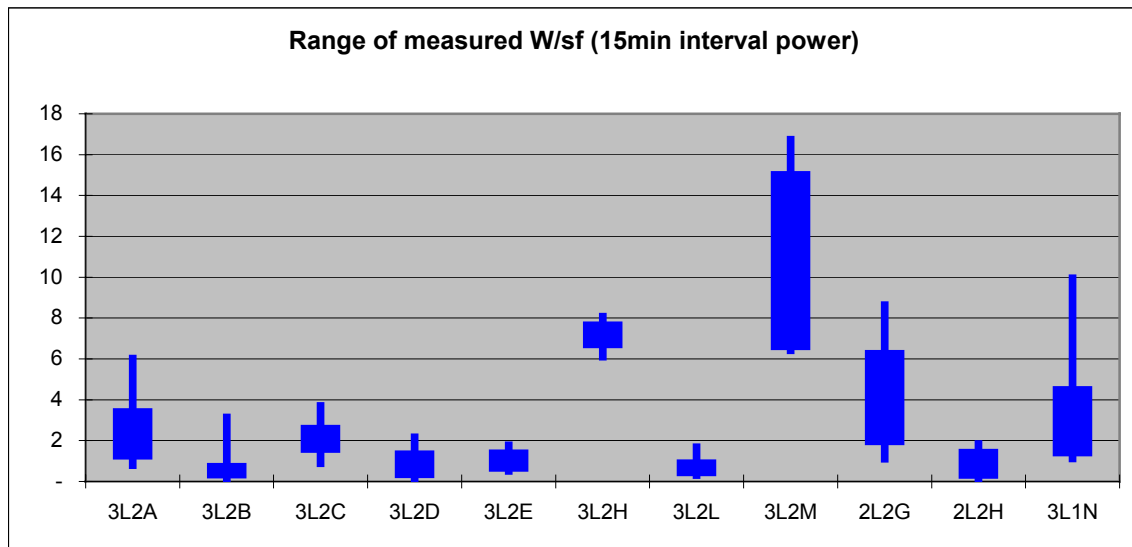
Figure 5. Range of measured 15-min interval power for various laboratory spaces in a building at UC Davis. The upper and lower ends of the lines represent maximum and minimum respectively. The upper and lower ends of the boxes represent 99 th and 1 st percentiles of the measurements respectively.
