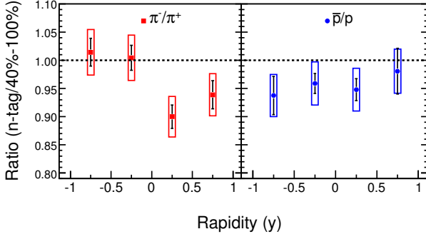
FIG. 13: (Color online) Variation of double ratio (\pi^-/\pi^+)_{n\text{-tag}}/(\pi^-/\pi^+)_{40\text{-}100\%} and (\bar{p}/p)_{n\text{-tag}}/(\bar{p}/p)_{40\text{-}100\%} with rapidity for 2.5 < p_T < 10 GeV/c for d+Au collisions at \sqrt{s_{NN}} = 200 GeV. The boxes are the systematic errors.
