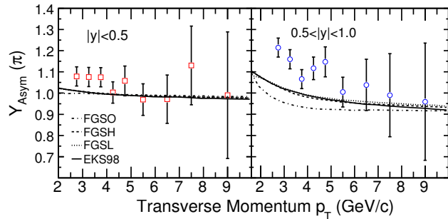
FIG. 6: (Color online) High transverse momentum rapidity asymmetry factor ( Y_{\text{Asym}} ) for \pi^+ + \pi^- at |y| < 0.5 and 0.5 < |y| < 1.0 for minimum bias d+Au collisions at \sqrt{s_{\text{NN}}} = 200 GeV compared to a model with only nuclear shadowing [1]. The different curves represent different parametrization of nuclear shadowing. See text for more details.
