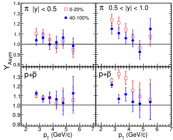
FIG. 5: (Color online) Centrality dependence of high transverse momentum rapidity asymmetry factor ( Y_{\text{Asym}} ) for \pi^+\pi^- and p+\bar{p} at |y| < 0.5 (left panels) and 0.5 < |y| < 1.0 (right panels) for d+\text{Au} collisions at \sqrt{s_{\text{NN}}} = 200 \text{ GeV} .
