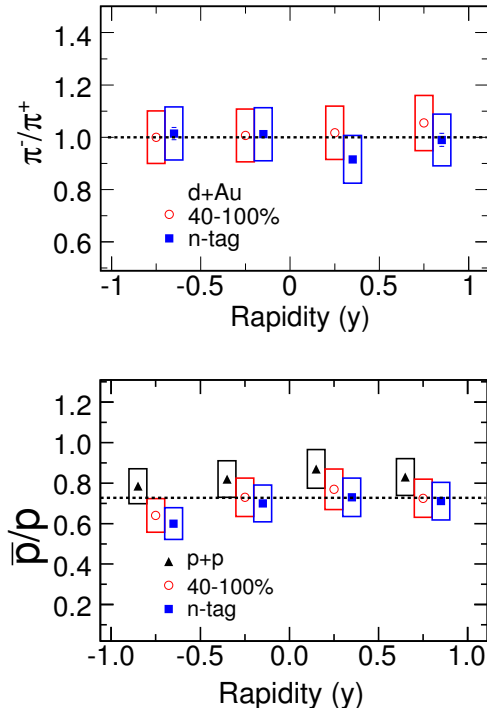
FIG. 12: (Color online) Variation of \pi^-/\pi^+ and \bar{p}/p with rapidity for 2.5 < p_T < 10 \text{ GeV}/c for peripheral (40-100%) and n -tag events for d+Au collisions at \sqrt{s_{NN}} = 200 \text{ GeV} . Also shown for comparison are the \bar{p}/p for minimum bias p+p collisions. The boxes are the systematic errors. The ratios for n -tag events are shifted by 0.05 units in rapidity and those for p+p collisions by -0.05 units in rapidity for clarity of presentation.
