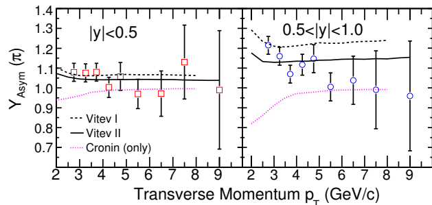
FIG. 7: (Color online) High transverse momentum rapidity asymmetry factor ( Y_{\text{Asym}} ) for \pi^+ + \pi^- at |y| < 0.5 and 0.5 < |y| < 1.0 for minimum bias d+Au collisions at \sqrt{s_{\text{NN}}} = 200 GeV compared to models incorporating multiple scattering, shadowing, and energy loss in cold nuclear matter [3]. See text for more details.
