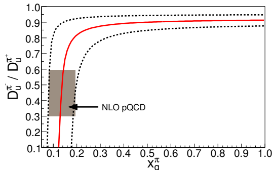
FIG. 14: (Color online) Variation of \frac{D_u^{\pi^-}}{D_u^{\pi^+}} with fraction of pions ( x_q^{\pi} ) originating from quark jets (solid line) obtained from the measured ratios of \pi^-/\pi^+ in peripheral d +Au collisions and n -tag events. The dashed lines reflect 1\sigma systematic errors in obtaining the \frac{D_u^{\pi^-}}{D_u^{\pi^+}} . The horizontal shaded band reflects the possible x_q^{\pi} range obtained from NLO pQCD calculations using AKK fragmentation functions [34].
