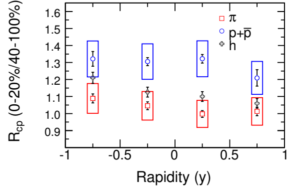
FIG. 11: (Color online) Variation of nuclear modification factor ( R_{\text{CP}} ) for \pi^+\pi^- and p+\bar{p} with rapidity for p_T > 2.5 GeV/ c for d +Au collisions at \sqrt{s_{\text{NN}}} = 200 GeV. Also shown for comparison are the R_{\text{CP}} values for inclusive charged hadrons as a function of pseudorapidity [5]. The errors shown as boxes are the systematic errors. The error due to number of binary collisions is \sim 14\% and is not shown in the figure.
