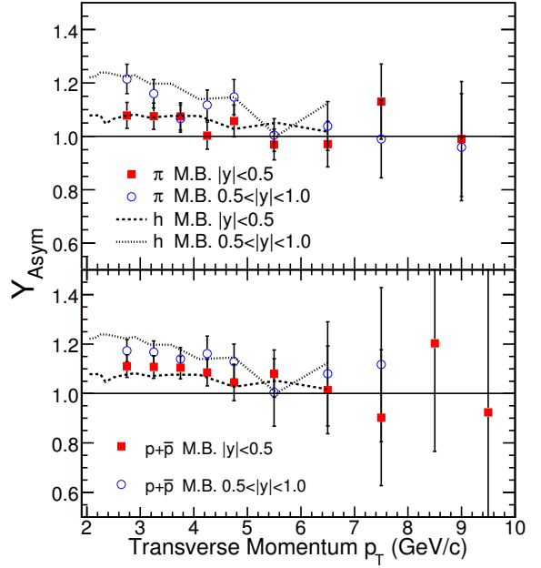
FIG. 4: (Color online) High transverse momentum rapidity asymmetry factor ( Y_{\text{Asym}} ) for \pi^+\pi^- and p+\bar{p} for |y| < 0.5 and 0.5 < |y| < 1.0 for minimum bias d+\text{Au} collisions at \sqrt{s_{\text{NN}}} = 200 \text{ GeV} . For comparison the inclusive charged hadron results from STAR [5] are also shown by the curves.
