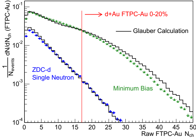
FIG. 1: (Color online) Uncorrected charged particle multiplicity distributions measured in -3.8 < \eta < -2.8 (Au-direction) for d+Au collisions. Points are for minimum bias (triangles) and peripheral (circles, ZDC-d single neutron) collisions [15]. Both are normalized to the total number of d+Au collisions. Histograms are Glauber model calculations.
