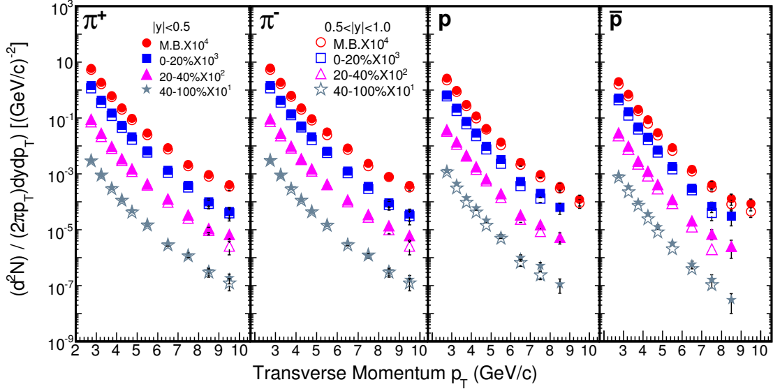
FIG. 3: (Color online) High transverse momentum spectra ( p_T > 2.5 GeV/c) of charged pions, proton, and anti-proton for the rapidity regions |y| < 0.5 (solid symbols) and 0.5 < |y| < 1.0 (open symbols) for d+Au collisions and various event centrality classes at \sqrt{s_{NN}} = 200 GeV.
