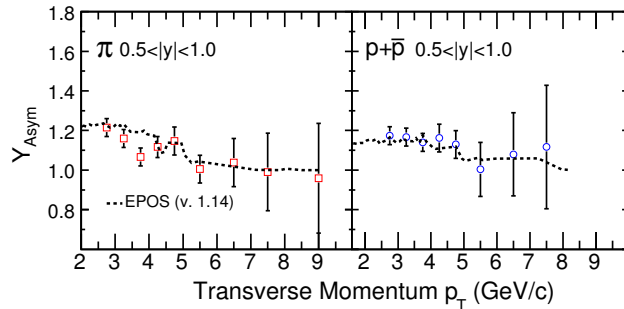
FIG. 8: (Color online) High transverse momentum rapidity asymmetry factor ( Y_{\text{Asym}} ) for \pi^+ + \pi^- and p + \bar{p} for 0.5 < |y| < 1.0 for minimum bias d+Au collisions at \sqrt{s_{\text{NN}}} = 200 GeV compared to the EPOS model [7]. See text for more details.
