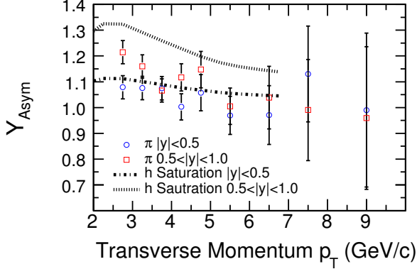
FIG. 10: (Color online) High transverse momentum rapidity asymmetry factor ( Y_{\text{Asym}} ) for \pi^+\pi^- at |y| < 0.5 and 0.5 < |y| < 1.0 for minimum bias d +Au collisions at \sqrt{s_{\text{NN}}} = 200 GeV compared to the saturation model [4]. See text for more details.
