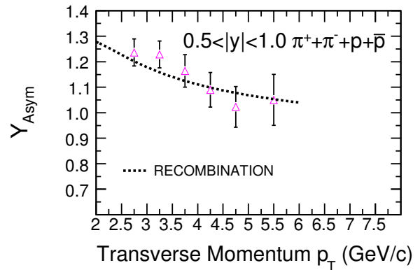
FIG. 9: (Color online) High transverse momentum rapidity asymmetry factor ( Y_{\text{Asym}} ) for \pi^+ + \pi^- + p + \bar{p} and 0.5 < |y| < 1.0 in 0–20% central d+Au collisions at \sqrt{s_{\text{NN}}} = 200 GeV compared to the recombination model [6]. See text for more details.
