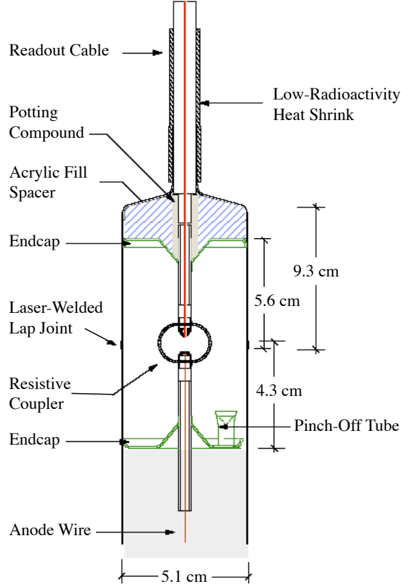
Fig. 7. Schematic of the single-ended readout with the cable bell connected to the top NCD of a string.
