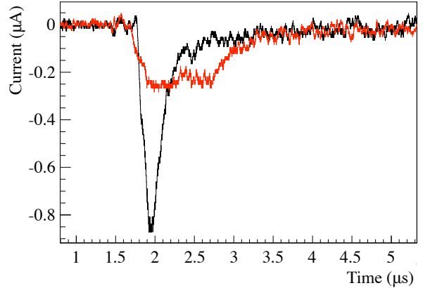
Fig. 13. Digitized current pulses of two neutron-capture events. The wider pulse had the proton-triton track nearly perpendicular to the anode wire, and the narrower pulse had the track nearly parallel to the anode wire.
