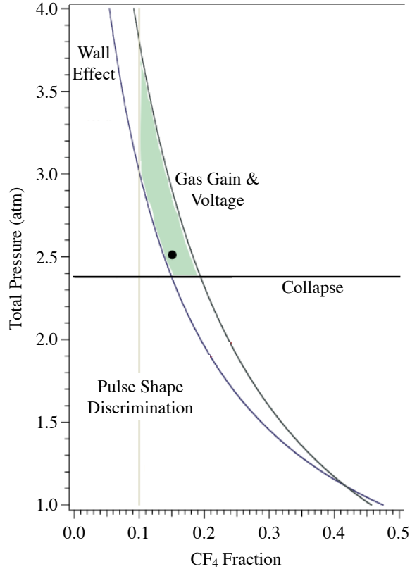
Fig. 5. Optimization of gas fill fraction and pressure. The shaded region shows the \text{CF}_4 fraction and total pressure that fit the scientific and mechanical constraints (explained in the text). The dot shows the pressure and \text{CF}_4 fraction chosen for the NCD array.
