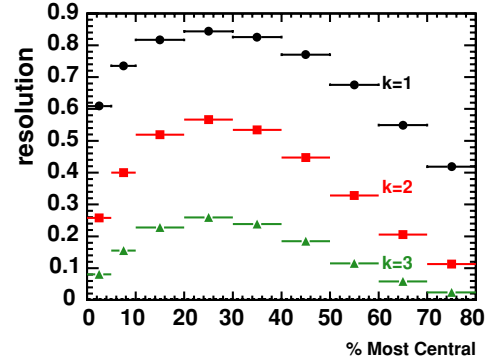
FIG. 1. (Color online) The event plane resolutions as a function of centrality for v_{k2}\{EP_2\} .
