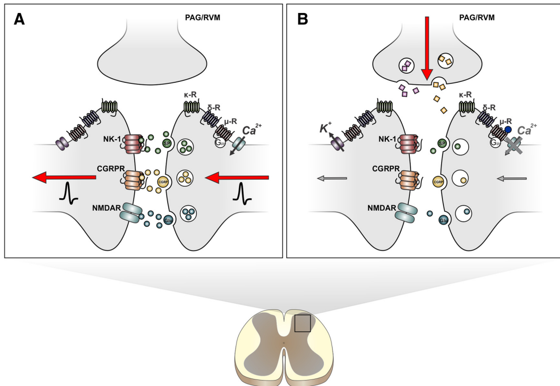
Figure 1. Spinal mechanisms of opioid analgesia. A , In the spinal dorsal horn, nociceptive signals encoded by action potentials trigger the release of nociceptive transmitters, such as substance P (SP), calcitonin gene-related peptide (CGRP), and L-glutamate (Glu). Second-order projection neurons then relay this information from the spinal cord to the brain, where the information is disseminated and decoded to produce the emotional and sensory experiences of pain. B , Opioids produce their analgesic effects by inhibiting spinal nociceptive transmission. On presynaptic nerve terminals, opioids reduce cAMP signaling and suppress activity of voltage-gated calcium channels, which inhibits release of nociceptive transmitters. On postsynaptic neurons, opioids activate inward potassium channels to cause hyperpolarization of ascending projection neurons. Opioids also produce analgesia by activating descending inputs from the periaqueductal gray (PAG) and rostral ventromedial medulla (RVM), which are key components of the descending inhibitory pain pathways. In these supraspinal structures, opioid-mediated disinhibition of GABAergic interneurons leads to activation of monoamine-containing descending neurons that suppress nociceptive transmission in the spinal dorsal horn. CGRPR, Calcitonin gene-related peptide receptor; NK-1, neurokinin-1 receptor.
