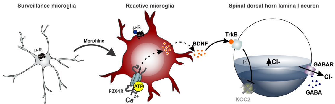
Figure 2. Microglial-mediated disruption of chloride homeostasis in spinal lamina I neurons gates morphine hyperalgesia. In response to chronic morphine treatment, microglia residing in the spinal cord adopt a reactive state characterized by \mu receptor-dependent upregulation of P2X 4 R expression. Activation of P2X 4 R causes the release of BDNF, which signals to downregulate the potassium-chloride cotransporter KCC2, resulting in a dysregulation of chloride homeostasis in spinal lamina I pain signaling neurons. The P2X 4 R–BDNF–KCC2 pathway is not only critical for the paradoxical hyperalgesic effect of morphine but also for pain hypersensitivity after peripheral nerve injury.
