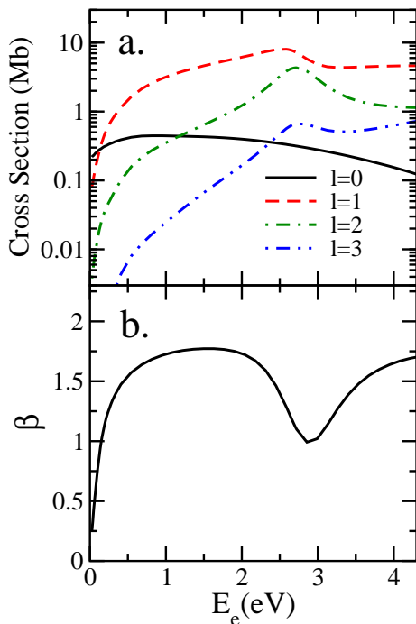
FIG. 4: (Color online) a) Partial photodetachment cross section for \text{trans-HOCO}^- summed over quantum number m . b) Beta parameter for \text{trans-HOCO}^- . The calculations are done using transition-state orbitals.
