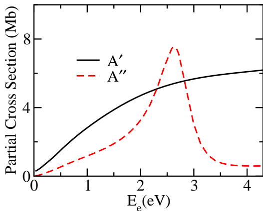
FIG. 3: (Color online) A' and A'' components of the photodetachment cross section for \text{trans-HOCO}^- calculated using transition-state orbitals.
