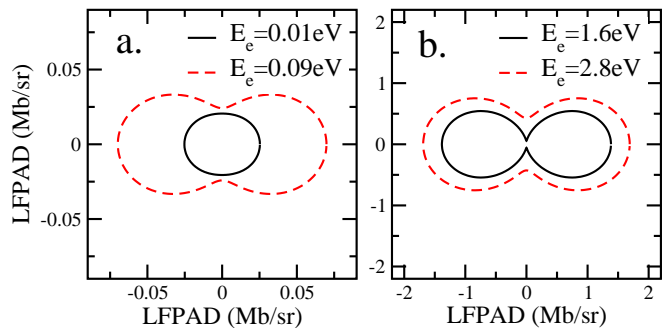
FIG. 5: (Color online) a) Near threshold laboratory frame photoelectron angular distributions for \text{trans-HOCO}^- . b) The distributions plotted near the resonance energy.
