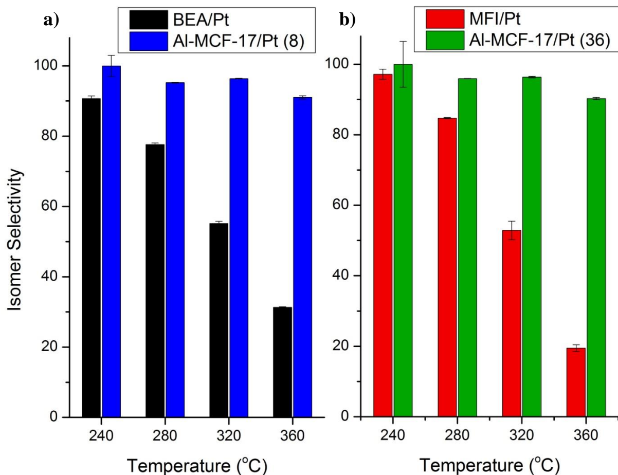
Figure 4. a) Isomer selectivities for BEA/Pt zeolite (black) and Al-MCF-17/Pt (blue). Both catalysts shown contain a Si:Al ratio of 8:1. b) Isomer selectivities for MFI/Pt (red), and Al-MCF-17/Pt (green). Both catalysts shown contain a Si:Al ratio of 36:1. In both plots the zeolite catalysts (BEA/Pt and MFI/Pt) drop in isomer selectivity as the reaction temperature increases. The Al modified MCF-17/Pt catalysts retain high isomer selectivity at higher temperatures. A more detailed version of this figure, with additional temperature points, is shown in Figure S5.
