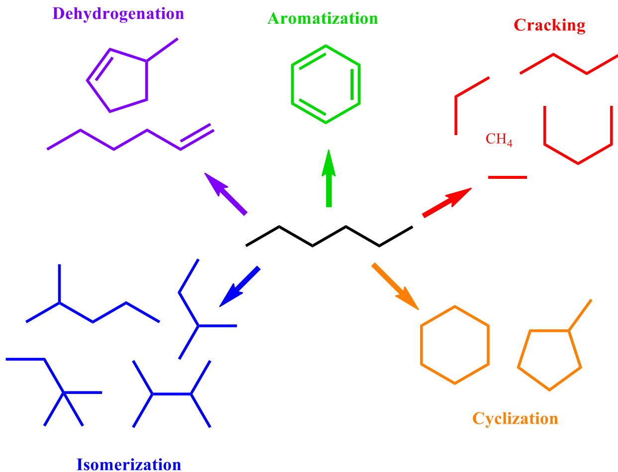
Figure 1. Scheme showing the possible products in the catalytic reforming of n-hexane. Isomerization and cyclization products are desired, while dehydrogenation, aromatization and cracking are undesired. For all catalysts studied in this work, excluding unmodified MCF-17/Pt, isomer and cracking products accounted for over 98% of the total reaction products. The unmodified MCF-17/Pt catalyst also produced methylcyclopentane via cyclization.
