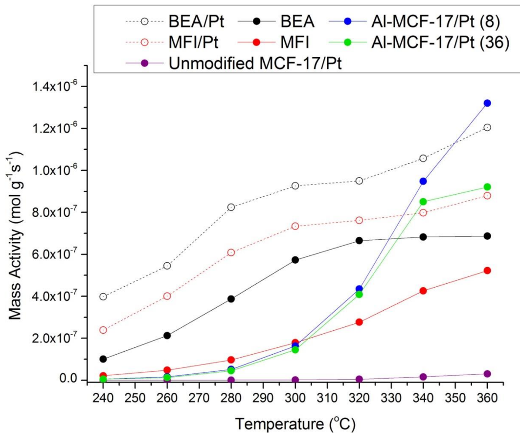
Figure 2. Mass activity (in terms of total moles of n-hexane converted per gram of catalyst per second) for all studied catalysts.
