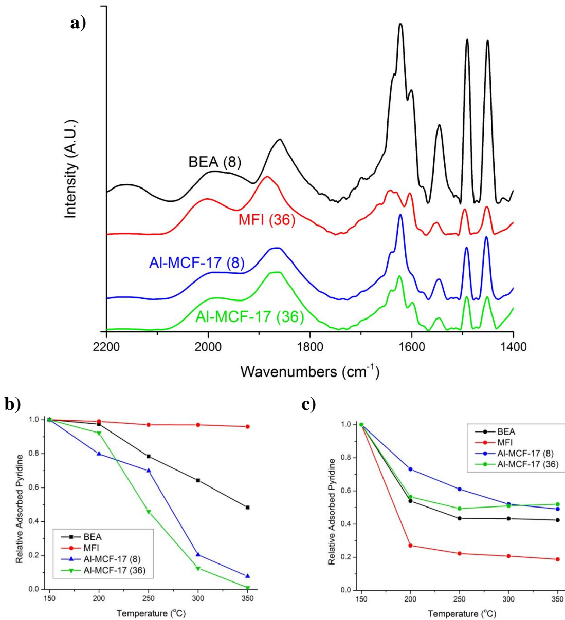
Figure 5. a) FT-IR spectra of pyridine adsorbed onto mesoporous BEA (black), mesoporous MFI zeolite (red), aluminum modified MCF-17 with an 8:1 Si:Al ratio (blue) and aluminum modified MCF-17 with a 36:1 Si:Al ratio (green). The IR spectra are normalized with the band between 2100 and 1750 \text{cm}^{-1} , which originates from the Si-O-Si stretch. After pyridine adsorption, both Brönsted and Lewis acid sites are distinguishable at 1550 and 1450 \text{cm}^{-1} , respectively. Utilizing the adsorption coefficients of 1.13 \text{cm}/\mu\text{mol} for Brönsted sites and Lewis 1.28 \text{cm}/\mu\text{mol} for Lewis acid sites, the amount of each type of sites can be quantified (shown in Table 1). Si:Al ratios for each material are shown in parenthesis. b) The relative amount (normalized to initial spectrum at 150 ^{\circ}\text{C} ) of Brönsted acid sites determined from FT-IR of adsorbed pyridine at 1550 \text{cm}^{-1} as a function of temperature. It can be seen that the amount of
