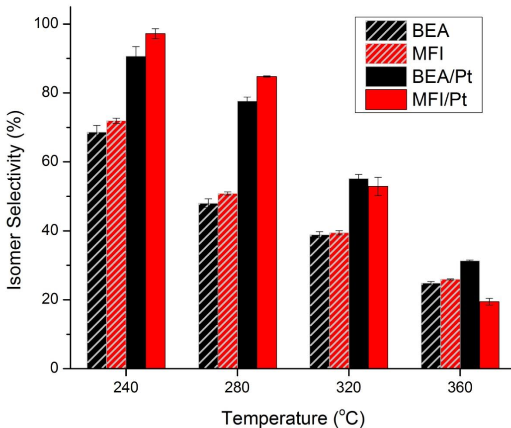
Figure 3. Total isomer selectivity of BEA (black/gray), MFI (red/gray), BEA/Pt (black) and MFI (red). It can be seen that at low temperatures the isomer selectivity is higher when Pt NPs are present in the mesopores of the zeolites. However, at higher temperatures the selectivity is nearly the same with or without Pt present, indicating the micropores of the zeolite dominate the catalytic chemistry. A more detailed plot with additional temperature points is shown in Figure S3.
