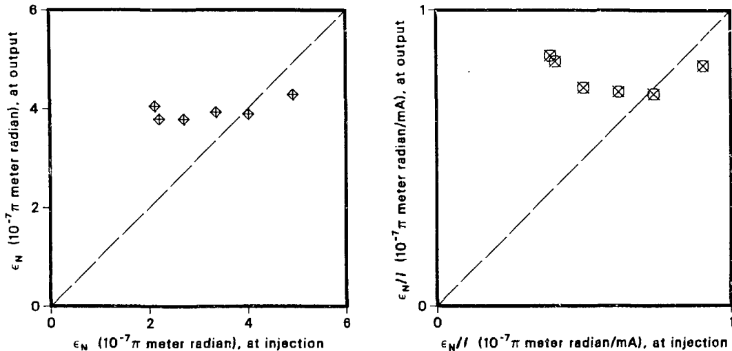
Figure 5.19: Threshold measurement for \sigma_0 = 124^\circ , showing behavior similar to that for \sigma_0 = 118^\circ . Emittance growth for unstable injection is accompanied by a small beam loss for the larger-diameter beam used here. The beam loss diminishes as the input emittance is increased, with the output emittance remaining nearly constant until the injection emittance rose above about 3.5 \times 10^{-7}\pi meter radian. The plot of \epsilon_N/I at the end of the SBTE vs. the corresponding value at injection shows the same general features as for \sigma_0 = 118^\circ . The total beam current is about 5.4 mA.
