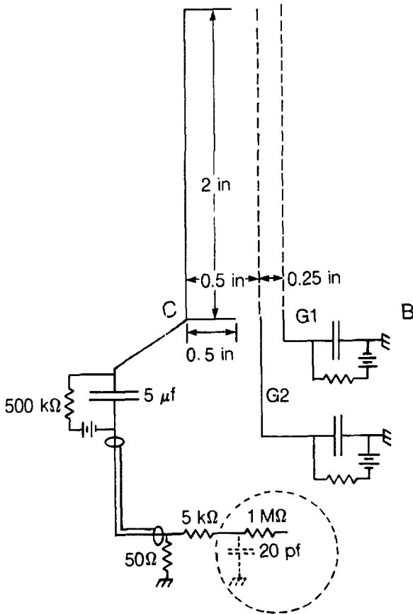
Shallow Faraday Cup
