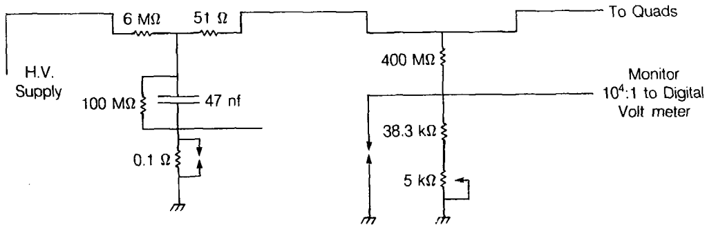
Quadrupole Power Supply Stiffener and Monitor Circuitry
