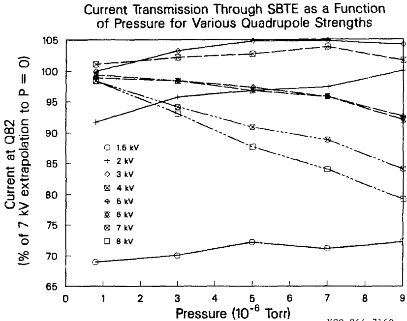
Figure 6.7: Current vs. pressure in SBTE lattice at 120 keV particle energy. Second ionization of the \text{Cs}^+ ions causes loss of the ion for quadrupole voltages above about 7.5 kV, because \sigma_0 > 180^\circ for the resulting \text{Cs}^{2+} ion. For lower quadrupole voltages, a \text{Cs}^{2+} ion may remain, if its transverse phase space coordinates fall within the acceptance curve for the new charge state. The exponential loss of ions from the beam from the combined processes of second ionization and neutralization may be calculated from the high voltage current vs. pressure curves. If the bore clearance is great, so that all the \text{Cs}^{2+} are retained, the low voltage curves give the exponential drop (or rise) in current as the electrical current is augmented by the \text{Cs}^{2+} ions. If the second ionization rate exceeds the neutralization rate, the current rises with pressure until the depopulation of \text{Cs}^{2+} ions by other processes becomes important. The very low voltage curves for the 120 keV ions show a distinct rise in current at the Q82 Faraday cup, as the pressure rises. This effect disappears for quadrupole voltages greater than about 4 kV.
