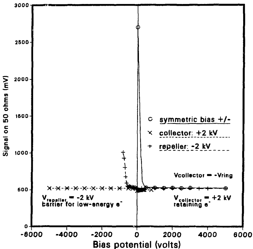
Figure B.2: Bias curves for the DFC. With biases for the collector and the repeller ring differing only in polarity, the DFC response saturated cleanly in both the secondary electron retention and secondary emission modes. The ion current saturated at \pm 500 \text{ V} , respectively, for the collector and repeller, but we operated at the design bias of \pm 2 \text{ kV} . This maintains a negative potential across the central plane of the repeller ring to prevent any possible entry of low-energy electrons.
