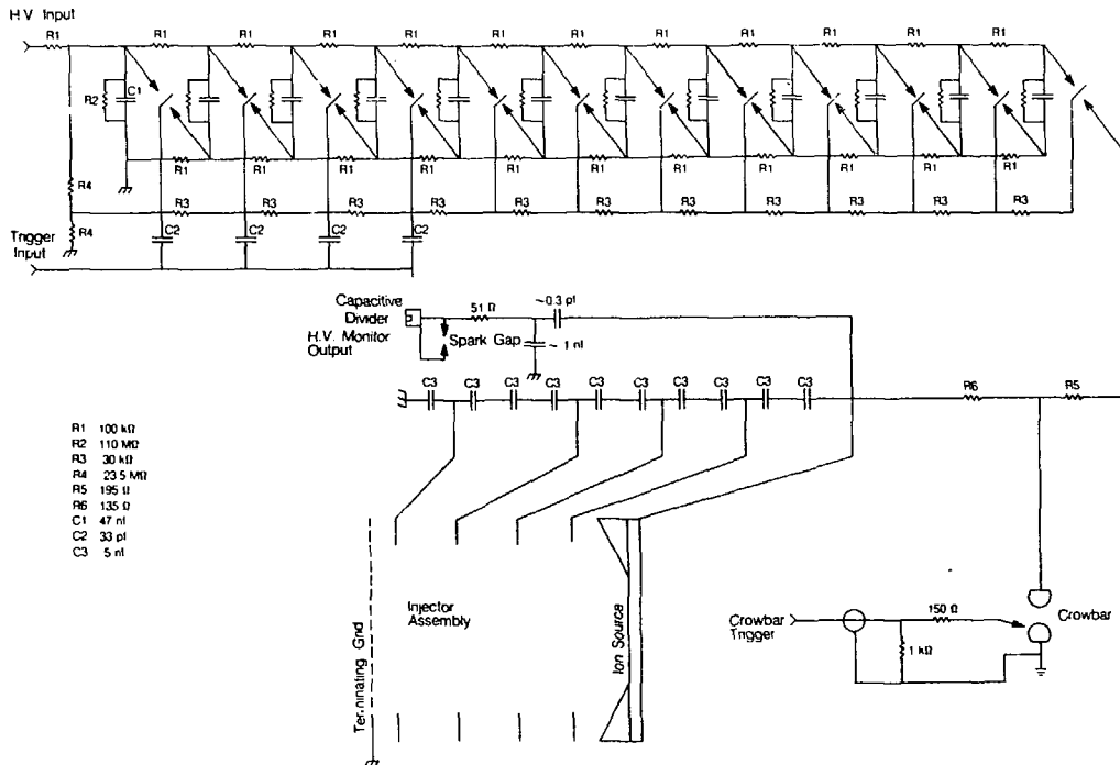
Figure 3.5: Circuit diagram for the SBTE Marx generator, showing the divider circuitry for the high voltage monitor and for the injector aperture voltages, as well as the triggers for the Marx itself and for the crowbar used to terminate the beam pulse.
