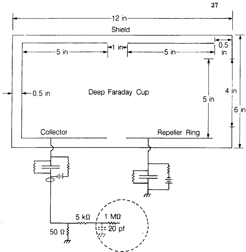
Deep Faraday Cup with Bias and Detector Circuitry
