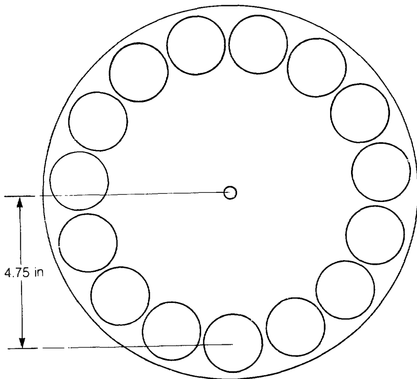
Figure 3.13: Diagnostic wheel assembly. The holes in the wheel were of 1.5-inch diameter to avoid clipping the beam edges. Various attenuator grids were provided, along with blank inserts having either 2-mm or 3-mm diameter holes to generate beamlets for diagnostic purposes.
