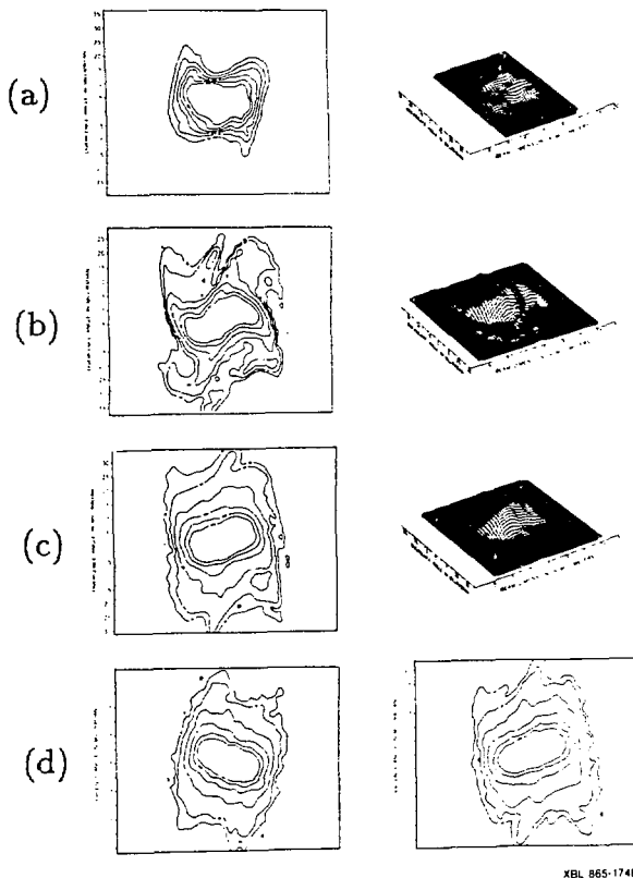
Figure 5.15: Phase space contours for \sigma_0 = 98^\circ . The perspective views are for the contour maps at the left for Q4 in row (a), Q35 in row (b), and Q59 in row (c). In row (d) are contour maps for Q80 (horizontal) on the left and Q76 (vertical) on the right. The evolution of the beam between Q4 and Q35 shows a four-pointed structure which is apparent in our other measurements only for \sigma_0 = 102^\circ . The structure is similar to that shown in some simulation work by Haber and Maschke [45] and by Hofmann [46] for strongly focused beams. As the beam propagates downstream, the structure becomes much less prominent, and the beam ultimately stabilizes.
