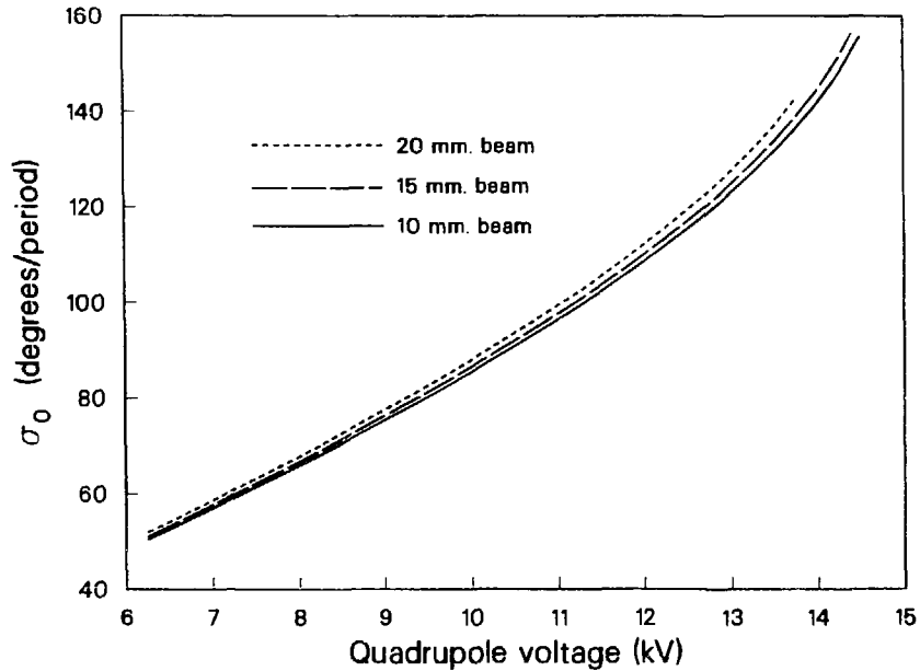
Variation of \sigma_0 with Quadrupole Voltage at Various Oscillation Amplitudes
