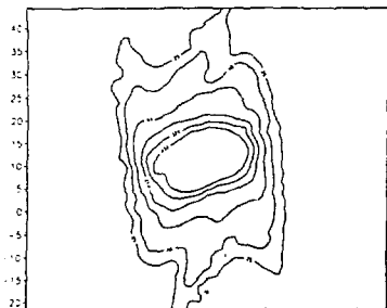
Figure 5.17: Phase space contours for \sigma_0 = 102^\circ . The perspective views correspond to the contour maps to the left of each for (a) Q35, (b) Q59, and (c) Q76. The four-pointed structure again is visible at Q35, and remains visible to some extent at Q59. The beam is very nearly stabilized by this point, evolving little in the remaining transport to Q76.
