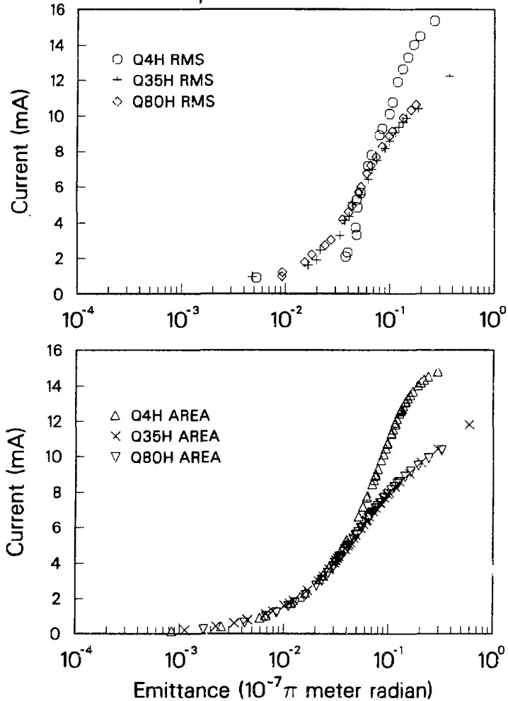
Figure 5.28: Current vs. emittance for \sigma_0 = 94^\circ , unstable beam. The core of the beam is little affected during the instability. Most of the change takes place in the outer phase space areas, with the change nearly complete by Q35. Downstream of Q35, the only change is an additional loss of about 2 mA of beam from the phase space tails.
