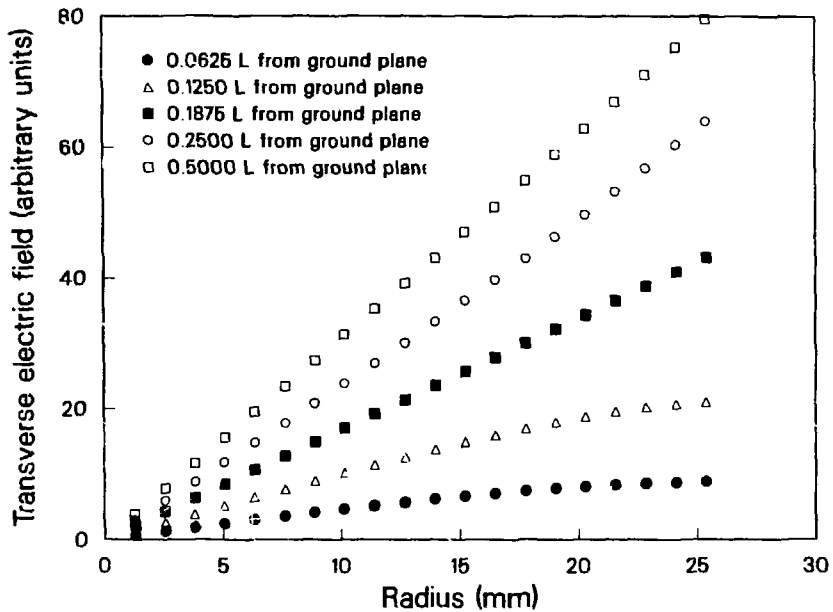
Fields of the SBTE Quads as a Function of Radius at Various Z-positions
