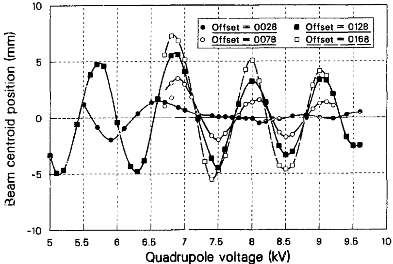
Centroid Position at Q79H vs. Quad Potential for Various x' Values, 0.35 mA
