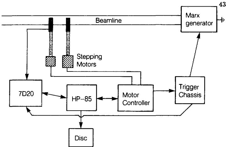
Automated data acquisition network physical layout
