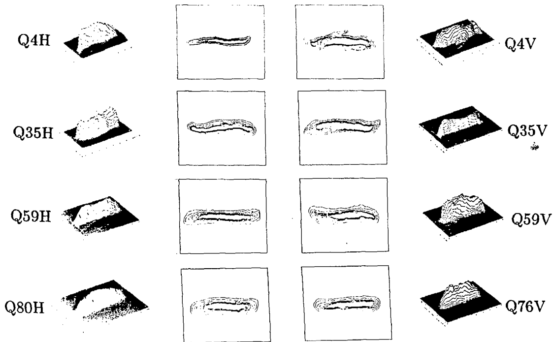
Figure 6.2: Phase space contours at various positions along the SBTE. The two left-most columns show the horizontal dimension results, while the two right-most columns show the vertical dimension data. The interchange of transverse energy is essentially completed upstream of Q35.
