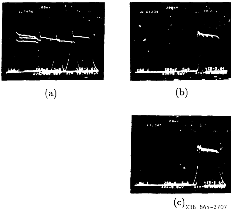
Figure 5.3: (a) Faraday cup traces along the lattice, showing the differences in the direct response to essentially equal beam currents. (b) Deep Faraday cup traces with short fall-times (at M5), showing the separation of the light ion component from the \text{Cs}^+ component in the small step at the trailing edge of the beam pulse before the main pulse ends. (c) Overlay of the \text{Cs}^+ component as measured at M5 and at Q82 using identical DFC's. The long fall-time at Q82 prevents observation of the undershoot at the tail of the pulse. The equality of \text{Cs}^+ component at either end of the lattice to within about 2% (the level of the beam loss from background gas interactions and beam debunching from the Marx generator output droop) may be seen from the oscilloscope traces. The effect of the longitudinal electric field is apparent from the elongation of the beam ends.
