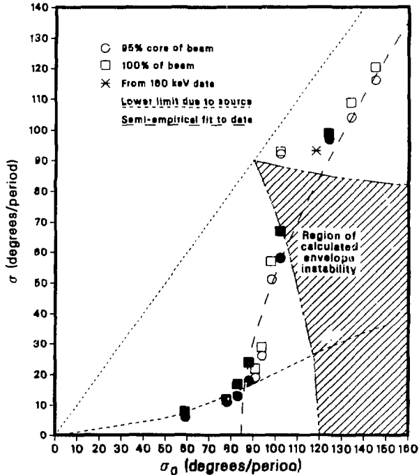
Figure 5.11: Summary of results for empirical stability of beams in A.G. lattice. The shaded region marks the area of instability of the envelope equations. For \sigma_0 < 88^\circ , the data are limited by the emittance of the SBTE source. For \sigma_0 > 88^\circ , the points mark the empirical collective stability boundary. The solid symbols mark beam parameters for which the current and emittance were conserved throughout the SBTE. We have also plotted results for which the beam stabilized during transport through the channel, as discussed in the text for the various cases. The hyperbola plotted with the data is described in section 5.5.
