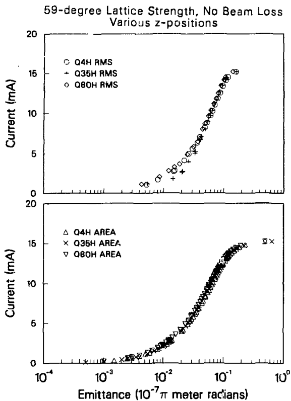
Figure 5.6: Plot of i vs. \epsilon(i) for \sigma_0 = 59^\circ . (a) RMS analysis of emittance, and (b) Area emittance. The distribution is almost linear for i/I < 0.9 when plotted on linear scales. In these and the succeeding figures 5.7 and 5.8, there is no perceptible change in the overall emittance. In the actual phase space data, however, there is a small tail of ions, with a density on the order of 1% of the peak value of the distribution, which forms outside the main beam. This is to be expected from realistic distributions, as a result of thermal tails in the distribution.
