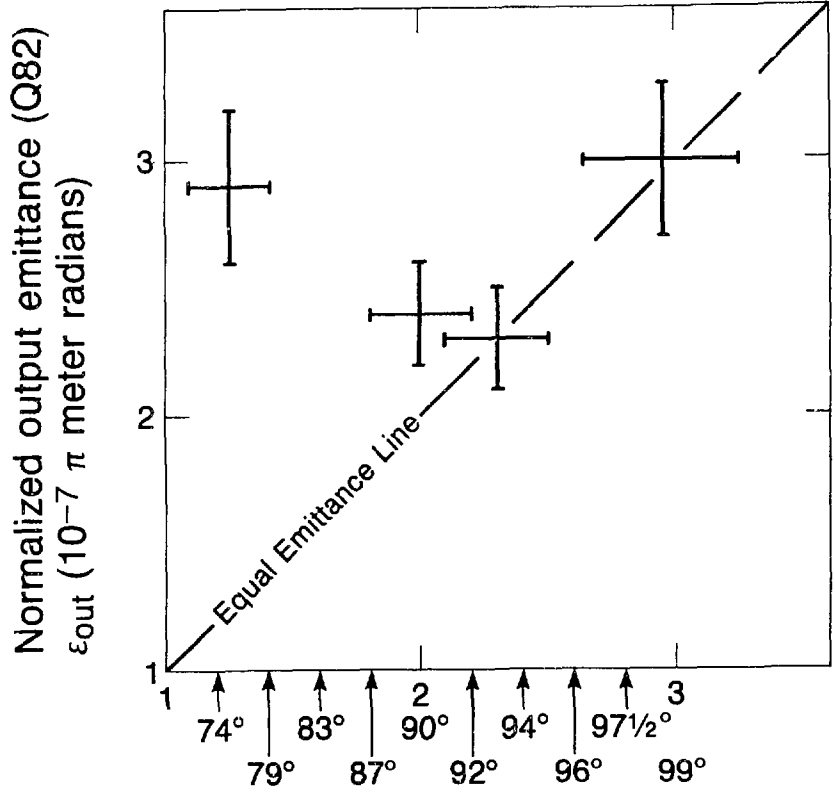
Normalized injection emittance, \epsilon_{in} ( 10^{-7} \pi meter radians)
