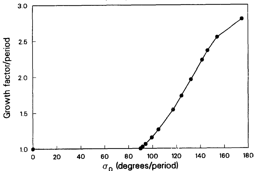
Figure 5.27: Maximum growth rates for the envelope instability for hard-edge quadrupoles with an occupancy factor of 0.5. The thresholds and growth rates were compared with both thin lens quadrupoles and the SBTE model given in Appendix D, and gave agreement within about 1^\circ in thresholds and a few percent in growth rate.
