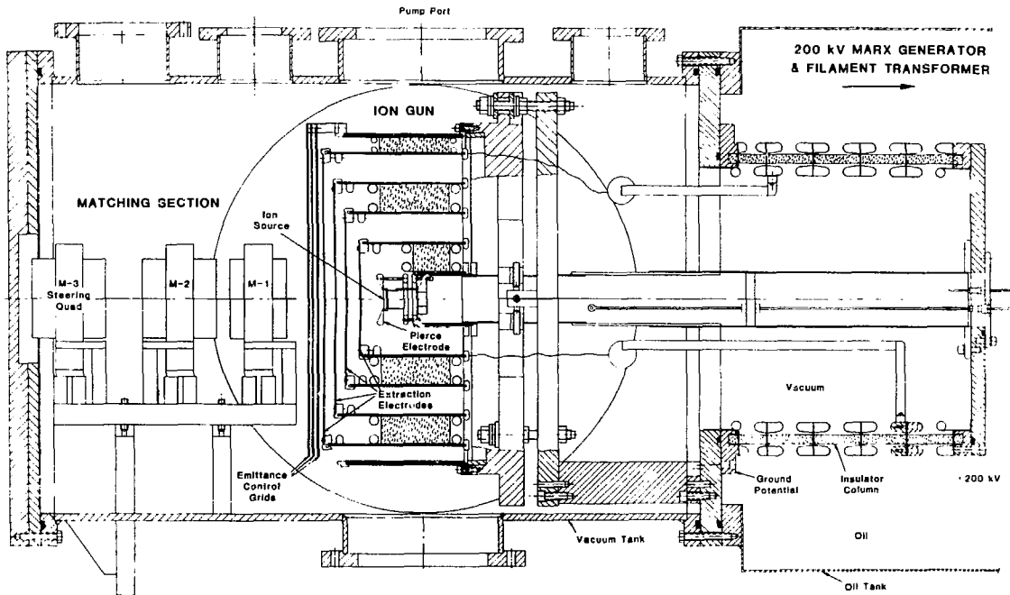
SINGLE BEAM TRANSPORT EXPERIMENT GUN & MATCHING SECTION
