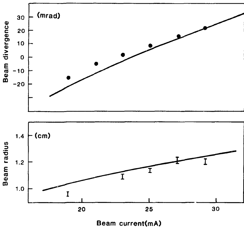
Figure 4.1: Comparison of measured and calculated injector output, with the initial injector design, operating at 160 kV. The agreement with the design values is good.
