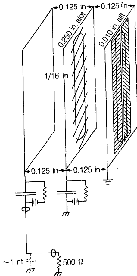
Slit Collector Cup
