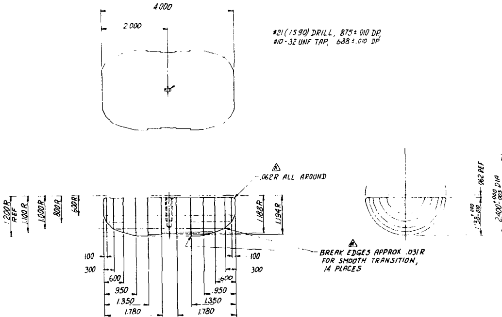
Figure D.1: SBTE electrostatic quadrupole dimensions.
