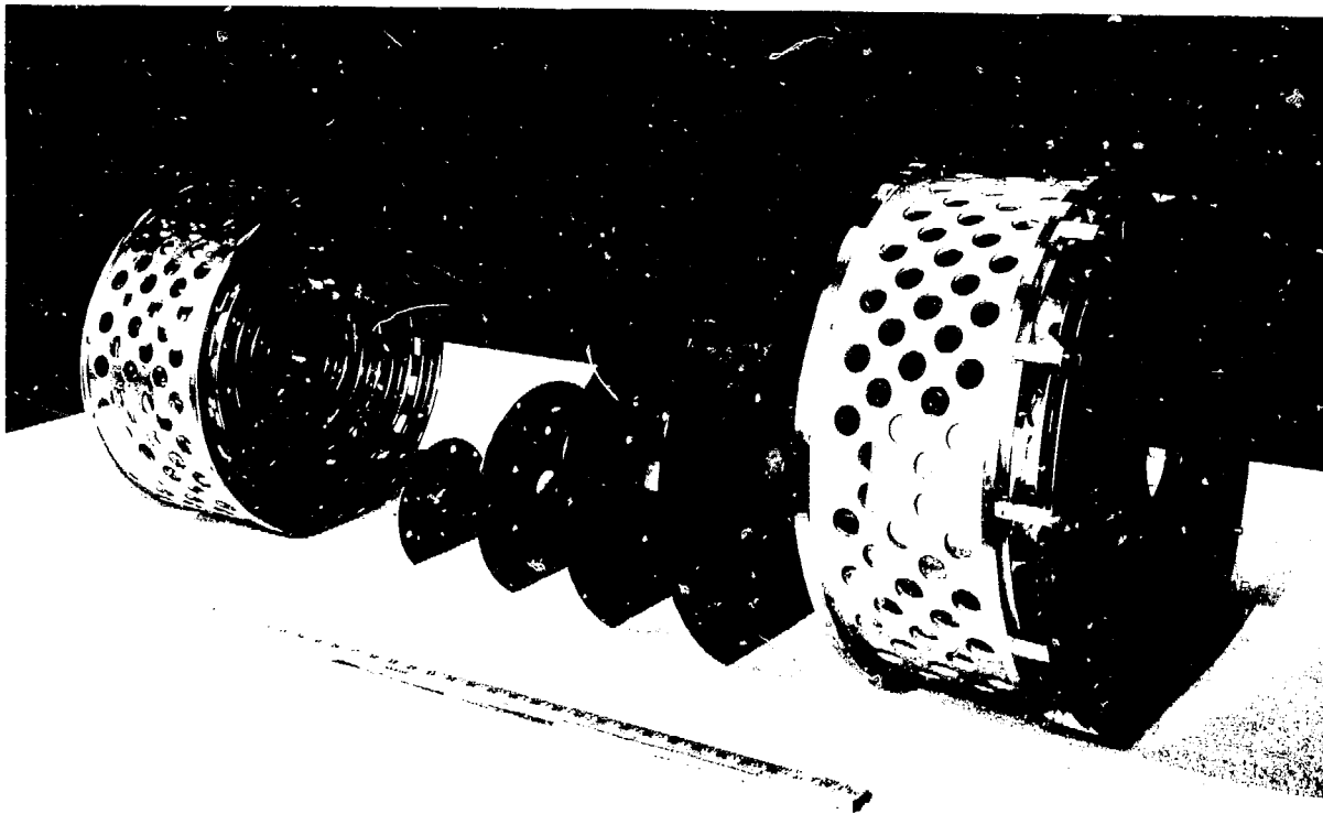
Figure 3.4: Exploded view of the SBTE injector, with the source visible at the center.
