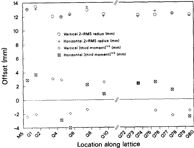
Figure 5.5: The points near the top of the figure show the measured RMS beam radius along the lattice for \sigma_0 = 83^\circ . The envelope oscillation in the two planes is almost exactly in phase, so that the envelope oscillation with these initial conditions is in only one mode. The wavelength, \lambda in units of focusing periods, calculated from the smooth focusing model is such that (360^\circ/\lambda)^2 = 2\sigma_0^2 + 2\sigma^2 . For \sigma_0 = 83^\circ and \sigma \sim 16^\circ , \lambda given by this formula is about three focusing periods, which is in good agreement with the measurements. The third moment of the beam distribution is plotted along the lower portion of the figure. The period of the oscillation is in reasonable agreement with the value 360^\circ/\sigma_0 , as it should from constant-focusing calculations for \sigma much less than \sigma_0 .
