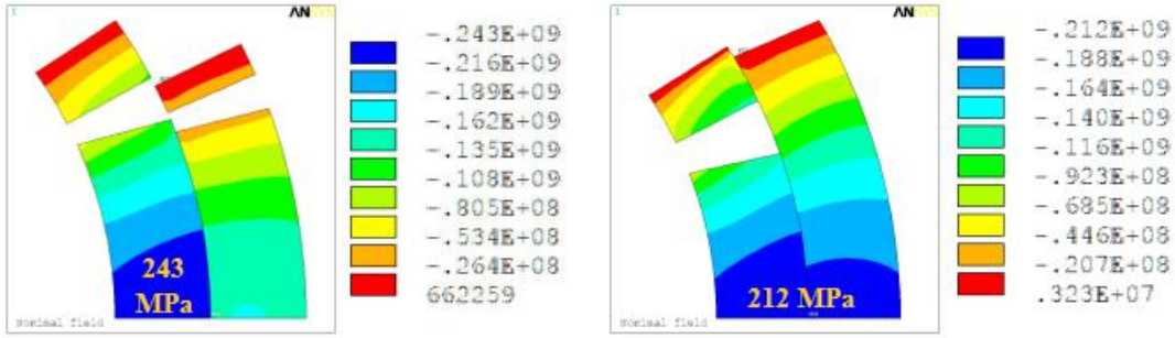
Figure 2: Azimuthal stress distribution due to Lorentz forces at 200 T/m in an infinitely stiff structure with sliding between layers for two 134 mm aperture cross-sections. Left: F_0 L_1 = -3.58 MN/m F_0 L_2 = -2.46 MN/m – Right: F_0 L_1 = -2.7 MN/m F_0 L_2 = -3.4 MN/m
