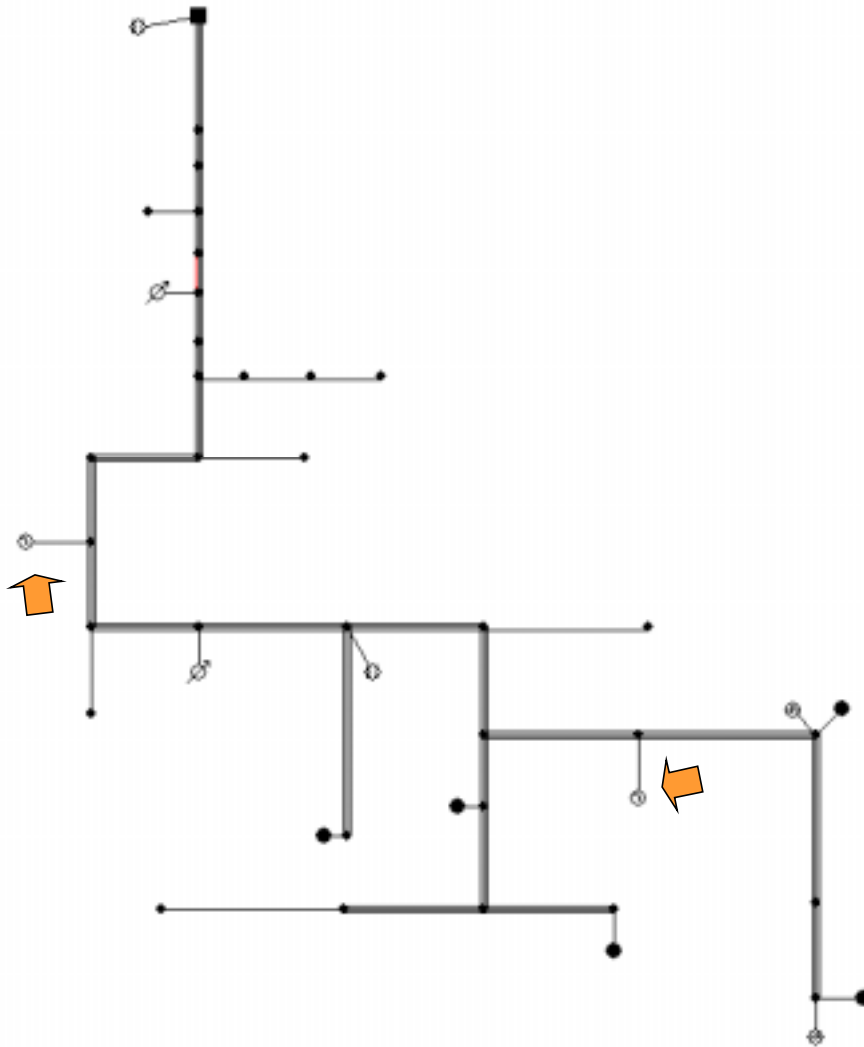
Figure 10: Test Feeder with Embedded Generation
