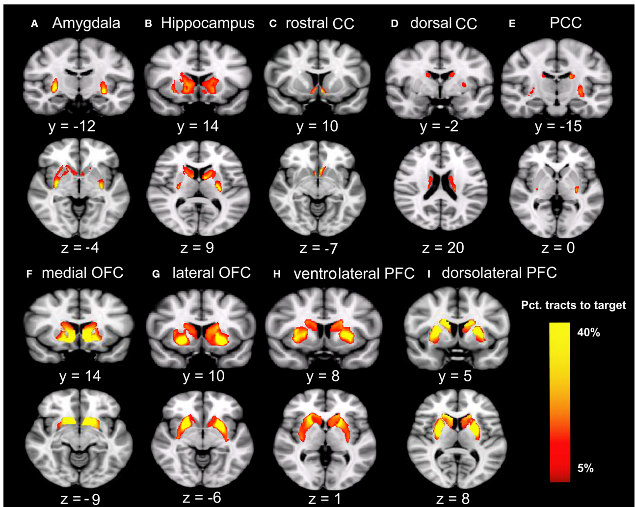
FIGURE 1 | Tracts between the striatum and each of the nine target regions. Only voxels with at least 5% target-ending tracts are displayed. Colors indicate the proportions of target-specific tracts out of all tracts for a given voxel. mOFC, the medial orbitofrontal cortex; IOFC, the lateral orbitofrontal cortex; vlPFC, the ventrolateral prefrontal cortex; dlPFC, the dorsolateral prefrontal cortex; PCC, the posterior cingulate cortex/retrosplenial cortex; dorsal CC, the dorsal cingulate cortex; rostral CC, the rostral cingulate cortex; Amy, amygdala; Hipp, hippocampus. (A) Group-average tractography from the striatum to amygdala. (B) Group-average tractography from the striatum to hippocampus. (C) Group-average tractography from the striatum to rostral CC. (D) Group-average tractography from the striatum to dorsal CC. (E) Group-average tractography from the striatum to PCC. (F) Group-average tractography from the striatum to medial OFC. (G) Group-average tractography from the striatum to lateral OFC. (H) Group-average tractography from the striatum to ventrolateral PFC. (I) Group-average tractography from the striatum to dorsolateral PFC.
