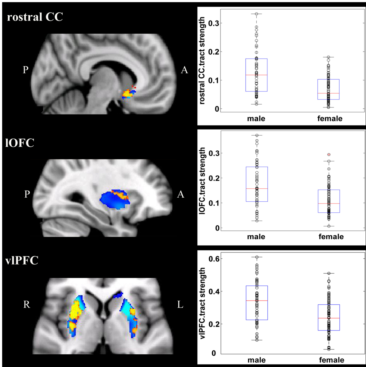
FIGURE 2 | Stronger fiber connection in males than in females. Fiber connections between left caudate and rostral CC (top), between the right putamen and the IOFC (middle), between bilateral caudate and the vIPFC (bottom), and between the putamen and the vIPFC (bottom). Red, stronger connection for males than for females; Blue, proportion of target-specific tracts from Figure 1 . See Figure 1 for abbreviations.
