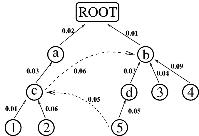
Fig. 8. Tree modification process. Solids arrows show the current tree. Lettered nodes are internal nodes. Numbered nodes are leaf nodes. The cost as leaf is 0.03 for “a” and 0 for “d.” Node “d” is first turned into a leaf. Its child “5” goes to “c.” Then “a” is turned into a leaf. Its child “c” goes to “b.” Note that “c” takes its children “1,” “2,” and “5” together with it.
