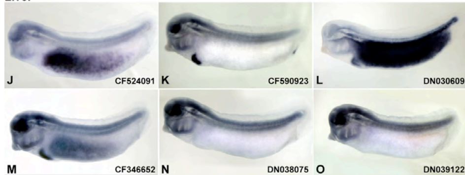
Figure S2. Expression of EST clusters with high representation in adult brain or liver libraries at the tailbud tadpole stage. A-I. EST clusters in which 100% of the constituent ESTs were present in an adult brain library were analyzed by in situ hybridization for their expression at several stages during development. Examples of ESTs with strong expression in the nervous system at tailbud stages are shown here; of 14 ESTs tested, 7 showed expression only in the central nervous system, 3 showed expression in the CNS as well as in some other organ (such as the cement gland, B, or
