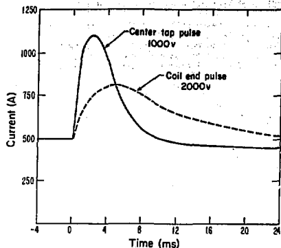
Fig. 7. Current in outer half coil during protection pulse.
