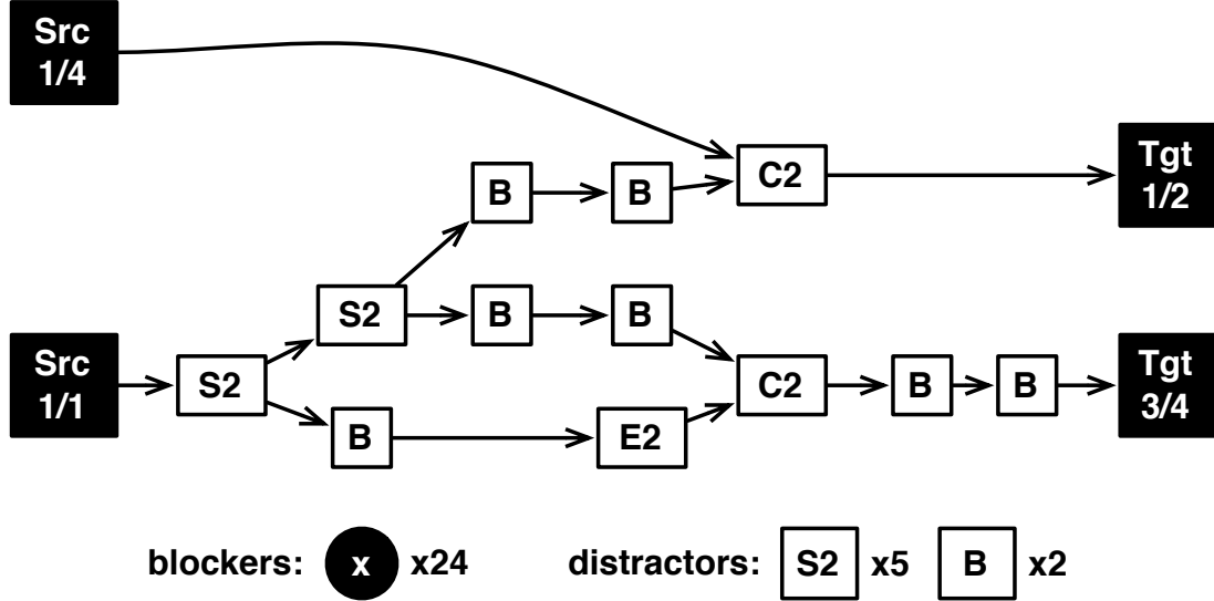
Figure 15.2: Mission DAG containing several 2-splitters (S2), benders (B), 2-combiners (C2), and a 2-expander (E2). Several blockers (x) and distracting pieces will also be present in any spatial realization of this mission.
