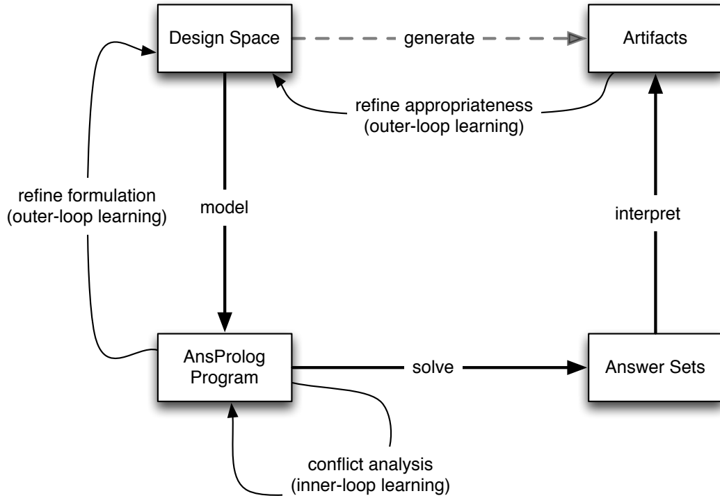
Figure 10.1: Modeling a design space as an AnsProlog program. The intent to generate artifacts from a designer’s hazily defined design space is carried out by modeling the design space (producing a tentative formal specification of appropriateness), applying an answer set solver to produce answer sets, and then interpreting the logical facts in those answer sets as descriptions of an artifact to be used in the desired domain. Observing artifacts other than those that the designer would think to construct manually provides new opportunities for learning in the outer loop of the designer’s double-loop learning. Likewise, spotting regularities in special cases encoded in the model can prompt a complete reformulation of how appropriateness is defined. This diagram is itself a refinement to the model–solve–interpret flow described in the practice documented by Brain et al. [17].
