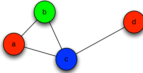
Figure 10.3: The first solution identified for coloring the graph from Figure 10.2 with three colors.
