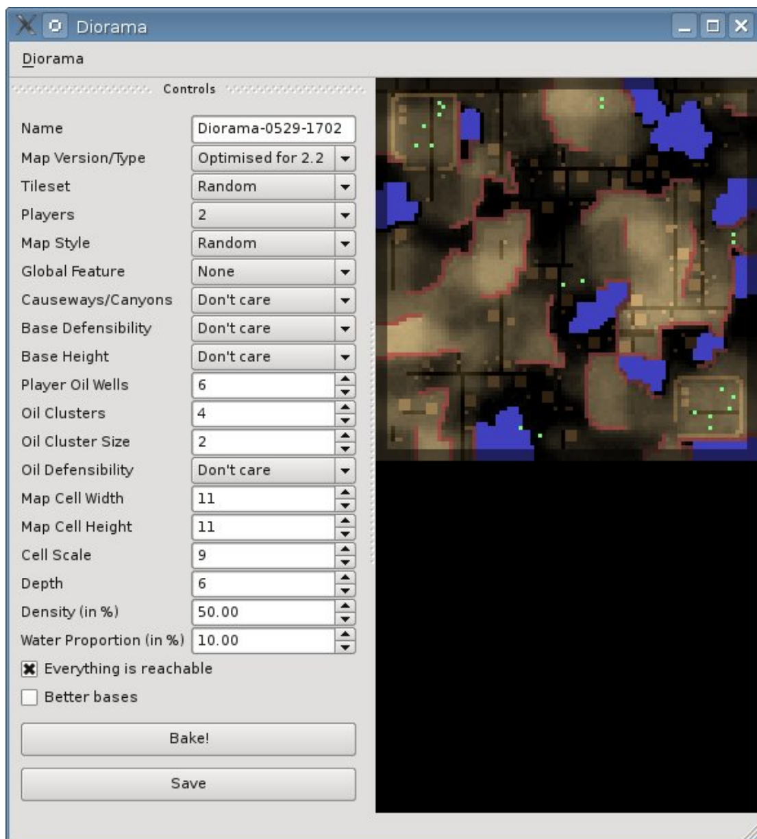
Figure 10.6: Screenshot of DIORAMA’s user interface. The “Bake!” button can be pressed to repeatedly sample alternate maps that satisfy the user’s specified design constraints.
