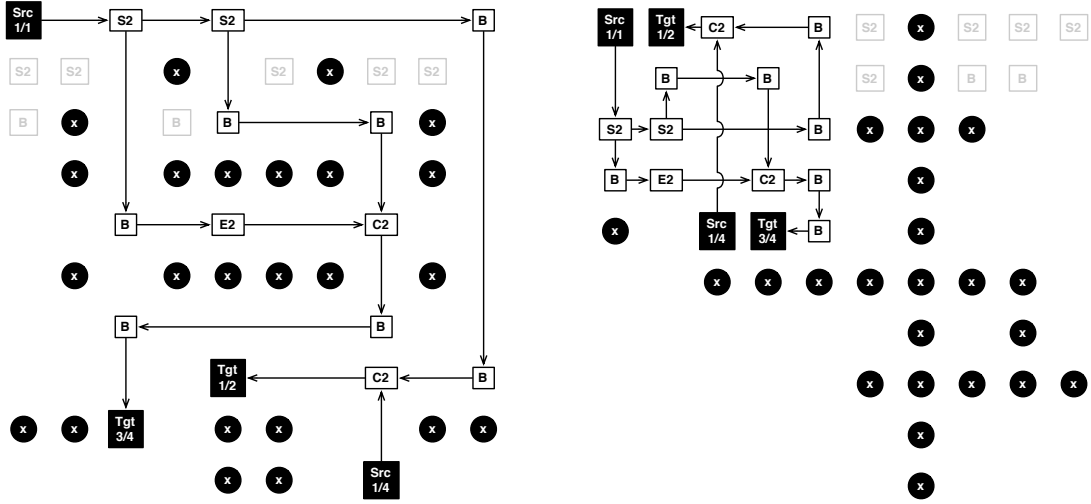
Figure 15.4: Two oppositely styled embeddings: the left exhibits compositional balance, blocker symmetry, beam spacing, and a lack of crossings while the right exhibits forced imbalance on both axes, asymmetry, piece abutting and multiple beam crossings.
