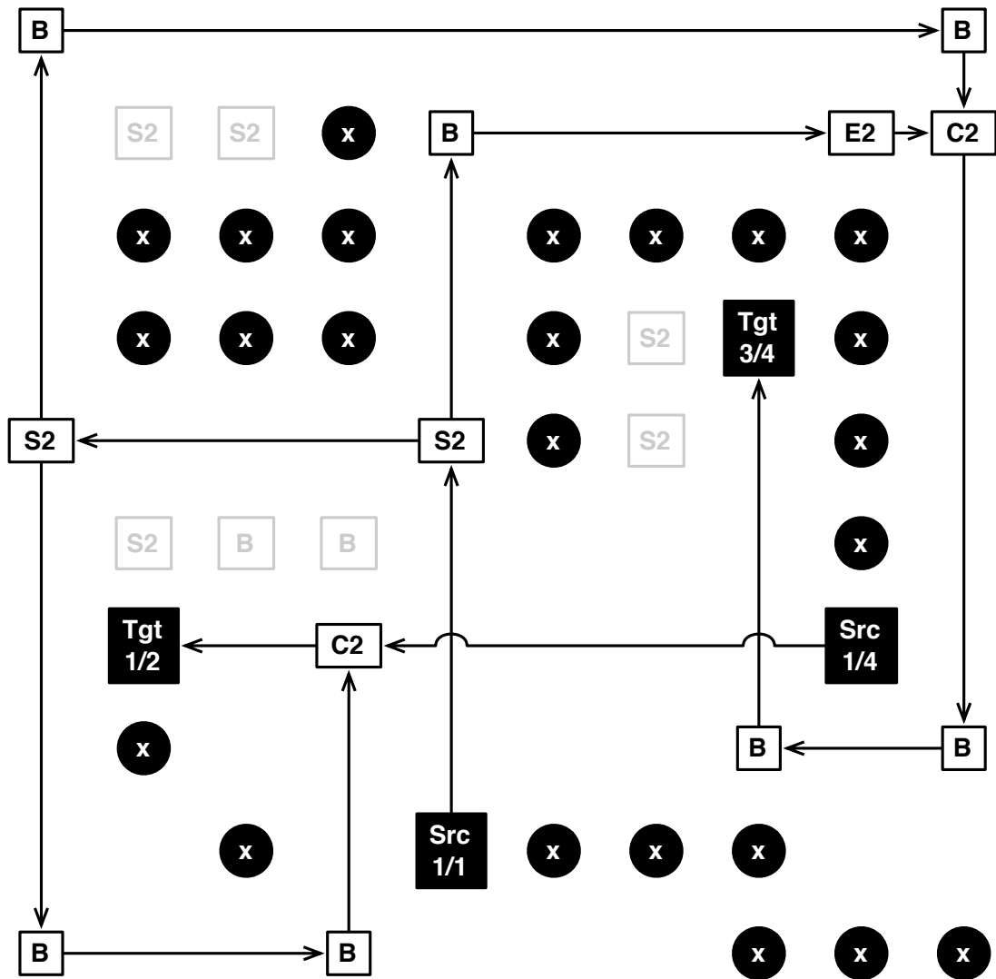
Figure 15.3: Embedding of the mission DAG from Figure 15.2 into Refraction 's 10-by-10 spatial grid under no special style constraints.
