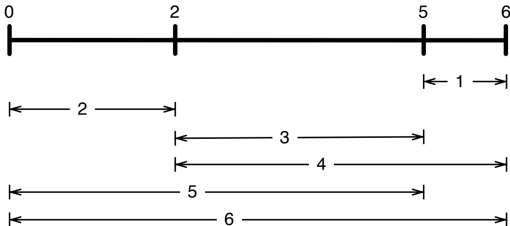
Figure 10.5: Example Golomb ruler of order 4 (the number of marks) and length 6 (the largest distance between marks). This is an optimal Golomb ruler because there are no shorter rulers of the same order.
