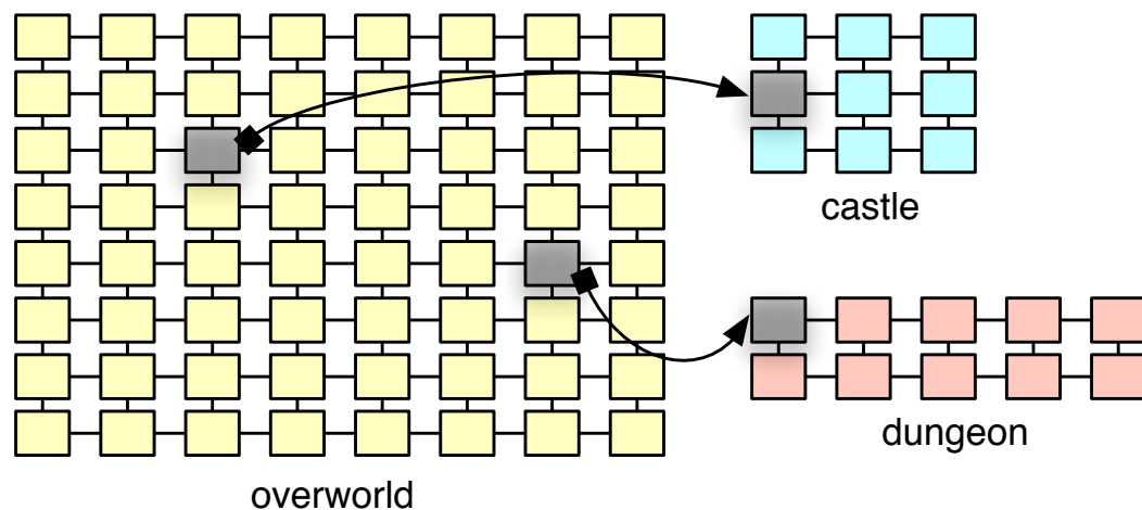
Figure 17.1: Map for a game sketch involving several interacting grid maps linked by directional portals. This is an example of simple content generation using deductive rules understandable by both BIPED’s machine and human playtesting sides.
