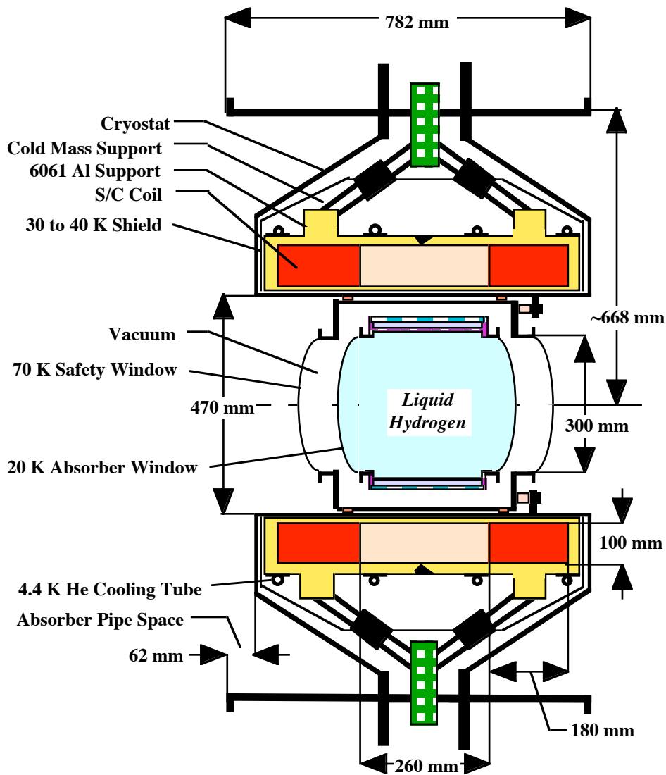
FIGURE 2. A cross-section of the MICE focusing module showing the S/C coils and a liquid absorber
