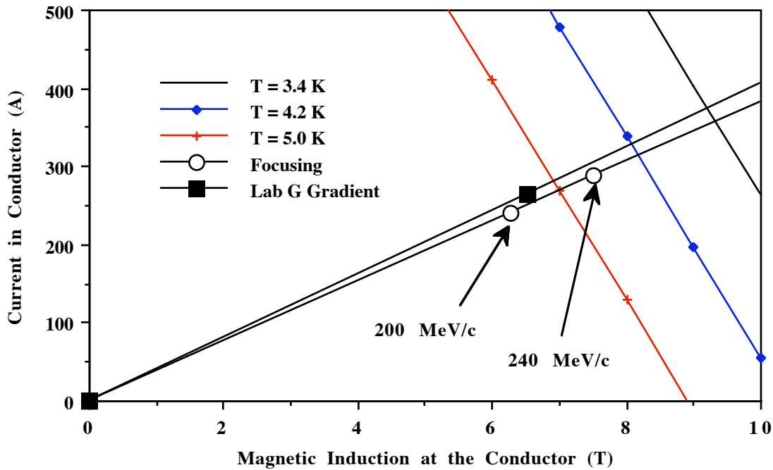
FIGURE 4. The Load Line for the Focusing Magnet and the Lab G Solenoid as Built (Both coils use the same conductor. The critical current versus induction for the conductor is shown at 3.4 K, 4.2 K, and 5.0 K.)
