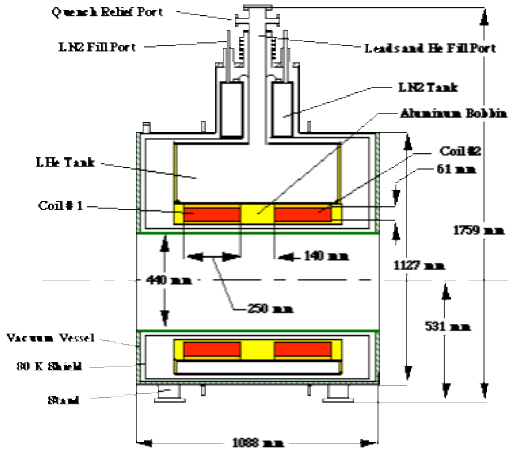
FIGURE 3. A cross-section of the gradient solenoid built for the 800 MHz RF experiment in Lab G
