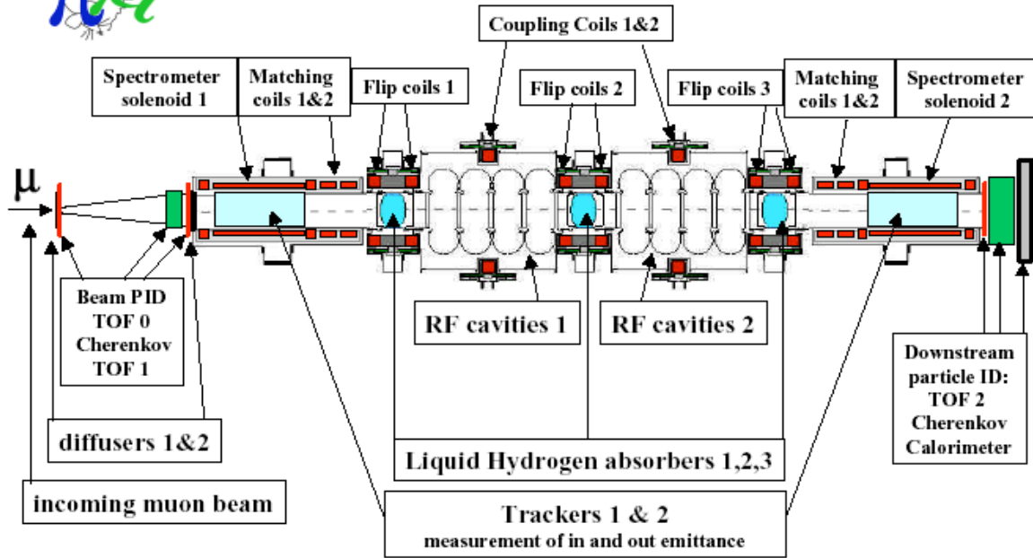
FIGURE 1. A general layout of the full MICE experiment showing all eighteen superconducting solenoid coils in seven magnet modules, the conventional RF cavities, the liquid hydrogen absorbers, the two central trackers which are in a uniform magnetic field and other types of particle detectors
