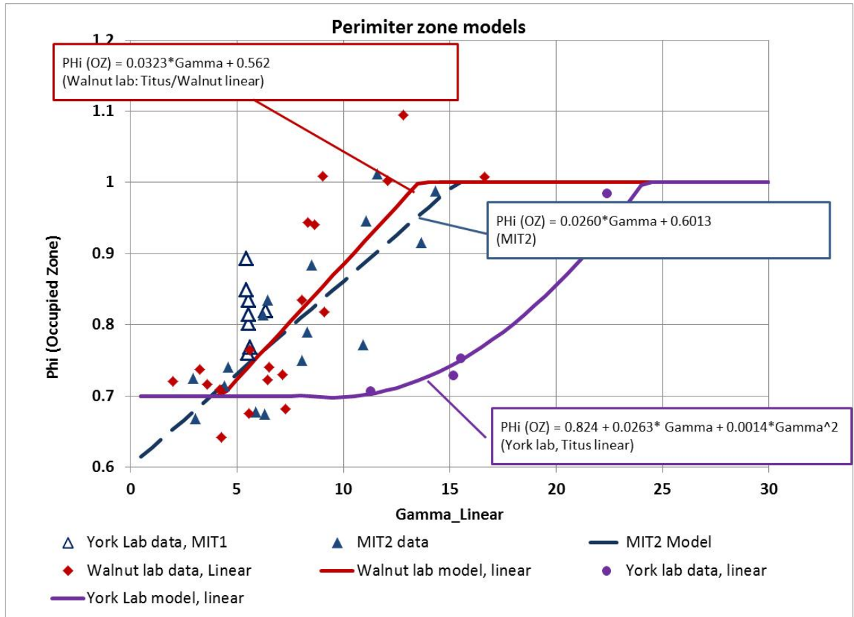
Figure 4. Perimeter zone stratification correlations ( NOTE: DO NOT USE York lab results )
