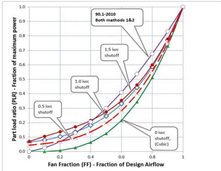
Figure 8. Fan part load curves for central airfoil fans with difference shutoff assumptions and for variable speed VAV terminal units.
