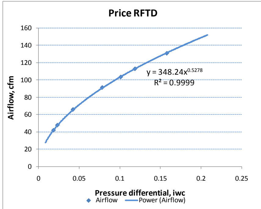
Figure 5c. Price swirl diffuser airflow performance
