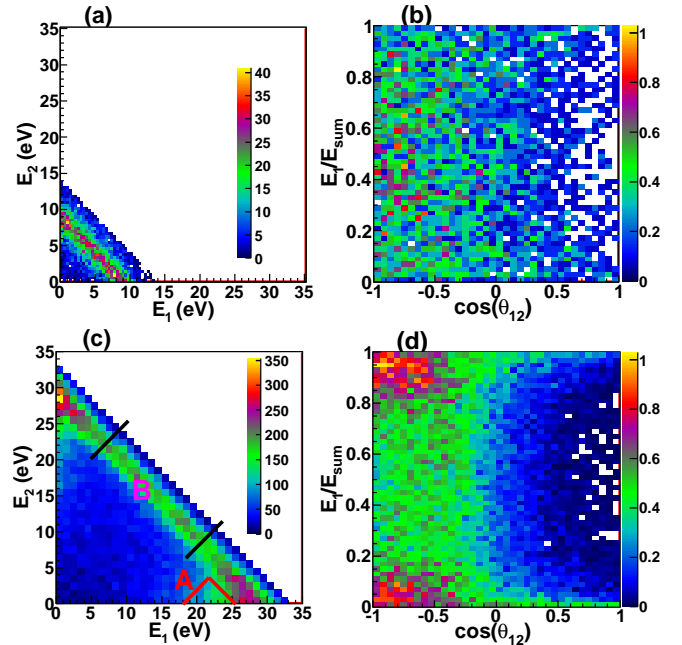
FIG. 5. (Color online) (a) Density plot of the kinetic energies of the two electrons measured in coincidence with the dications ( C_2H_2F_2^{2+} ). (b) Yield as a function of the cosine of the relative angle \theta_{12} between the two electrons' momenta and the energy sharing. Both (a) and (b) were measured using photon energy of 40 eV. (c-d) Same as (a-b), but for 60 eV photon energy. The regions A and B in panel (c) are used later on to identify the different ionization processes.
