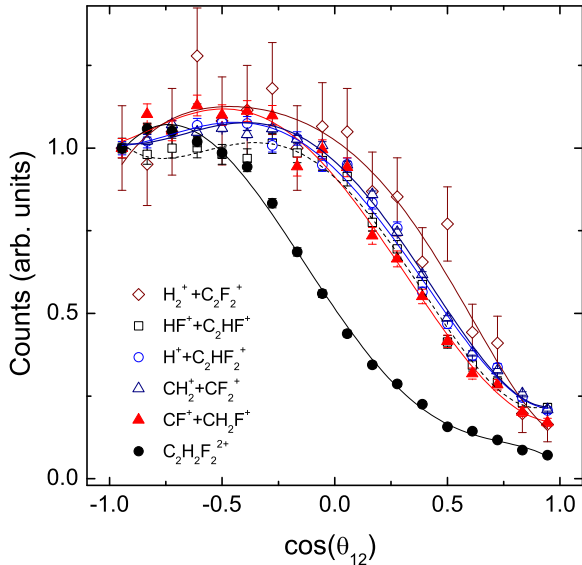
FIG. 4. (Color online) Yield as a function of cosine of the angle \theta_{12} between the momenta of the expelled electrons associated with different NDI and DI channels measured for the PDI of 1,1- C_2H_2F_2 at 60 eV photon energy. The lines (whose colors match the symbols' color of the corresponding channels) are just to guide the eye.
