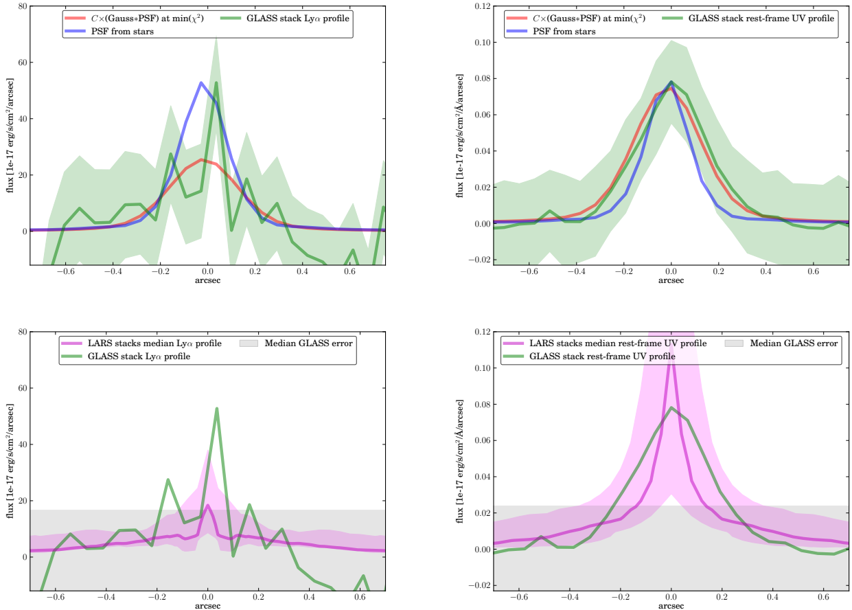
FIG. 10.— The spatial profiles of the stacked Gold_EL Ly \alpha emitters at \langle z \rangle = 7.2 (left, green curve) and their observed NIR (rest-frame UV) direct images (right, green curve). In the top panels these profiles are compared to the PSF represented by the spatial profile of stars (blue curves) in the GLASS filed-of-views. The red curves show the convolved PSF (multiplied by a constant C ) that minimizes the \chi^2 between the PSF and the data. Both the Ly \alpha and the rest-frame UV profiles from the GLASS stacks are unresolved. Hence, taken at the face value, there is no evidence that the spatial extent of Ly \alpha is more extend than the UV light in the GLASS stack. The bottom panels show a comparison to the median LARS Ly \alpha and rest-frame UV profiles at z = 7.2 cf. Section 10.1. The shaded area around the profiles shows the 1\sigma spread of the individual profiles. The median error on the GLASS stacks (from the top panel’s green shaded region) is represented by the gray band. Based on this comparison, we conclude that the extended Ly \alpha emission surface brightness typical of lower-redshift Lyman break galaxies is too faint to be detected in this GLASS stack.
