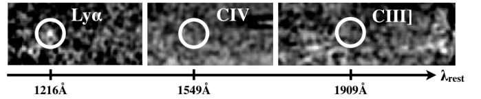
FIG. 9.— Cutouts of the stacked two-dimensional spectrum of the Gold_EL emission line objects listed in Table 3. The mean redshift of the shown stack is \langle z \rangle = 7.2 . The stacked Ly \alpha marked by the white circle on the left, appears compact and is not resolved (see top panel of Figure 10). There is no detection of a continuum break red-wards of the Ly \alpha line. The stacks show no detection of CIV \lambda 1549Å and CIII] \lambda 1909Å as indicated by the two right-most white circles.
