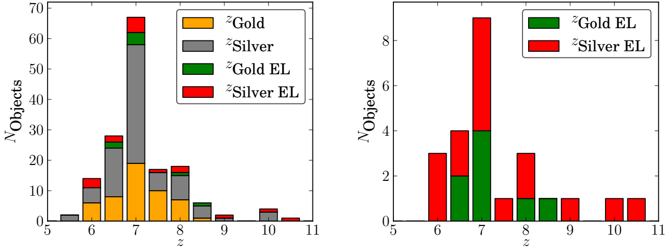
FIG. 3.— The redshift distribution of the Gold (orange), Silver (gray), Silver_EL (red) and Gold_EL (green) samples from Tables 2 and 3. In both panels, the distributions are stacked to show the total number of sources in each bin. For the Gold and Silver sample the redshift from the photometric selection(s) is used, whereas the redshifts for the EL samples correspond to the redshifts of the emission lines listed in Table 3, assuming that they are Ly \alpha .
