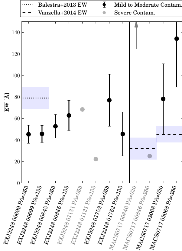
FIG. 11.— The equivalent widths estimated from the detections of Ly \alpha in the individual GLASS spectra of the four main images of the multiple imaged system at z = 6.1 from Boone et al. (2013) and Balestra et al. (2013) (left part) and the two images of the z = 6.4 Ly \alpha emitter from Vanzella et al. (2014b) (right part) listed in Table 5. The equivalent widths estimated by Balestra et al. (2013) and Vanzella et al. (2014b) are marked by the dotted and dashed lines, respectively. The shaded regions indicate the quoted uncertainties. The gray dots represent GLASS spectra with severe contamination at the location of Ly \alpha making the GLASS equivalent width estimates only tentative. The arrow indicates that the tentative estimate of MACS0717.00846 at PA=020 is outside the plotted range. The equivalent width estimates from the GLASS spectra generally agree with each other. There is marginal agreement with the Vanzella et al. (2014b) estimates, whereas the GLASS equivalent widths are generally lower than the estimate from Balestra et al. (2013).
