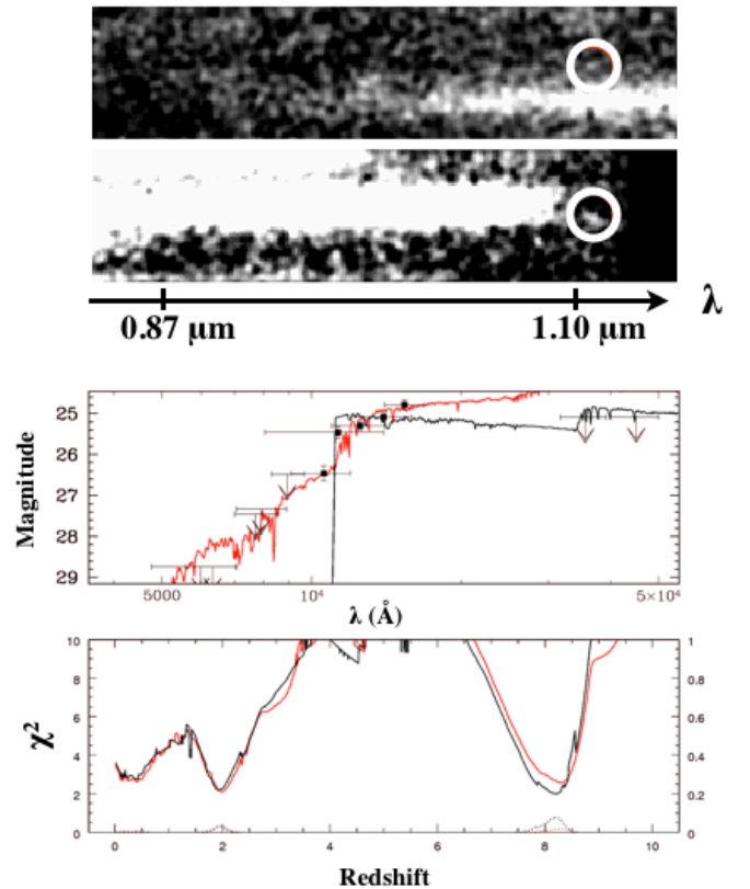
FIG. 7.— The GLASS G102 spectra (top panels), photometry (central panel) and photometric redshift estimate \chi^2 curve (bottom panel) for the candidate Ly \alpha emitter at z = 8.1 MACS2129_00899. The photometry includes CH1 and CH2 IRAC 1\sigma upper limits from SURFS-UP (Bradač et al. 2014) obtained following Huang et al. (2015). The black \chi^2 curve in the bottom panel includes F160W, whereas the red curve does not (F160W has potential contamination and therefore uncertain photometry). In both cases there are valid photometric redshifts around z \sim 8 (black spectral energy distribution over-plotted the photometry in center panel) and z \sim 2 (red spectral energy distribution over-plotted the photometry in center panel) with marginal statistical difference. The z \sim 2 solution over-estimates the 1\sigma IRAC constraints. If the line was [OII] \lambda 3727 at z = 1.97 we would expect to see [OIII] at roughly 14870Å. We do not detect any [OIII] emission in the GLASS G141 spectra, consistent with the z \sim 8 solution.
