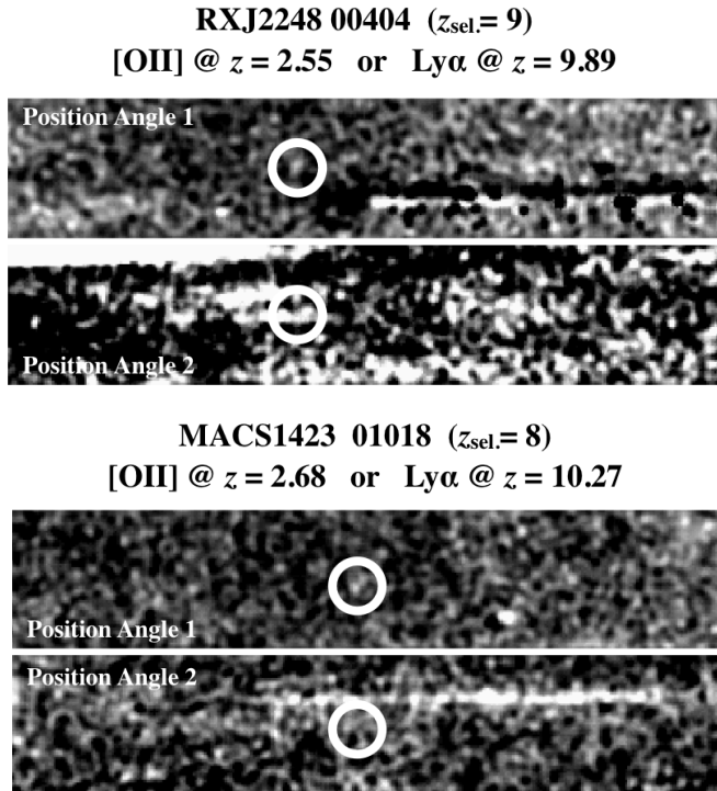
FIG. 8.— The GLASS G141 spectra of the two potential line emitters at z \sim 10 from the Silver_EL sample. The white circles mark the detected line emission. The objects were selected as Lyman break dropouts. However, highly likely low-redshift solutions in the EAZY p(z) suggest that the lines could also be [OII] at z \sim 2.6 . Given the location of the lines at 1.32\mu\text{m} and 1.37\mu\text{m} the G141 spectrum does not cover [OIII], and the resolution does not allow us to resolve the potential [OII] doublet or detect the asymmetry of Ly \alpha . With the current data we can therefore not rule out the high-redshift scenario.
