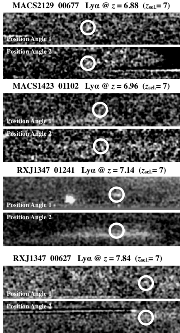
FIG. 2.— Examples of GLASS spectra for 4 out of the 24 z \gtrsim 7 emission line objects listed in Table 3. For each object the G102 spectrum at both of the GLASS PAs are shown. The assumed Ly \alpha redshift and the selection redshift from Table 3 are quoted above each panel. The circles mark the location of the emission lines. All spectra have been subtracted the contamination model from the GLASS reduction.
