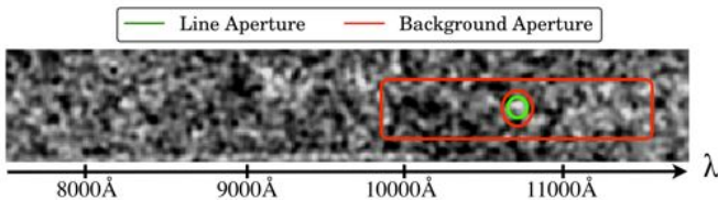
FIG. 4.— Example of the emission line and background apertures used when estimating the emission line fluxes (and 1\sigma flux sensitivities) of the GLASS spectra of RXC J1347.5-1145_00627 shown in Figure 2. The line flux is obtained by accumulating (‘integrating’) the flux in the green ellipsoidal line aperture ( E_{\text{line}} ). The red background aperture (excluding the red ellipse around the line aperture) is used to normalize the background level of the contamination-subtracted spectrum to account for over/under subtraction of the local background (and contamination).
