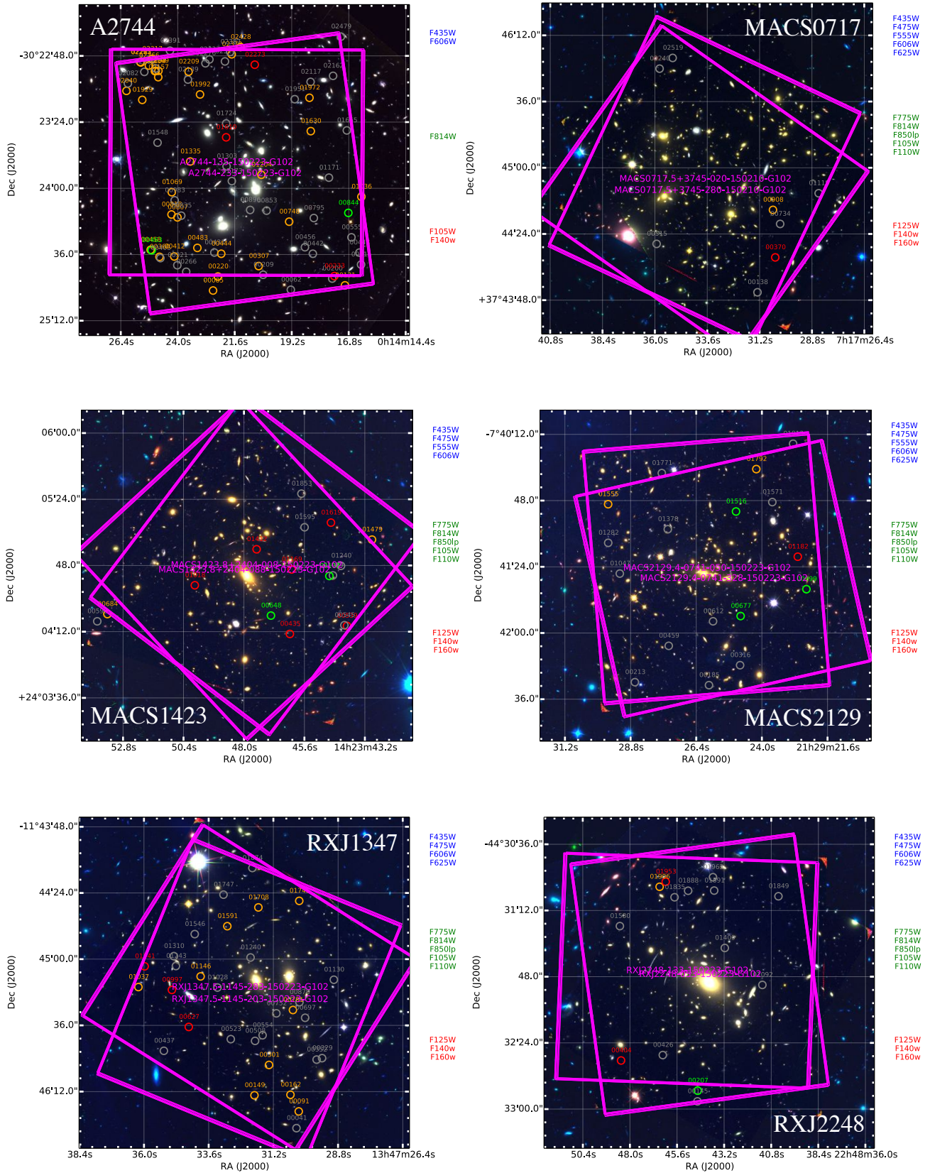
FIG. 1.— False-color composite images of the 6 GLASS clusters analyzed in this paper. From top left to bottom right we show Abell 2744, MACS J0717.5+3745, MACS J1423.8+2404, MACS J2129.4-0751, RXC J1347.5-1145, and RXC J2248.7-4431. Next to each panel the individual images used to generate the blue, green and red channels of the color composites are listed. The magenta polygons mark the field-of-view of the 20-degree separated GLASS pointings. The circles mark the location of the z \gtrsim 7 objects described in Section 3. The orange and gray circles mark the ‘Gold’ and ‘Silver’ objects from Table 2. The green and red circles show the location of the ‘Gold_EL’ and ‘Silver_EL’ objects presented in Table 3. The redshift distributions of these sources are shown in Figure 3. Note that objects immediately outside the GLASS field-of-view (MACS J1423.8+2404 in the center left panel) can still be recovered and extracted in the grism observations thanks to their detection in the ancillary CLASH imaging. The apparent over-density of high-redshift objects in Abell 2744 (top left) is caused by the increased depth (compared to the CLASH imaging) of the completed HFF data on Abell 2744. A similar improvement in sample size is expected for the remaining 5 HFF clusters in the GLASS sample.
