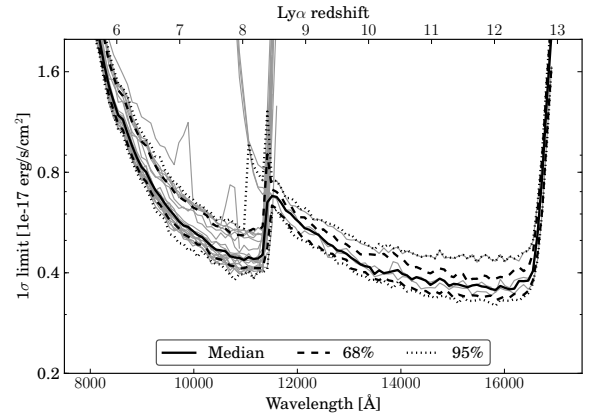
FIG. 5.— The 1\sigma sensitivity curves for the Gold sample in Table 2. The dashed and dotted lines show the 68% and 95% spread of the limits for the individual spectra, whereas the thick solid line shows the median 1\sigma sensitivity. The limits have not been corrected for the lensing magnification of each object, \mu , listed in Table 2. Including the lensing magnification will improve the line flux sensitivity by a factor \mu . The gray curves correspond to the line flux sensitivity of 25 (to avoid over-crowding the plot) individual spectra from a single PA. Combining the spectra from the two GLASS PAs for each object further decreases the noise level by a factor \sqrt{2} at all wavelengths.
