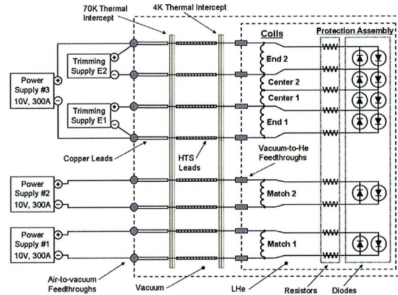
Figure 5: Magnet power supply and quench circuit.
