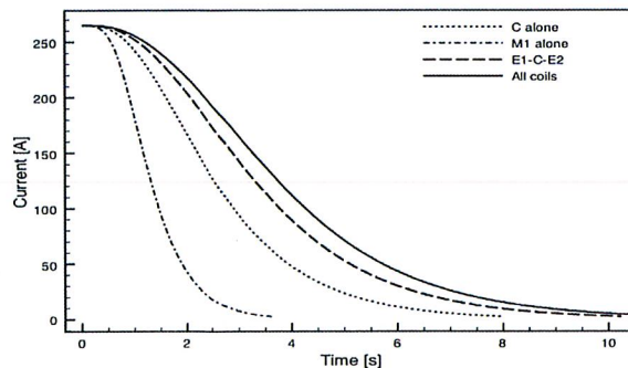
Figure 6: Current decay during a quench.
