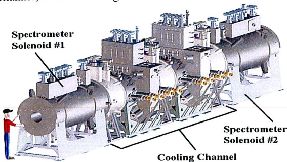
Figure 1: MICE cooling channel 3D CAD image.
