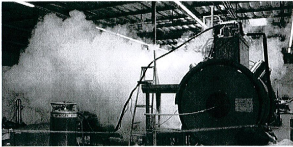
Figure 3: Quench during spectrometer solenoid training.
