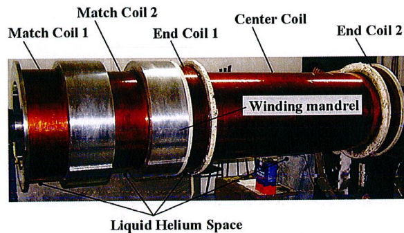
Figure 2: Spectrometer solenoid cold mass assembly.
