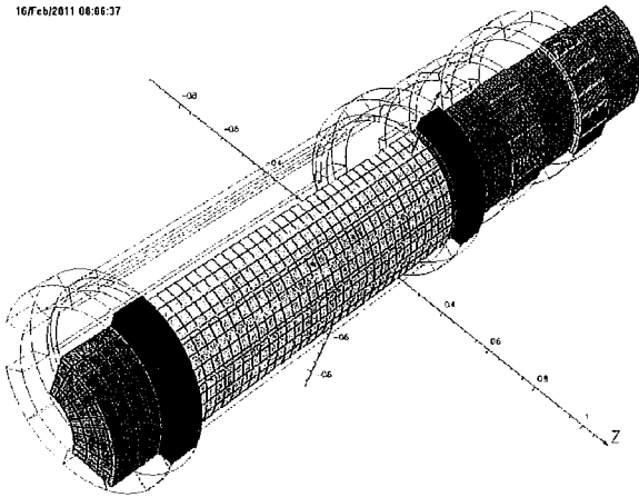
Figure 7: 3D quench analysis model.
