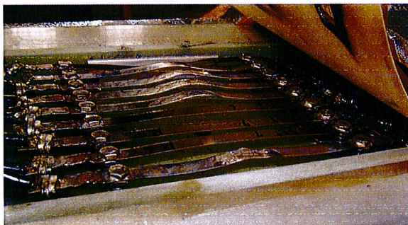
Figure 4: Heat damaged quench resistors.
