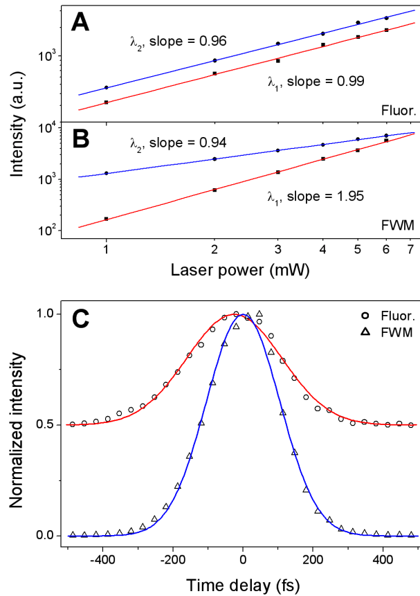
Fig. 3. Power dependence of the nonlinearly excited fluorescence (A) and FWM (B) signals. Both the signals and the laser powers of the fundamental beams ( \lambda_1, \lambda_2 ) are plotted on a logarithmic scale. (C) Fluorescence and FWM signals as a function of the time delay between the \lambda_1 and \lambda_2 beams. The red and blue curves show Gaussian fits to the nonlinear fluorescence and FWM cross correlations, respectively.
