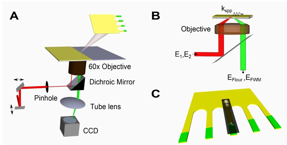
Fig. 1. (A) Schematic of the experimental setup. (B) Geometry of beam focusing and surface plasmon excitation with an objective lens. (C) Sketch of the patterned gold film (yellow) with extensions partially covered with CdSe quantum dots (green). The overlaid image represents actual data showing the FWM signals at the laser spot and the nonlinearly excited fluorescence from the quantum dots.
