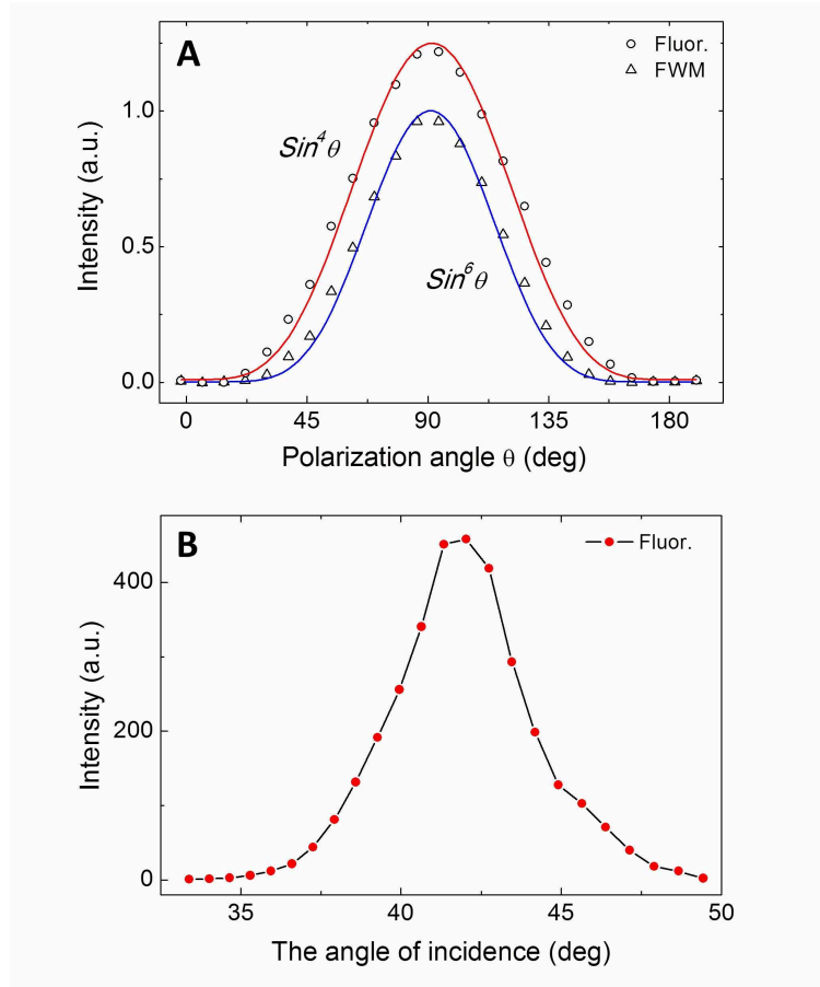
Fig. 4. (A) Nonlinearly excited fluorescence and FWM signals as a function of the polarization orientation of incident laser beams. S-polarized light corresponds to 0 degrees and p-polarized light coincides with 90 degrees in this graph. (B) Fluorescence intensity of the remotely excited quantum dots as a function of incident angle of the collinearly overlapped excitation beams.
