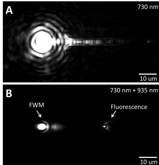
Fig. 2. (A) CCD image showing the laser spot and the leakage radiation of the propagating SPP mode excited by 730 nm p-polarized light. Note that the SPP mode propagates into the gold finger. (B) Image showing the FWM signal at the location of the laser spot, the leakage radiation from a SPP mode at 2\omega_1 = \omega_2 and the remotely-excited fluorescence from the quantum dots positioned on the gold finger. For this image, the bandpass filter in front of the CCD camera was chosen such that both the fluorescence emission and the FWM radiation was detected.
