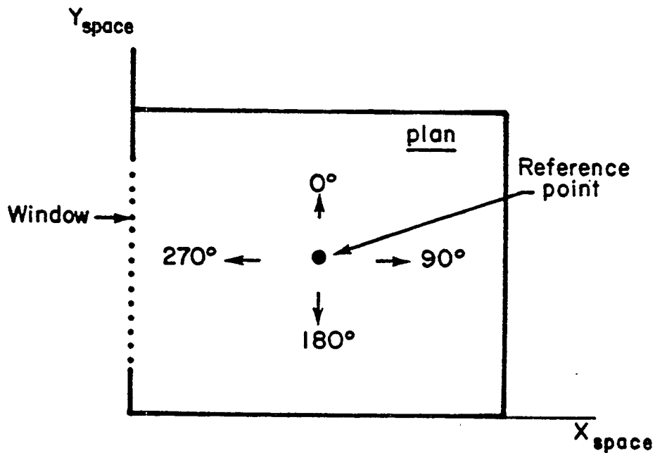
Figure 2.14: VIEW-AZIMUTH for four different occupant view directions. Daylight glare from the window will be greatest when occupant faces window, which corresponds to VIEW-AZIMUTH=270° in this example.
