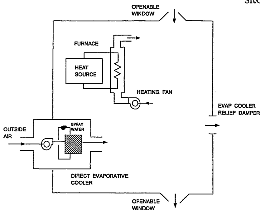
Figure 3.14: Residential System (RESYS) with Direct Evaporative Cooler.
