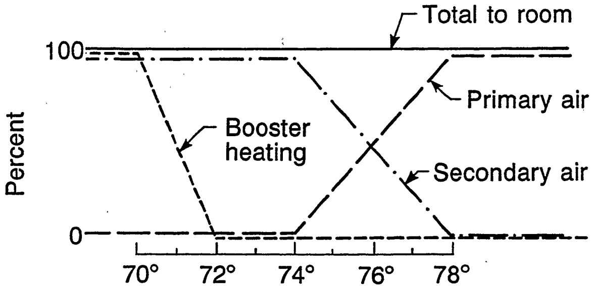
Figure 3.2: Series PIU
