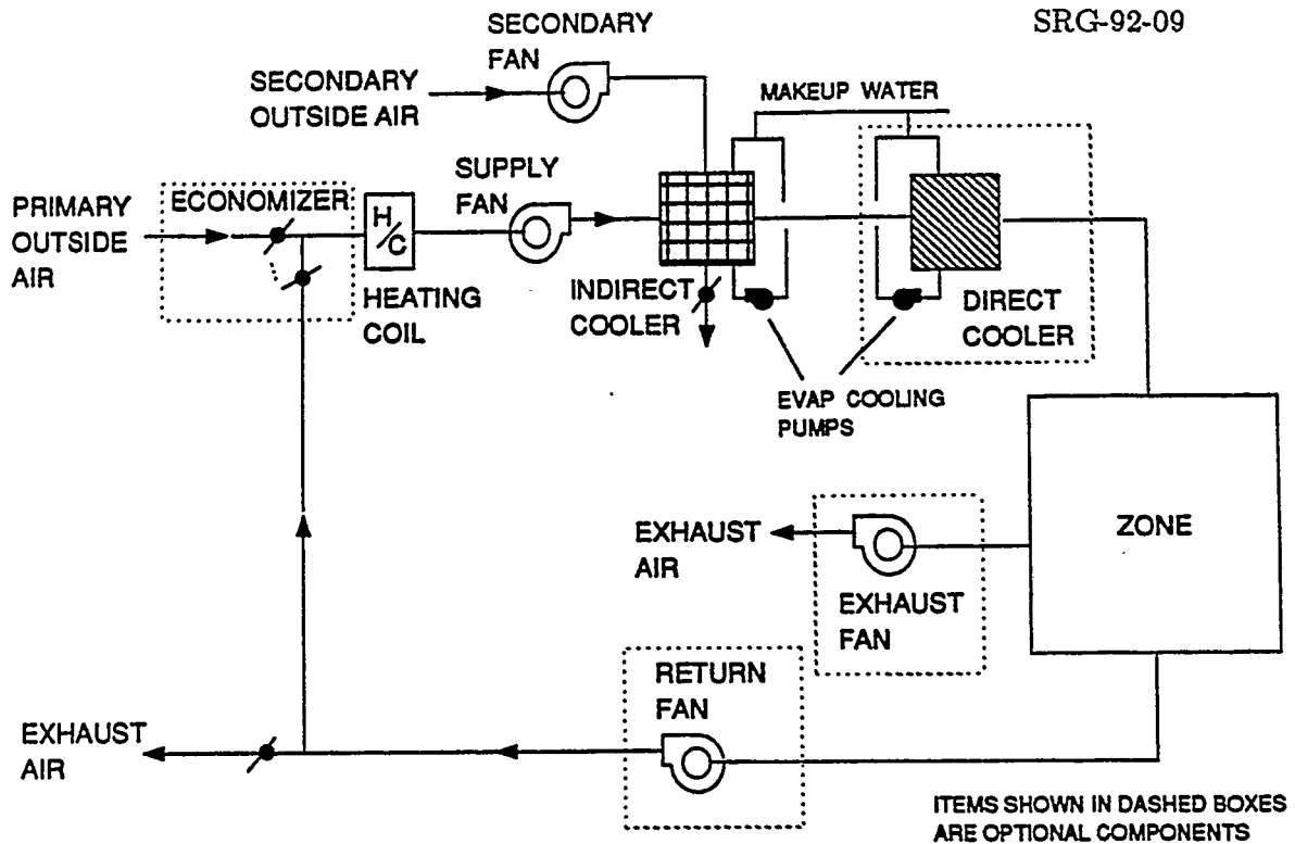
Figure 3.11: Stand-alone evaporative cooler system (SYSTEM-TYPE = EVAP-COOL).
