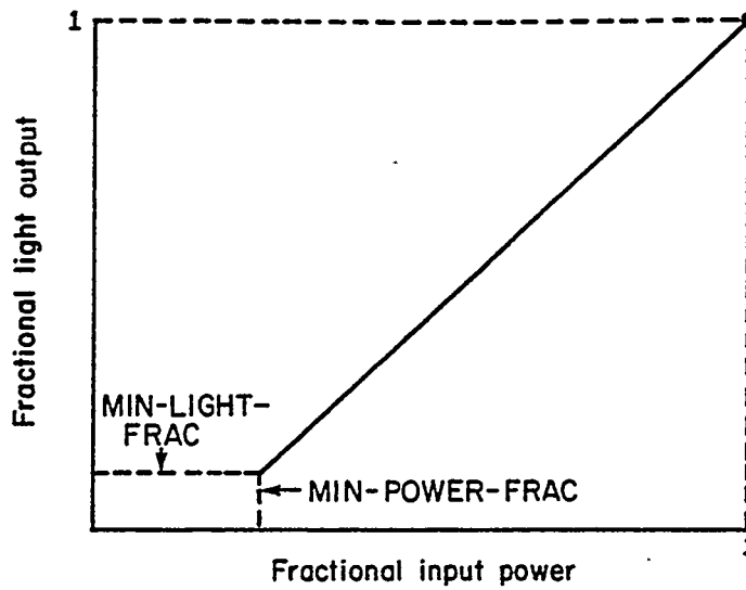
Figure 2.12: Relationship between light output and electrical input for a continuous dimming system.
