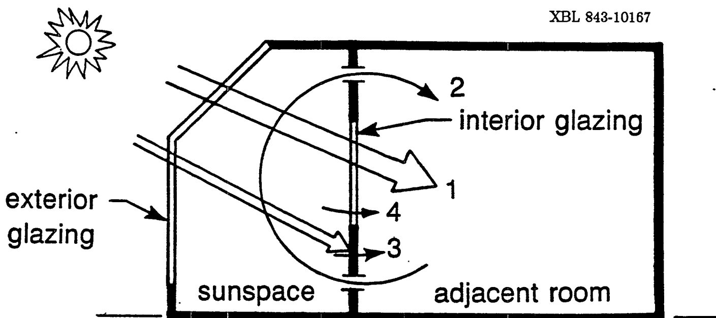
Figure 2.1: Forms of heat transfer calculated by the sunspace model: (1) direct and diffuse solar gain through interior glazing; (2) forced or natural convection through vents or an open doorway; (3) quick or delayed conduction through an interior wall, taking into account solar radiation absorbed on the sunspace side of the wall; and (4) conduction through interior glazing.
