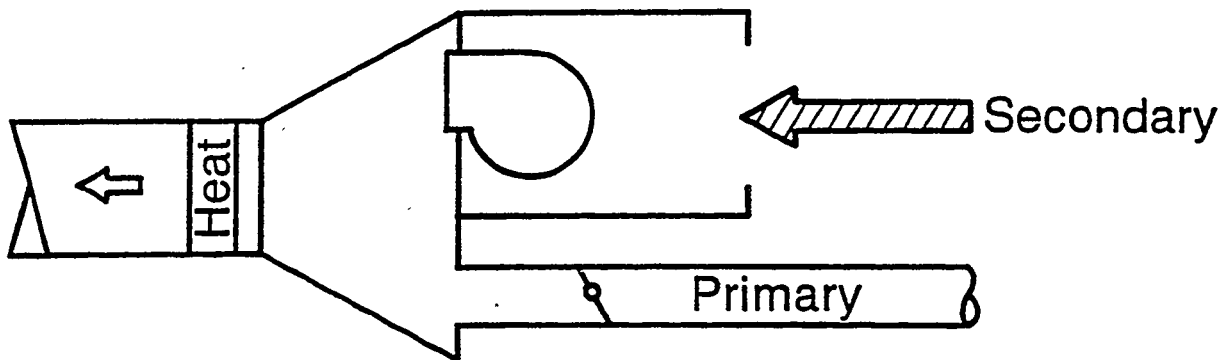
Figure 3.3: Parallel PIU
