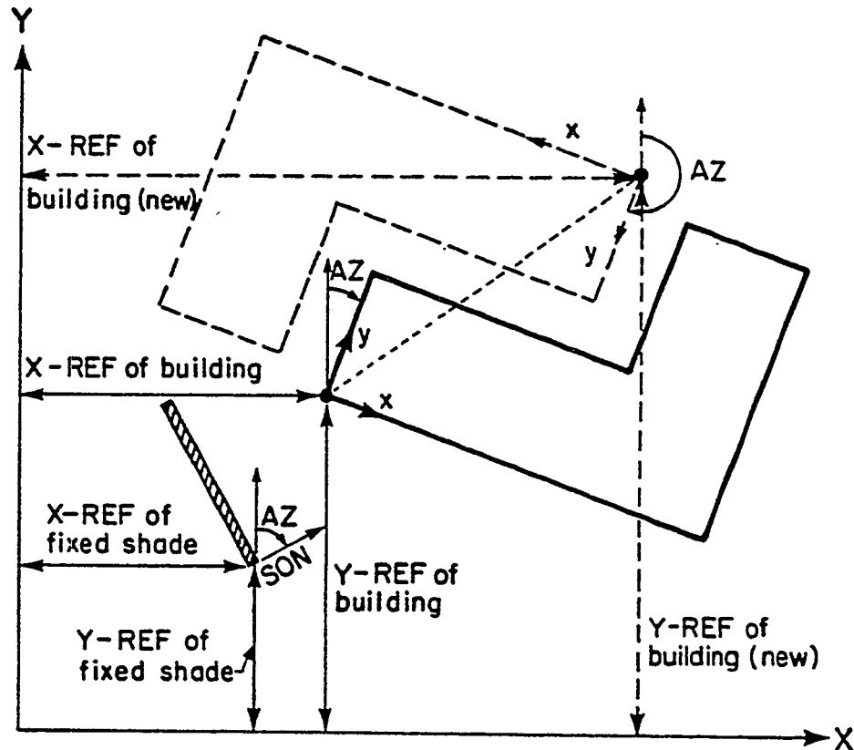
Figure 2.16 Reference coordinate system showing fixed shade and building. When the building is moved (dashed line), the fixed shade remains stationary.
