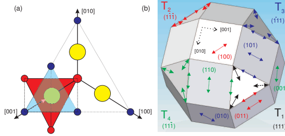
FIG. 1: (color online) (a) Atomic and spin structure in bulk NiO. Red and blue dots represent Ni atoms of opposite spin, while yellow dots represent O atoms. Antiferromagnetic order is caused by superexchange interaction along the Ni-O-Ni bond in the \langle 100 \rangle direction, so that the net moment on each O site vanishes. Ni spins within a particular \{111\} sheet are aligned parallel (red and blue planes). (b) Possible orientations of the T(win) domains, labeled T_1 to T_4 , and walls in NiO. The possible spin axes in each T -domain are shown by double headed arrows with the same color. Also shown are the spin axes and domain wall orientations for domains walls between T_1 shown in black and the three other T -domains.
