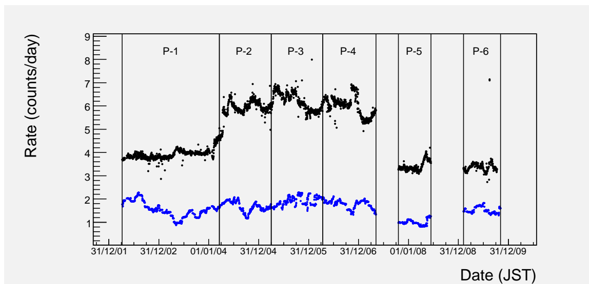
Figure 6.10: Accidental background rate and expected reactor signal rate — for an unoscillated reactor-flux — as a function of time. For the accidentals study the data is divided into 6 periods: P1, \dots , P6; the vertical lines mark the boundaries of these periods.
