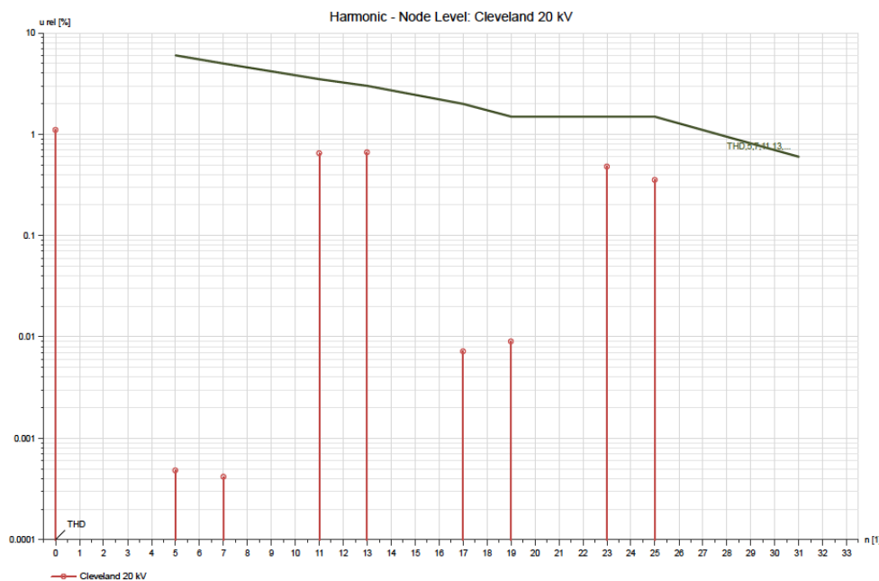
Figure 5. PSS/Sincal Harmonics Results Graph
