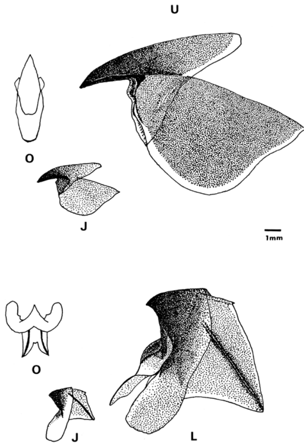
FIGURE 41. Histiotteuthis heteropsis ; mantle length of specimens: adult 82.0 mm, juvenile 21.0 mm. Adult beaks colored entirely. Upper beak: jaw angle approximately 90 degrees; distinct false angle present; shoulder irregular; crest and hood diverge at 30 degree angle. Lower beak: jaw angle obtuse; distinct narrow ridge on lateral wall extending to posterior corner; crest length shorter than hood length.
