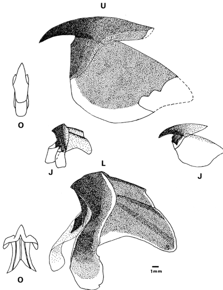
FIGURE 37. Onychoteuthis boreali-japonicus ; total length of specimens: adult 515.0 mm, juvenile 80.0 mm. Adult beaks colored entirely except for margin of lateral walls; juvenile colored less, more transparent. Upper beak: jaw angle acute with slight false angle in larger specimens; prominent striated dark segment on wing at jaw angle of juvenile. Lower beak: jaw angle obtuse; narrow ridge on lateral wall becoming broader posteriorly; hood short.
