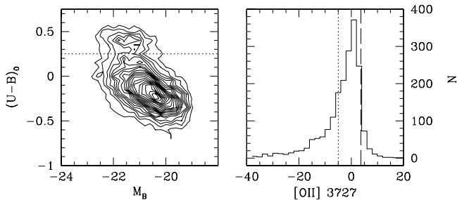
FIG. 1.— Left panel: Restframe color-magnitude diagram of 17,745 DEEP2 galaxies. Our sample of RSGs is defined by U-B > 0.25 (objects above the dotted line). Right panel: A histogram of [OII] \lambda 3727 EWs for RSGs. Because the [OII] line is overimposed to strong absorption lines, EW=0 is not achieved for zero emission. Instead, no [OII] emission happens when EW[OII]=3.7 \text{ \AA} (dashed line, Konidaris et al. in preparation), with emission line galaxies having lower EWs. All galaxies with EW[OII] \leq -5 \text{ \AA} (dotted line) are excluded from the sample.
