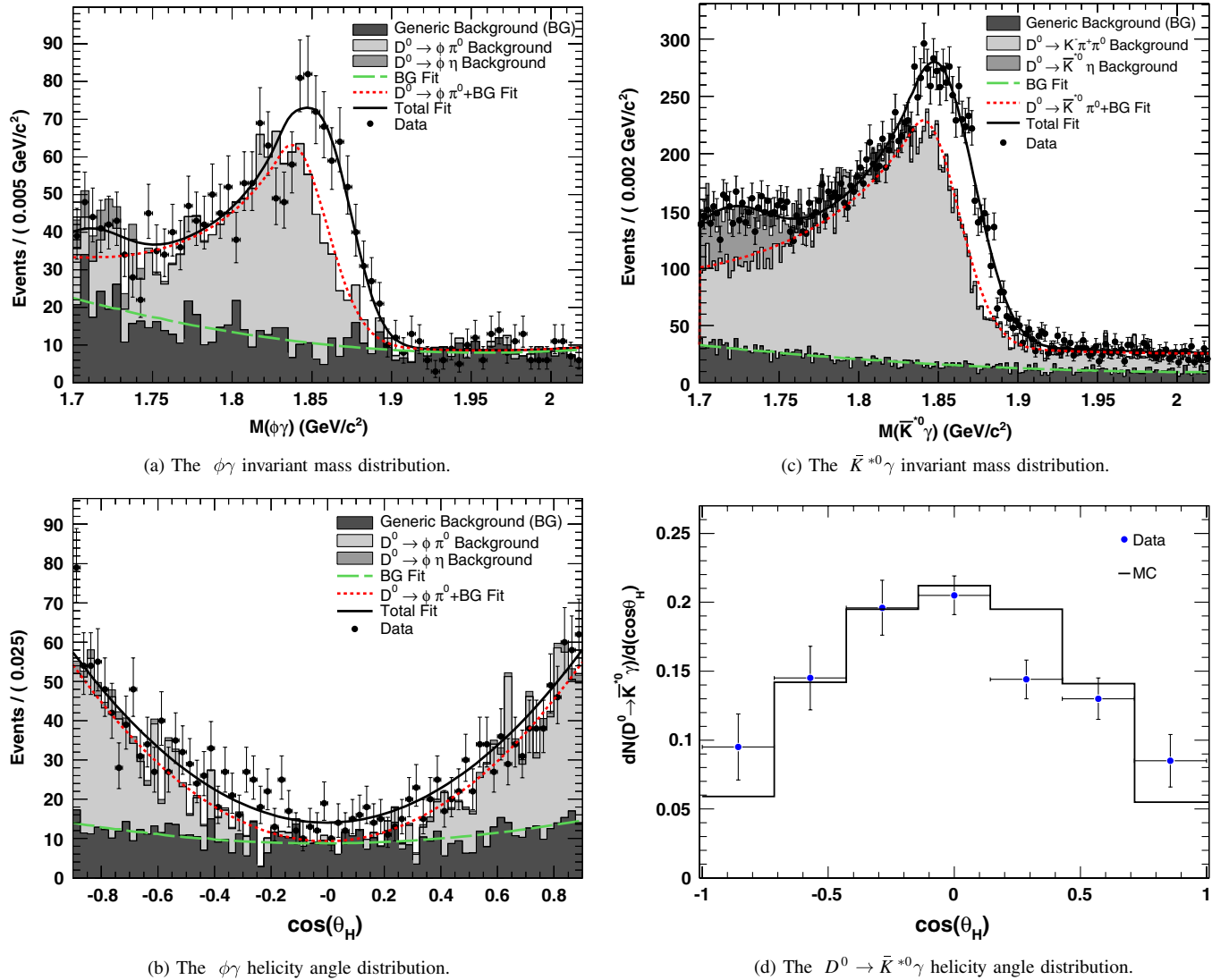
FIG. 2 (color online). Invariant mass and \cos\theta_H distributions for data (points) and simulated events (histograms). The curves show the fit results and the background contributions. BG refers to the combinatoric background.
