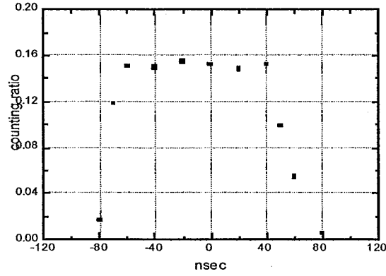
Fig. 11: A timing plateau of the ionization chamber in coincidence with the 5mm x 5mm and 50mm x 50mm scintillation counters.
