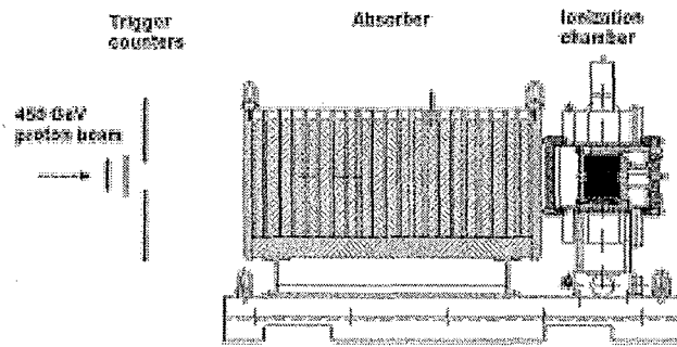
Fig. 3: Schematic of trigger counters, absorber and ionization chamber.
