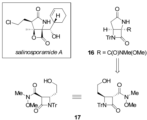
Figure 1. Diazabicyclo[3.2.0] retrosynthesis
