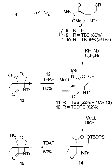
Scheme 3. Bicyclo[3.2.0] framework
