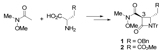
Scheme 1. Previous Work
