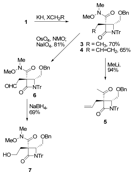
Scheme 2. \alpha -Alkylation
